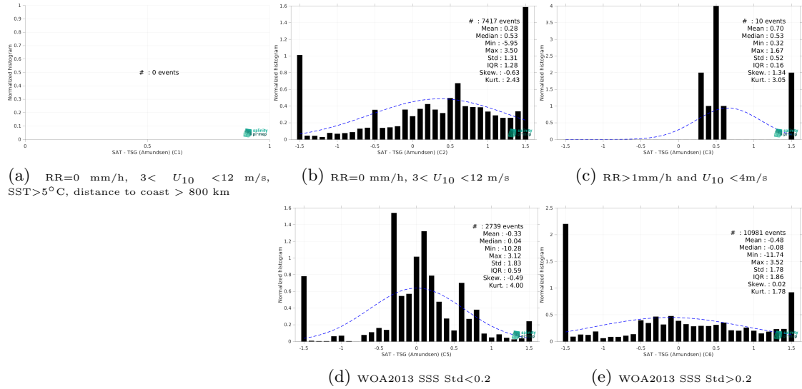
Figure 15: Normalized histogram of \Delta SSS (Aquarius SSS L2 OR v5 (NASA-GSFC) - TSG (Amundsen)) for 5 different subdatasets corresponding to: RR=0 mm/h, 3 < U_{10} < 12 m/s, SST > 5°C, distance to coast > 800 km (a), RR=0 mm/h, 3 < U_{10} < 12 m/s (b), RR > 1mm/h and U_{10} < 4 m/s (c), WOA2013 SSS Std < 0.2 (d), WOA2013 SSS Std > 0.2 (e).
