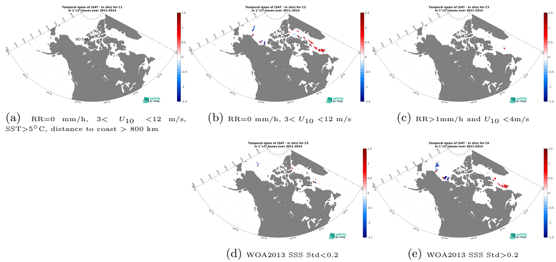
Figure 14: Temporal mean gridded over spatial boxes of size 1^\circ \times 1^\circ of \Delta SSS (Aquarius SSS L2 OR v5 (NASA-GSFC) - TSG (Amundsen)) for 5 different subdatasets corresponding to: RR=0 mm/h, 3 < U_{10} < 12 m/s, SST > 5°C, distance to coast > 800 km (a), RR=0 mm/h, 3 < U_{10} < 12 m/s (b), RR > 1mm/h and U_{10} < 4 m/s (c), WOA2013 SSS Std < 0.2 (d), WOA2013 SSS Std > 0.2 (e).
