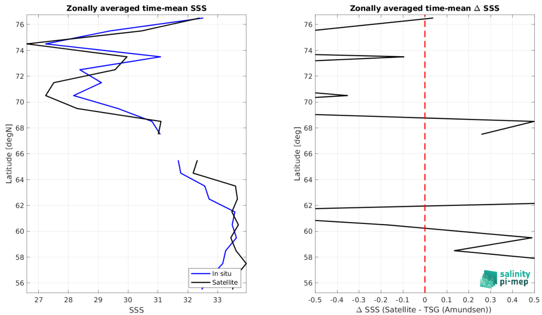
Figure 9: Left panel: Zonal mean SSS from Aquarius SSS L2 OR v5 (NASA-GSFC) satellite product (black) and from TSG (Amundsen) (blue). Right panel: Zonal mean of \Delta SSS (Satellite - TSG (Amundsen)) for all the collected Pi-MEP match-up pairs estimated over the full satellite product period.
