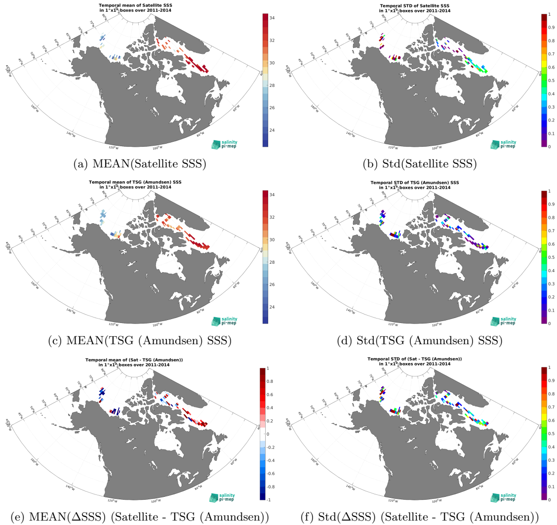
Figure 7: Temporal mean (left) and Std (right) of SSS from Aquarius SSS L2 OR v5 (NASA-GSFC) (top), TSG (Amundsen) (middle), and of \Delta SSS (Satellite - TSG (Amundsen)). Only match-up pairs are used to generate these maps.
