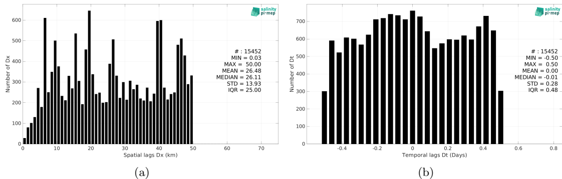
Figure 6: Histograms of the spatial (a) and temporal (b) lags between the location/time of the TSG (Amundsen) measurement and the date of the corresponding Aquarius SSS L2 OR v5 (NASA-GSFC) SSS pixel.
