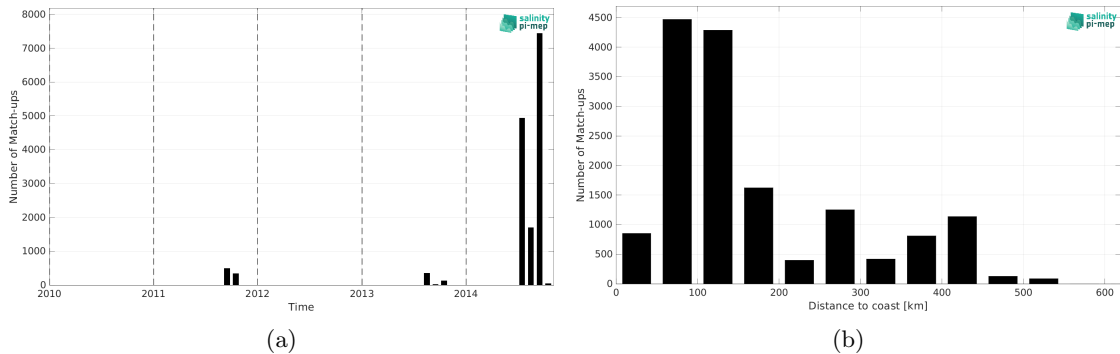
Figure 2: Number of match-ups between TSG (Amundsen) and Aquarius SSS L2 OR v5 (NASA-GSFC) SSS as a function of time (a) and as function of the distance to coast (b) over the Global Ocean Pi-MEP region and for the full satellite product period.
