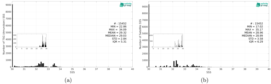
Figure 3: Histograms of SSS from TSG (Amundsen) (a) and Aquarius SSS L2 OR v5 (NASA-GSFC) (b) considering all match-up pairs per bins of 0.1 over the Global Ocean Pi-MEP region and for the full satellite product period.
