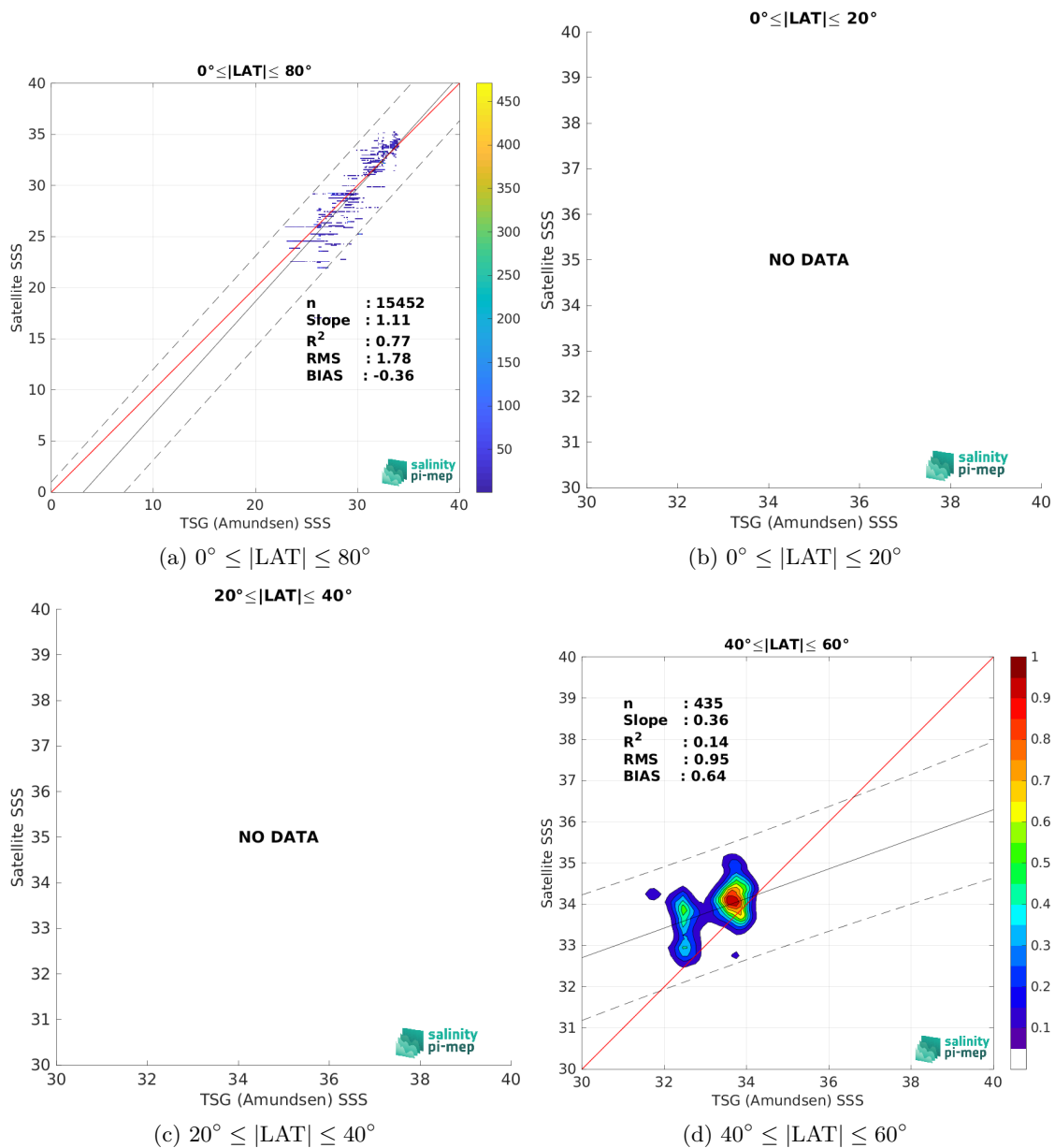
Figure 10: Contour maps of the concentration of Aquarius SSS L2 OR v5 (NASA-GSFC) SSS (y-axis) versus TSG (Amundsen) SSS (x-axis) at match-up pairs for different latitude bands. For each plot, the red line shows x=y . The black thin and dashed lines indicate a linear fit through the data cloud and the \pm 95\% confidence levels, respectively. The number match-up pairs n , the slope and R^2 coefficient of the linear fit, the root mean square (RMS) and the mean bias between satellite and in situ data are indicated for each latitude band in each plots.
