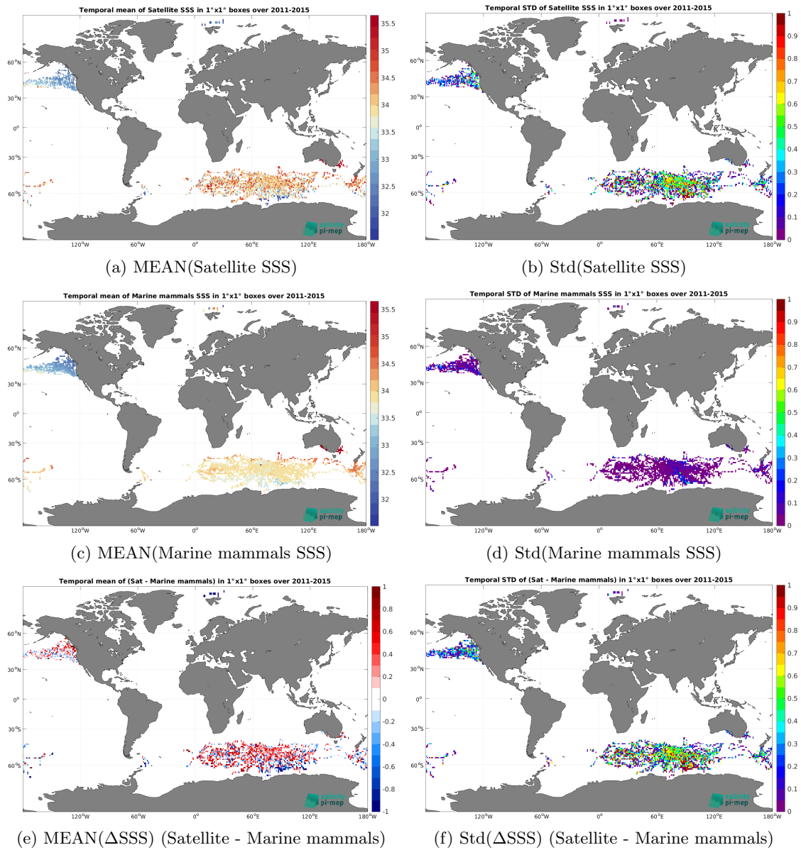
Figure 7: Temporal mean (left) and Std (right) of SSS from Aquarius SSS L2 OR v5 (NASA-GSFC) (top), Marine mammals (middle), and of \Delta SSS (Satellite - Marine mammals). Only match-up pairs are used to generate these maps.
