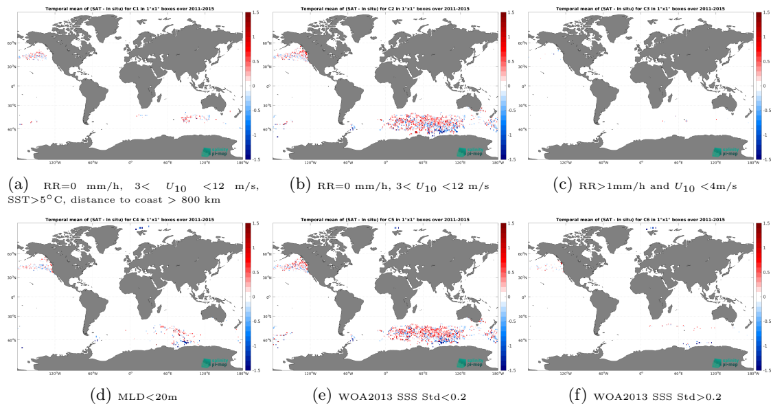
Figure 14: Temporal mean gridded over spatial boxes of size 1^\circ \times 1^\circ of \Delta SSS (Aquarius SSS L2 OR v5 (NASA-GSFC) - Marine mammals) for 6 different subdatasets corresponding to:RR=0 mm/h, 3 < U_{10} < 12 m/s, SST>5°C, distance to coast > 800 km (a), RR=0 mm/h, 3 < U_{10} < 12 m/s (b), RR>1mm/h and U_{10} < 4 m/s (c),MLD<20m (d),WOA2013 SSS Std<0.2 (e),WOA2013 SSS Std>0.2 (f).
