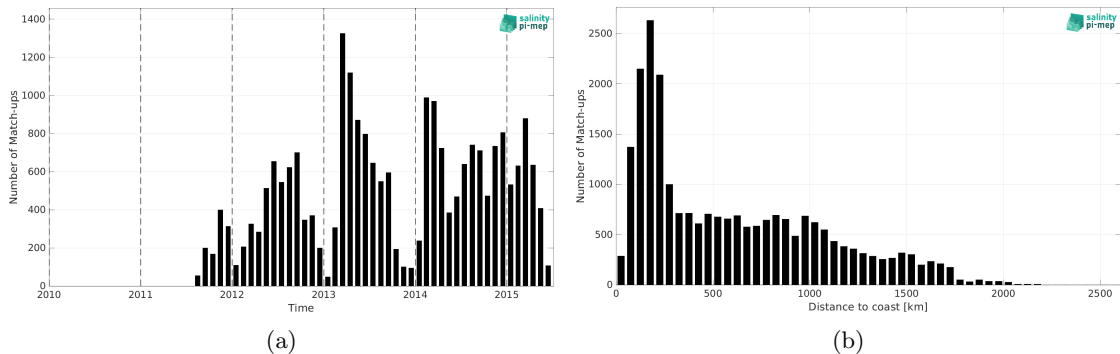
Figure 2: Number of match-ups between Marine mammals and Aquarius SSS L2 OR v5 (NASA-GSFC) SSS as a function of time (a) and as function of the distance to coast (b) over the Global Ocean Pi-MEP region and for the full satellite product period.
