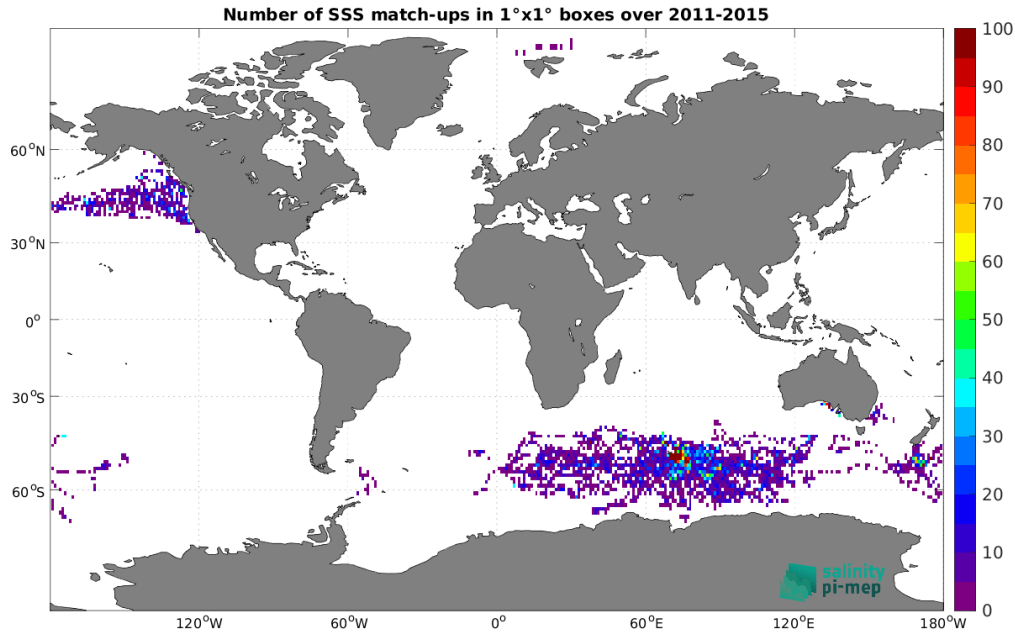
Figure 5: Number of SSS match-ups between Marine mammals SSS and the Aquarius SSS L2 OR v5 (NASA-GSFC) SSS product for the Global Ocean Pi-MEP region over 1^\circ \times 1^\circ boxes and for the full satellite product period.
