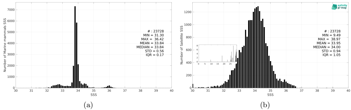
Figure 3: Histograms of SSS from Marine mammals (a) and Aquarius SSS L2 OR v5 (NASA-GSFC) (b) considering all match-up pairs per bins of 0.1 over the Global Ocean Pi-MEP region and for the full satellite product period.
