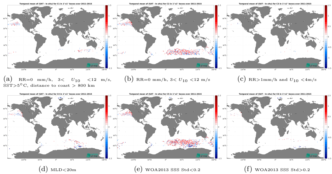
Figure 12: Temporal mean gridded over spatial boxes of size 1^\circ \times 1^\circ of \Delta SSS (Aquarius SSS L2 OR v5 (NASA-GSFC) - Marine mammals) for 6 different subdatasets corresponding to:RR=0 mm/h, 3 < U_{10} < 12 m/s, SST >5^\circ C, distance to coast > 800 km (a), RR=0 mm/h, 3 < U_{10} < 12 m/s (b), RR >1 mm/h and U_{10} < 4 m/s (c),MLD <20 m (d),WOA2013 SSS Std <0.2 (e),WOA2013 SSS Std >0.2 (f).
