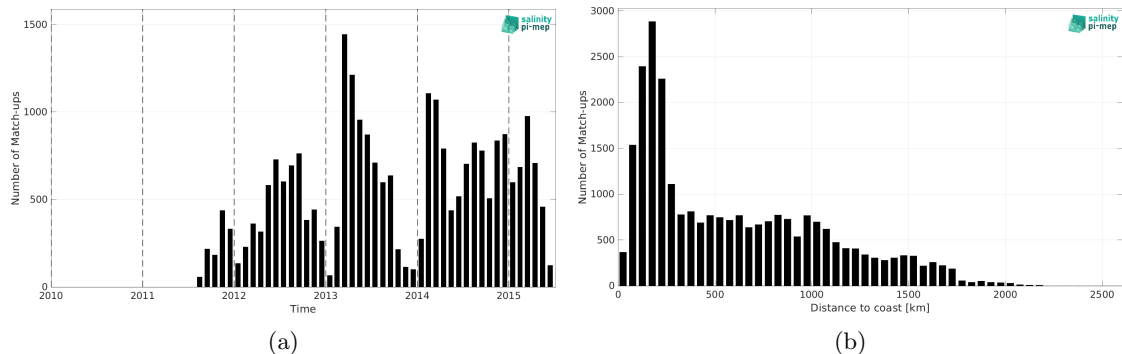
Figure 1: Number of match-ups between Marine mammals and Aquarius SSS L2 OR v5 (NASA-GSFC) SSS as a function of time (a) and as function of the distance to coast (b) over the Global Ocean Pi-MEP region and for the full satellite product period.
