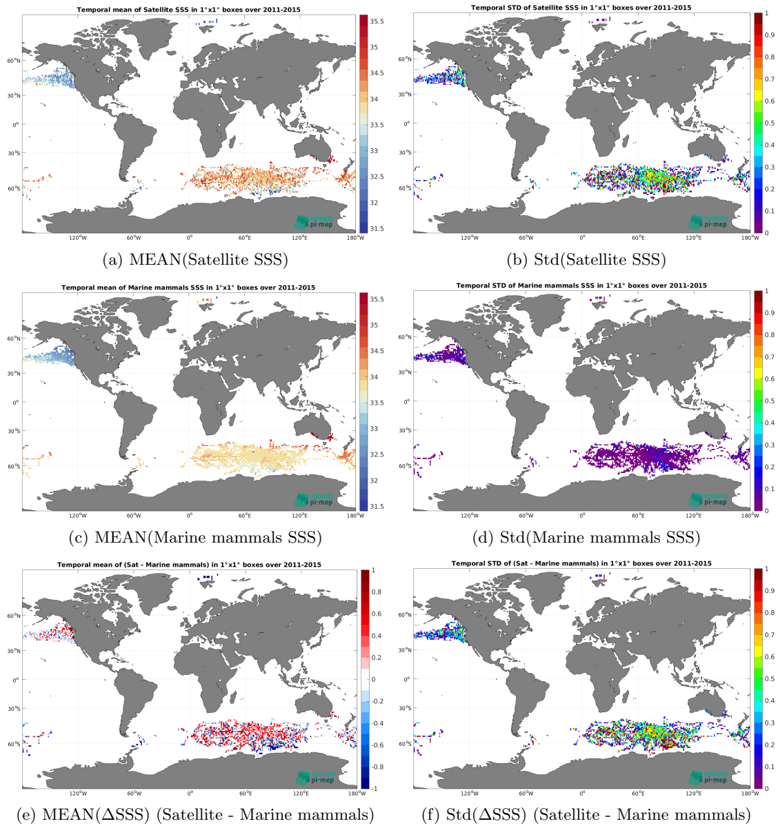
Figure 6: Temporal mean (left) and Std (right) of SSS from Aquarius SSS L2 OR v5 (NASA-GSFC) (top), Marine mammals (middle), and of \Delta SSS (Satellite - Marine mammals). Only match-up pairs are used to generate these maps.
