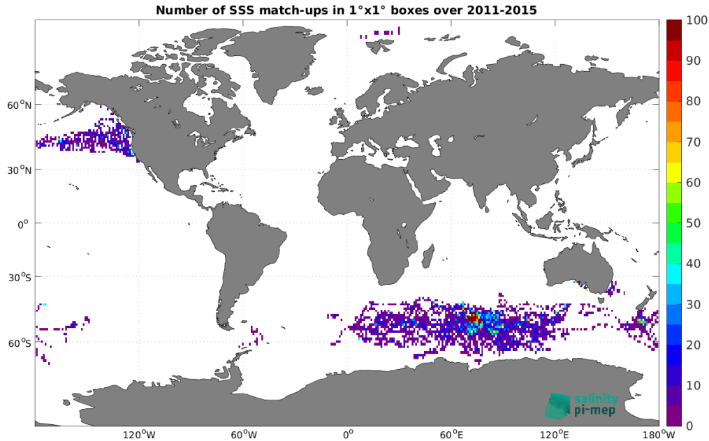
Figure 4: Number of SSS match-ups between Marine mammals SSS and the Aquarius SSS L2 OR v5 (NASA-GSFC) SSS product for the Global Ocean Pi-MEP region over 1°×1° boxes and for the full satellite product period.
