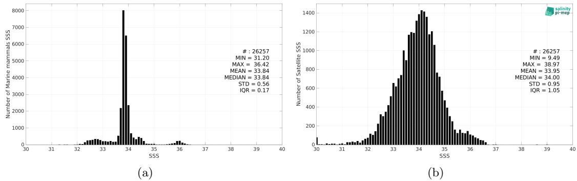
Figure 2: Histograms of SSS from Marine mammals (a) and Aquarius SSS L2 OR v5 (NASA-GSFC) (b) considering all match-up pairs per bins of 0.1 over the Global Ocean Pi-MEP region and for the full satellite product period.
