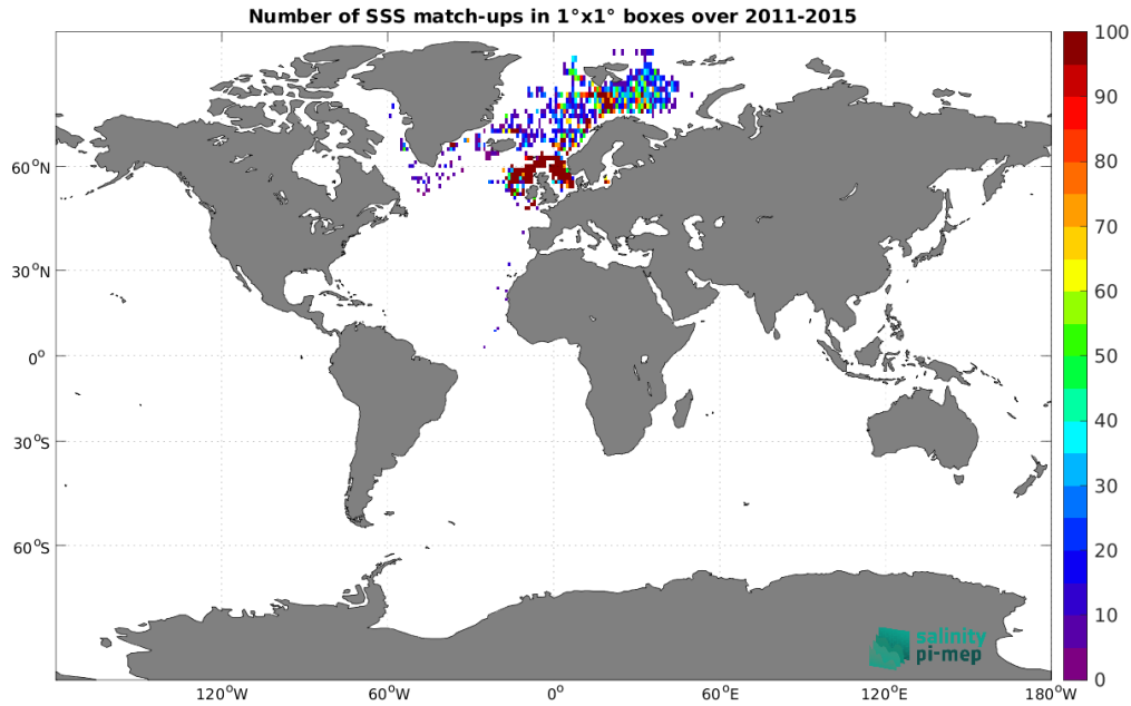
Figure 5: Number of SSS match-ups between ICES SSS and the Aquarius SSS L2 OR v5 (NASA-GSFC) SSS product for the Global Ocean Pi-MEP region over 1^\circ \times 1^\circ boxes and for the full satellite product period.
