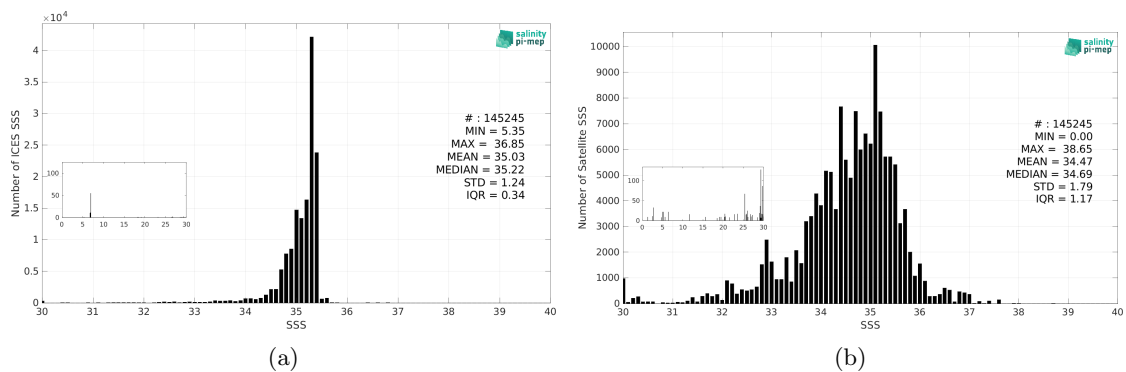
Figure 3: Histograms of SSS from ICES (a) and Aquarius SSS L2 OR v5 (NASA-GSFC) (b) considering all match-up pairs per bins of 0.1 over the Global Ocean Pi-MEP region and for the full satellite product period.
