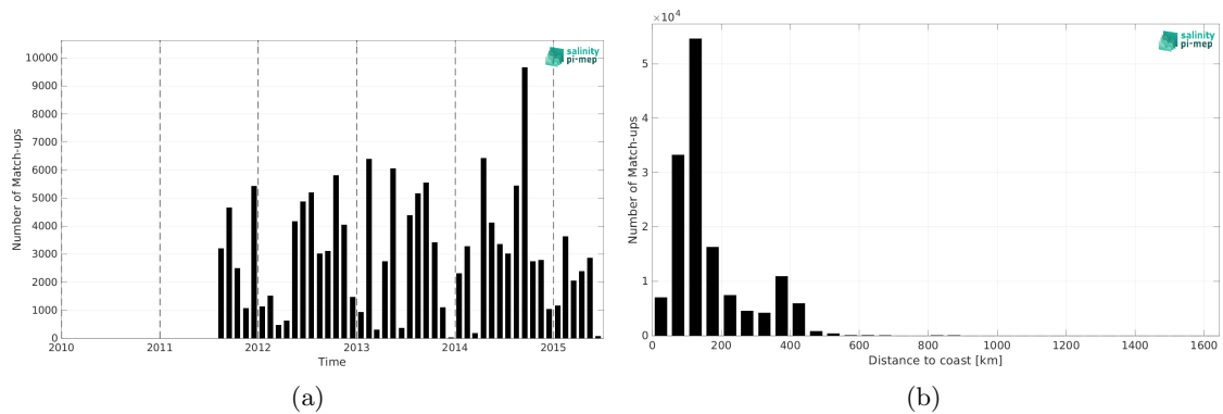
Figure 2: Number of match-ups between ICES and Aquarius SSS L2 OR v5 (NASA-GSFC) SSS as a function of time (a) and as function of the distance to coast (b) over the Global Ocean Pi-MEP region and for the full satellite product period.
