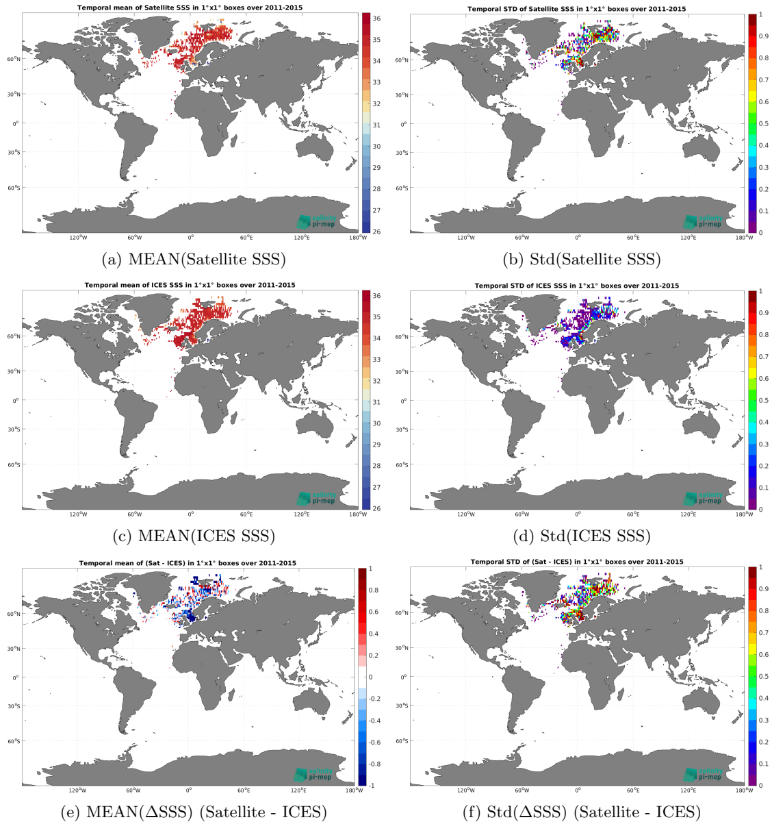
Figure 7: Temporal mean (left) and Std (right) of SSS from Aquarius SSS L2 OR v5 (NASA-GSFC) (top), ICES (middle), and of \Delta SSS (Satellite - ICES). Only match-up pairs are used to generate these maps.
