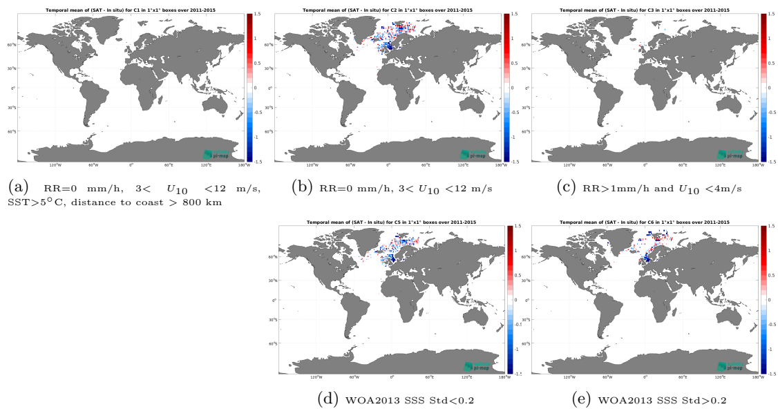
Figure 14: Temporal mean gridded over spatial boxes of size 1^\circ \times 1^\circ of \Delta\text{SSS} (Aquarius SSS L2 OR v5 (NASA-GSFC) - ICES) for 5 different subdatasets corresponding to:RR=0 mm/h, 3 < U_{10} < 12 m/s, SST > 5^\circ\text{C} , distance to coast > 800 km (a), RR=0 mm/h, 3 < U_{10} < 12 m/s (b), RR > 1 mm/h and U_{10} < 4 m/s (c), WOA2013 SSS Std < 0.2 (d), WOA2013 SSS Std > 0.2 (e).
