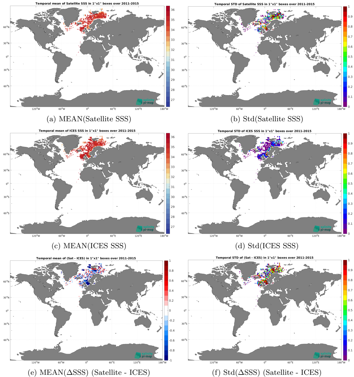
Figure 6: Temporal mean (left) and Std (right) of SSS from Aquarius SSS L2 OR v5 (NASA-GSFC) (top), ICES (middle), and of \Delta SSS (Satellite - ICES). Only match-up pairs are used to generate these maps.
