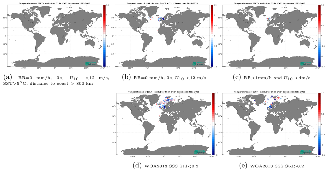
Figure 12: Temporal mean gridded over spatial boxes of size 1^\circ \times 1^\circ of \Delta SSS (Aquarius SSS L2 OR v5 (NASA-GSFC) - ICES) for 5 different subdatasets corresponding to:RR=0 mm/h, 3 < U_{10} < 12 m/s, SST > 5^\circ\text{C} , distance to coast > 800 km (a), RR=0 mm/h, 3 < U_{10} < 12 m/s (b), RR > 1 mm/h and U_{10} < 4 m/s (c), WOA2013 SSS Std < 0.2 (d), WOA2013 SSS Std > 0.2 (e).
