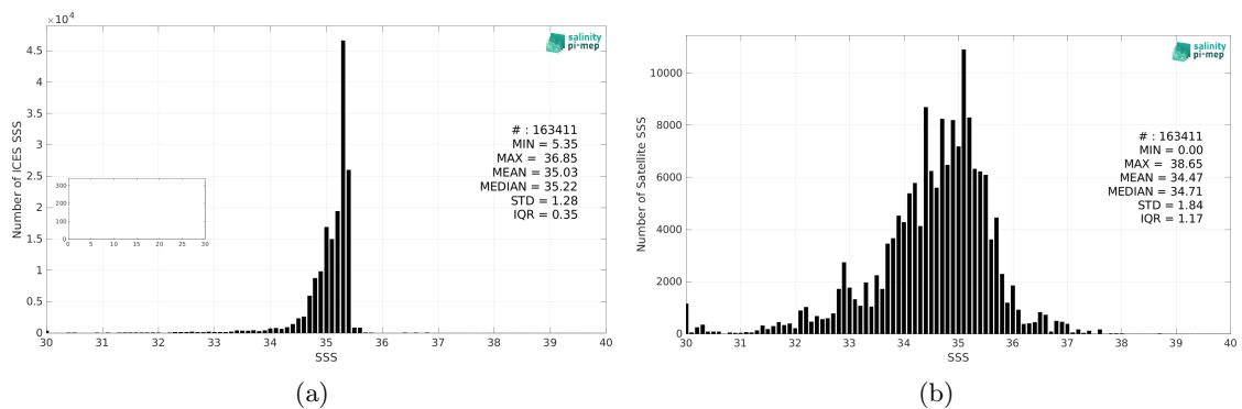
Figure 2: Histograms of SSS from ICES (a) and Aquarius SSS L2 OR v5 (NASA-GSFC) (b) considering all match-up pairs per bins of 0.1 over the Global Ocean Pi-MEP region and for the full satellite product period.
