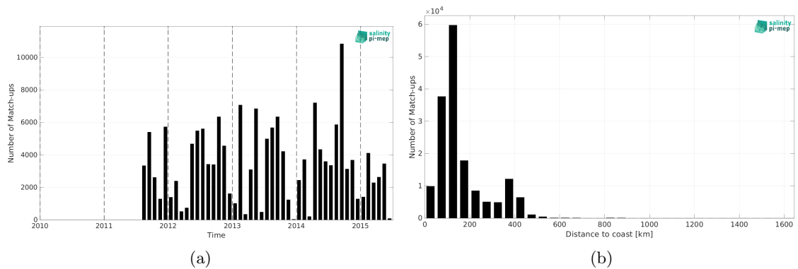
Figure 1: Number of match-ups between ICES and Aquarius SSS L2 OR v5 (NASA-GSFC) SSS as a function of time (a) and as function of the distance to coast (b) over the Global Ocean Pi-MEP region and for the full satellite product period.
