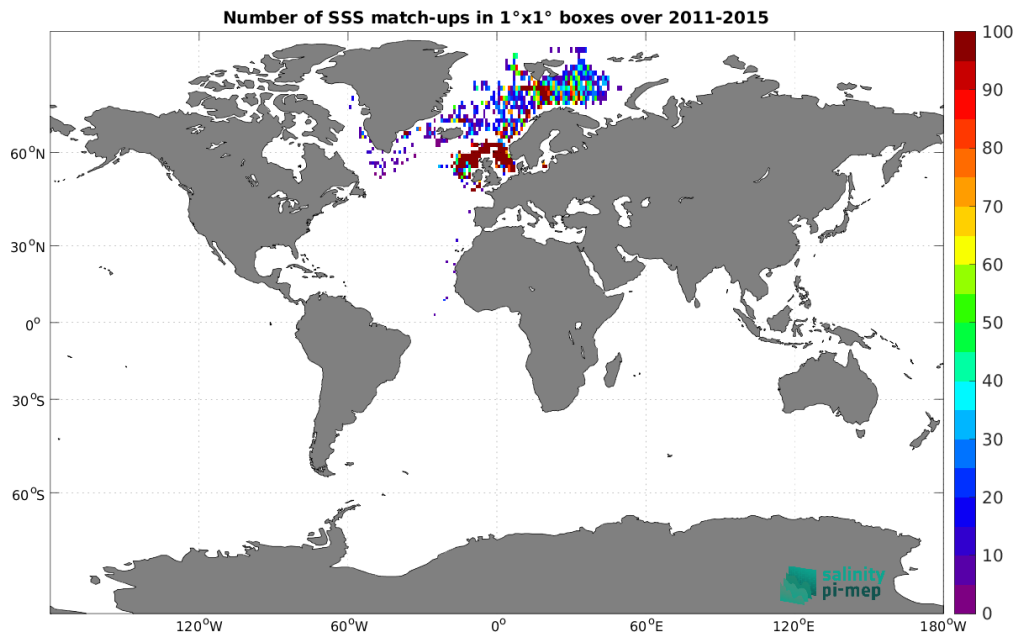
Figure 4: Number of SSS match-ups between ICES SSS and the Aquarius SSS L2 OR v5 (NASA-GSFC) SSS product for the Global Ocean Pi-MEP region over 1^\circ \times 1^\circ boxes and for the full satellite product period.
