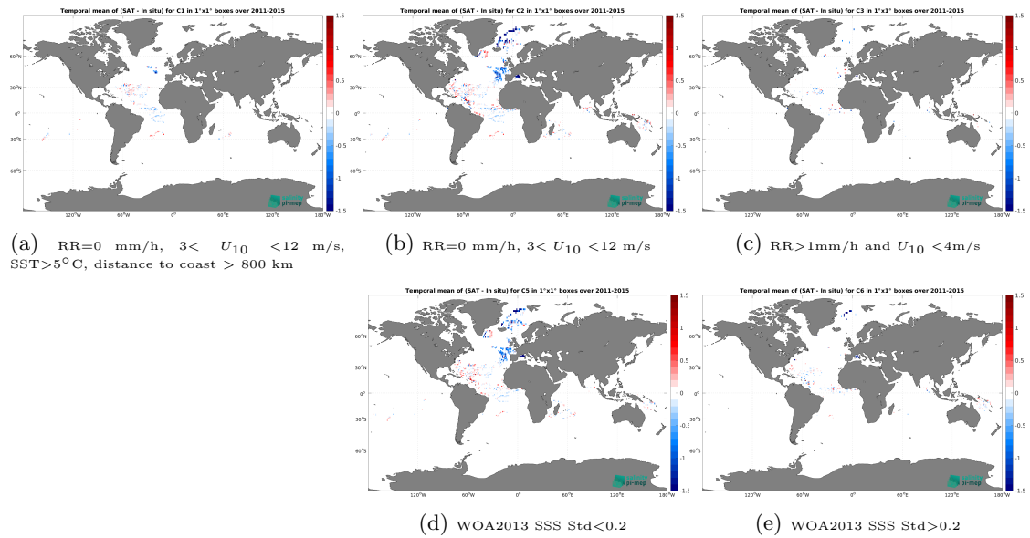
Figure 13: Temporal mean gridded over spatial boxes of size 1^\circ \times 1^\circ of \Delta SSS (Aquarius SSS L2 OR v5 (NASA-GSFC) - Surface drifters) for 5 different subdatasets corresponding to:RR=0 mm/h, 3 < U_{10} < 12 m/s, SST > 5^\circ\text{C} , distance to coast > 800 km (a), RR=0 mm/h, 3 < U_{10} < 12 m/s (b), RR > 1 mm/h and U_{10} < 4 m/s (c), WOA2013 SSS Std < 0.2 (d), WOA2013 SSS Std > 0.2 (e).
