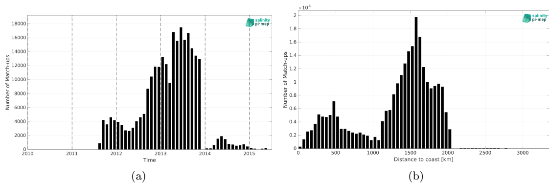
Figure 2: Number of match-ups between Surface drifters and Aquarius SSS L2 OR v5 (NASA-GSFC) SSS as a function of time (a) and as function of the distance to coast (b) over the Global Ocean Pi-MEP region and for the full satellite product period.
