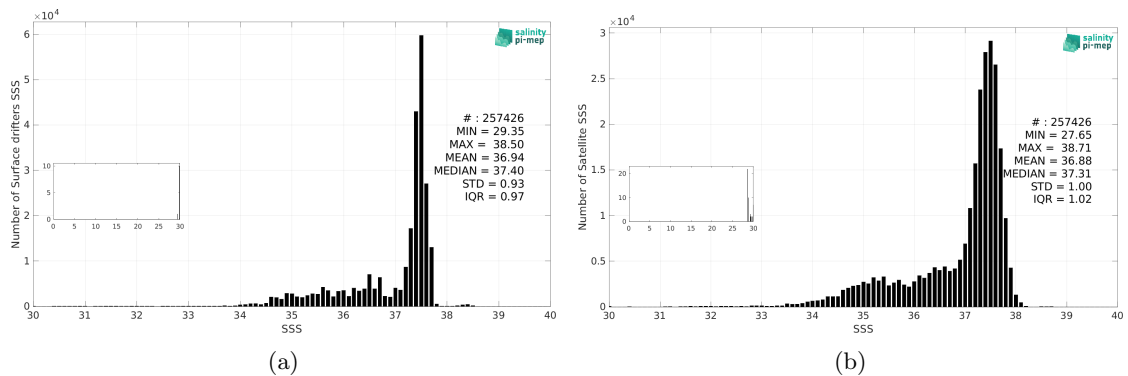
Figure 3: Histograms of SSS from Surface drifters (a) and Aquarius SSS L2 OR v5 (NASA-GSFC) (b) considering all match-up pairs per bins of 0.1 over the Global Ocean Pi-MEP region and for the full satellite product period.
