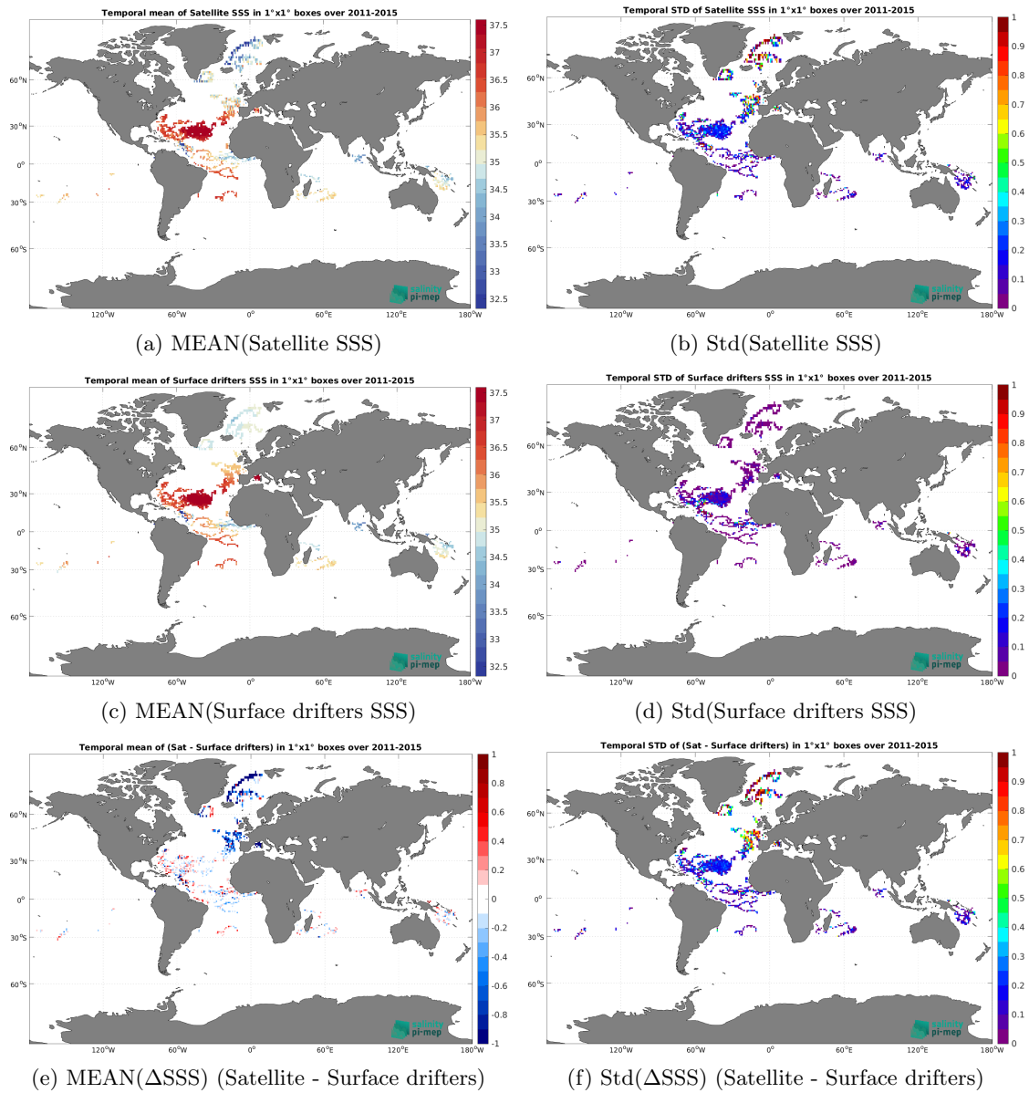
Figure 6: Temporal mean (left) and Std (right) of SSS from Aquarius SSS L2 OR v5 (NASA-GSFC) (top), Surface drifters (middle), and of \Delta SSS (Satellite - Surface drifters). Only match-up pairs are used to generate these maps.
