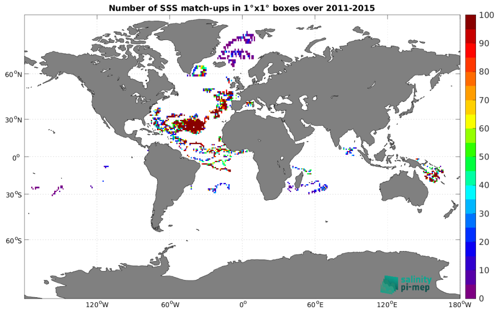
Figure 4: Number of SSS match-ups between Surface drifters SSS and the Aquarius SSS L2 OR v5 (NASA-GSFC) SSS product for the Global Ocean Pi-MEP region over 1^\circ \times 1^\circ boxes and for the full satellite product period.
