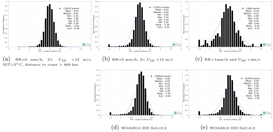
Figure 12: Normalized histogram of \Delta SSS (Aquarius-L2-OR-V5 - Surface drifters) for 5 different subdatasets corresponding to: RR=0 mm/h, 3 < U_{10} < 12 m/s, SST>5°C, distance to coast > 800 km (a), RR=0 mm/h, 3 < U_{10} < 12 m/s (b), RR>1mm/h and U_{10} < 4 m/s (c), WOA2013 SSS Std<0.2 (d), WOA2013 SSS Std>0.2 (e).
