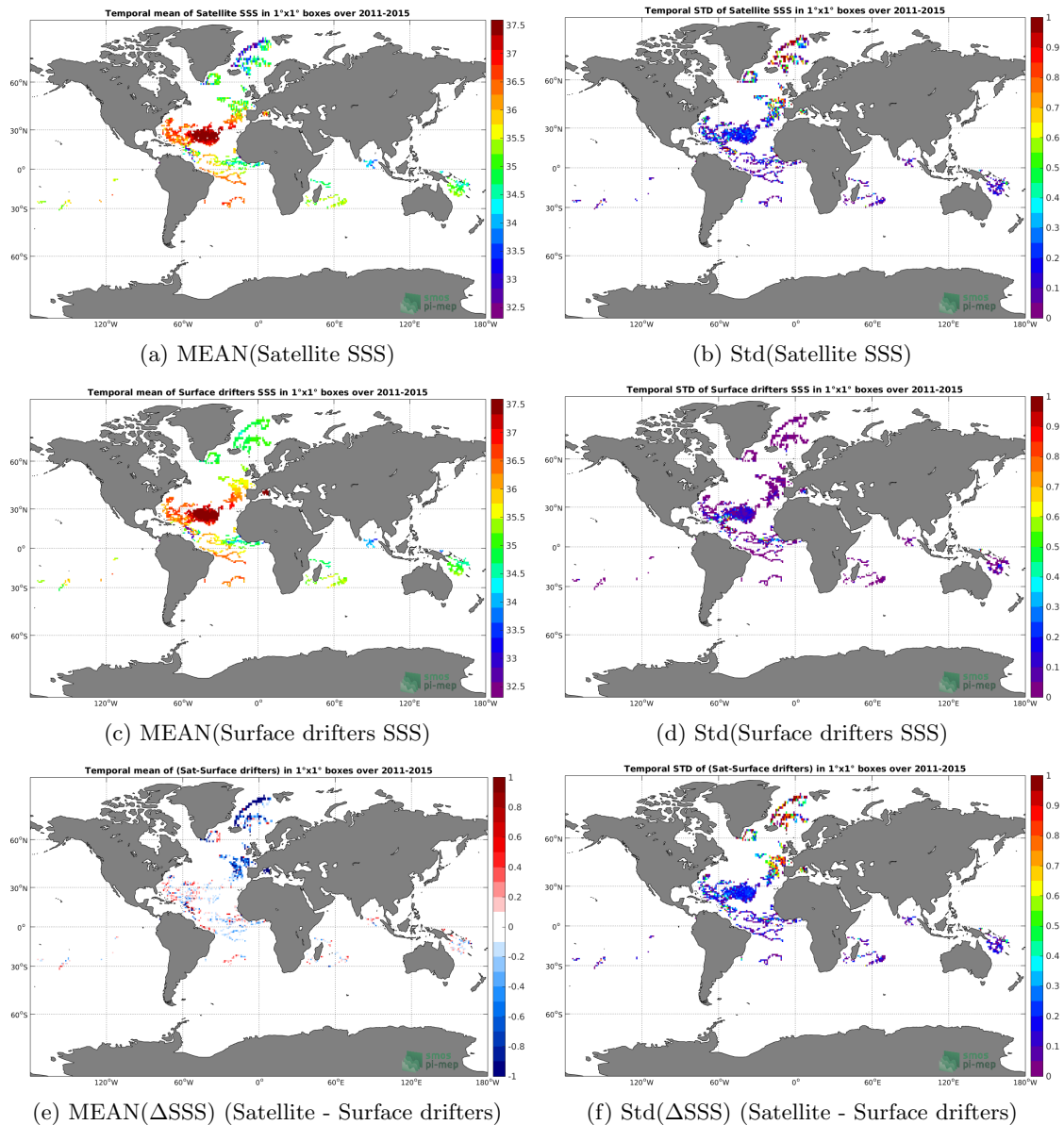
Figure 5: Temporal mean (left) and Std (right) of SSS from Aquarius-L2-OR-V5 (top), Surface drifters (middle), and of \Delta SSS (Satellite - Surface drifters). Only match-up pairs are used to generate these maps.
