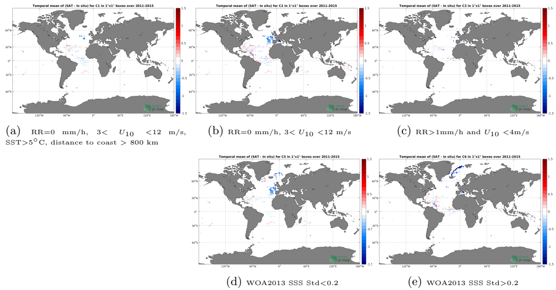
Figure 11: Temporal mean gridded over spatial boxes of size 1^\circ \times 1^\circ of \Delta SSS (Aquarius-L2-OR-V5 - Surface drifters) for 5 different subdatasets corresponding to:RR=0 mm/h, 3 < U_{10} < 12 m/s, SST > 5^\circ\text{C} , distance to coast > 800 km (a), RR=0 mm/h, 3 < U_{10} < 12 m/s (b), RR > 1 mm/h and U_{10} < 4 m/s (c), WOA2013 SSS Std < 0.2 (d), WOA2013 SSS Std > 0.2 (e).
