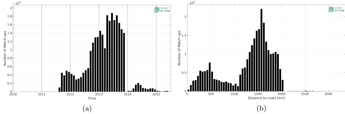
Figure 1: Number of match-ups between Surface drifters and Aquarius-L2-OR-V5 SSS as a function of time (a) and as function of the distance to coast (b) over the Global Ocean Pi-MEP region and for the full satellite product period.
