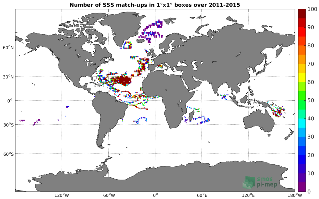
Figure 3: Number of SSS match-ups between Surface drifters SSS and the Aquarius-L2-OR-V5 SSS product for the Global Ocean Pi-MEP region over 1°x1° boxes and for the full satellite product period.
