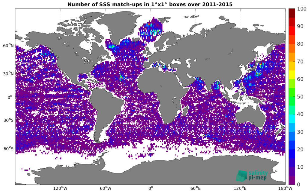
Figure 4: Number of SSS match-ups between Argo SSS and the Aquarius SSS L2 OR v5 (NASA-GSFC) SSS product for the Global Ocean Pi-MEP region over 1^\circ \times 1^\circ boxes and for the full satellite product period.
