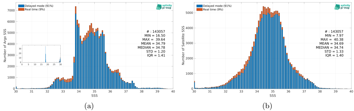
Figure 2: Histograms of SSS from Argo (a) and Aquarius SSS L2 OR v5 (NASA-GSFC) (b) considering all match-up pairs per bins of 0.1 over the Global Ocean Pi-MEP region and for the full satellite product period.
