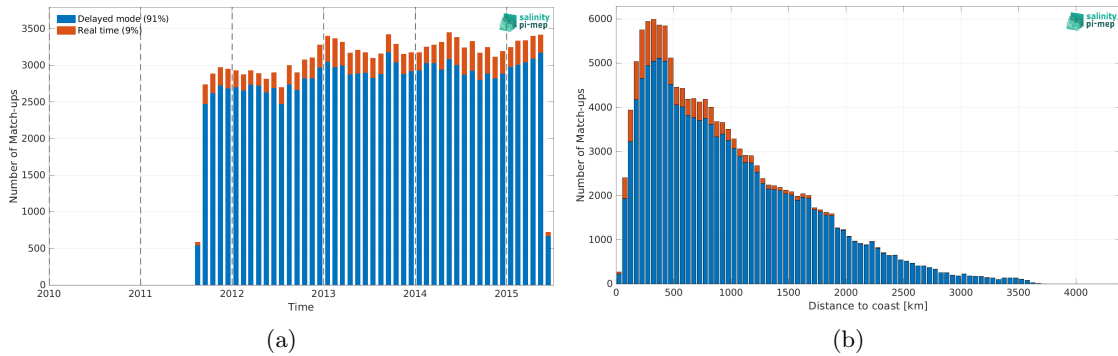
Figure 1: Number of match-ups between Argo and Aquarius SSS L2 OR v5 (NASA-GSFC) SSS as a function of time (a) and as function of the distance to coast (b) over the Global Ocean Pi-MEP region and for the full satellite product period.
