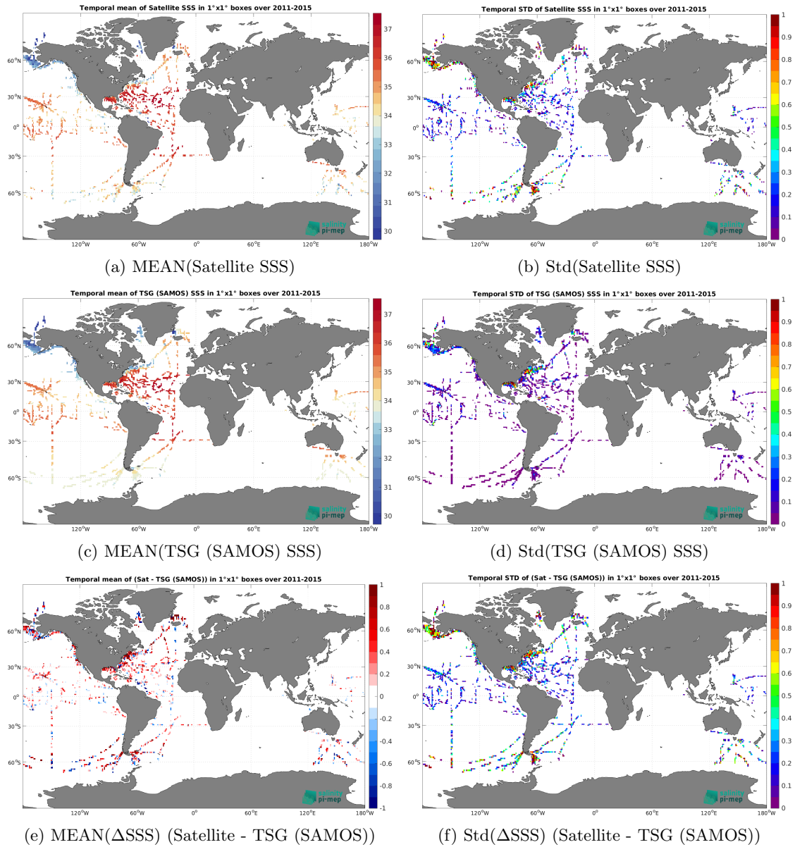
Figure 7: Temporal mean (left) and Std (right) of SSS from Aquarius SSS L2 CAP v5 (JPL) (top), TSG (SAMOS) (middle), and of \Delta SSS (Satellite - TSG (SAMOS)). Only match-up pairs are used to generate these maps.
