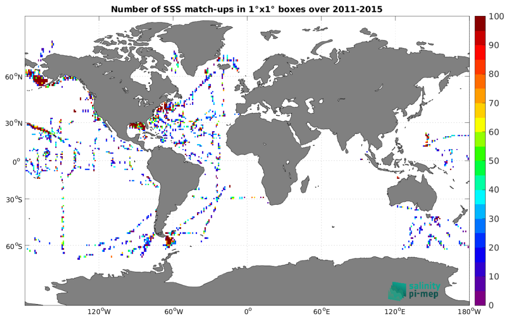
Figure 5: Number of SSS match-ups between TSG (SAMOS) SSS and the Aquarius SSS L2 CAP v5 (JPL) SSS product for the Global Ocean Pi-MEP region over 1^\circ \times 1^\circ boxes and for the full satellite product period.
