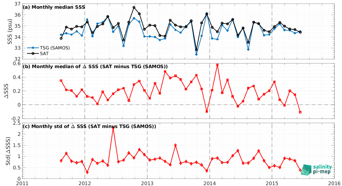
Figure 8: Time series of the monthly median SSS (top), median of \Delta\text{SSS} (Satellite - TSG (SAMOS)) and Std of \Delta\text{SSS} (Satellite - TSG (SAMOS)) over the Global Ocean Pi-MEP region considering all match-ups collected by the Pi-MEP.
