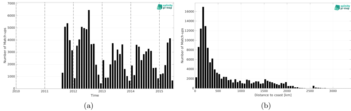
Figure 2: Number of match-ups between TSG (SAMOS) and Aquarius SSS L2 CAP v5 (JPL) SSS as a function of time (a) and as function of the distance to coast (b) over the Global Ocean Pi-MEP region and for the full satellite product period.
