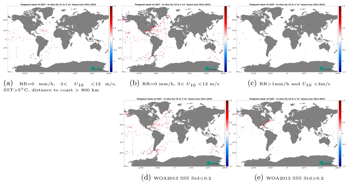
Figure 14: Temporal mean gridded over spatial boxes of size 1^\circ \times 1^\circ of \Delta\text{SSS} (Aquarius SSS L2 CAP v5 (JPL) - TSG (SAMOS)) for 5 different subdatasets corresponding to:RR=0 mm/h, 3 < U_{10} < 12 m/s, SST > 5^\circ\text{C} , distance to coast > 800 km (a), RR=0 mm/h, 3 < U_{10} < 12 m/s (b), RR > 1 mm/h and U_{10} < 4 m/s (c), WOA2013 SSS Std < 0.2 (d), WOA2013 SSS Std > 0.2 (e).
