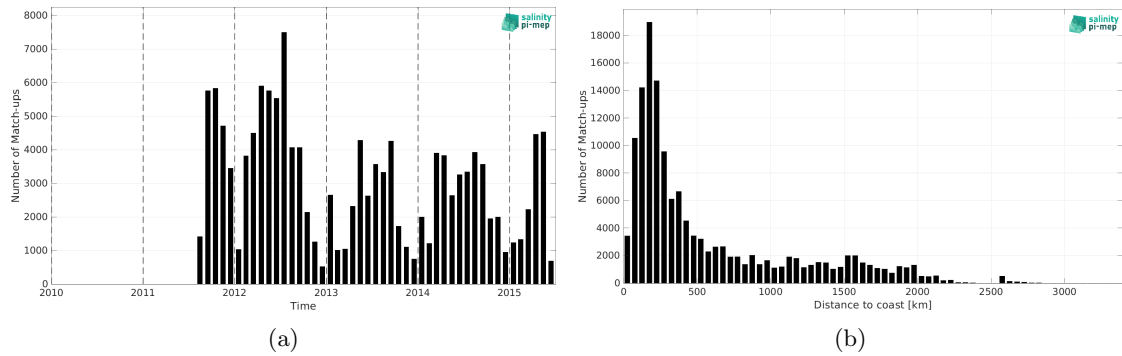
Figure 1: Number of match-ups between TSG (SAMOS) and Aquarius SSS L2 CAP v5 (JPL) SSS as a function of time (a) and as function of the distance to coast (b) over the Global Ocean Pi-MEP region and for the full satellite product period.
