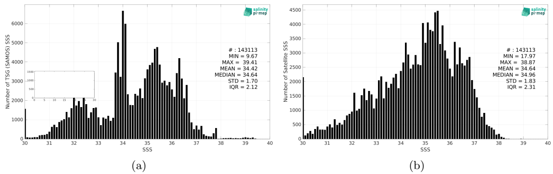
Figure 2: Histograms of SSS from TSG (SAMOS) (a) and Aquarius SSS L2 CAP v5 (JPL) (b) considering all match-up pairs per bins of 0.1 over the Global Ocean Pi-MEP region and for the full satellite product period.
