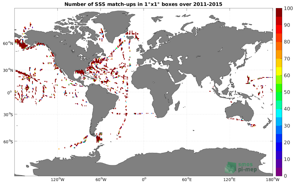
Figure 4: Number of SSS match-ups between TSG (SAMOS) SSS and the Aquarius SSS L2 CAP v5 (JPL) SSS product for the Global Ocean Pi-MEP region over 1^\circ \times 1^\circ boxes and for the full satellite product period.
