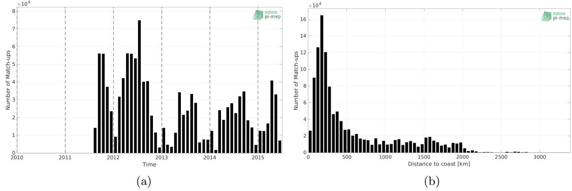
Figure 1: Number of match-ups between TSG (SAMOS) and Aquarius SSS L2 CAP v5 (JPL) SSS as a function of time (a) and as function of the distance to coast (b) over the Global Ocean Pi-MEP region and for the full satellite product period.
