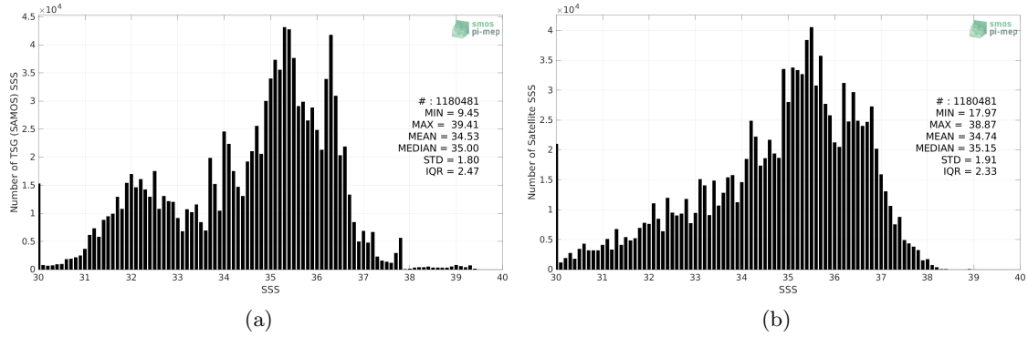
Figure 2: Histograms of SSS from TSG (SAMOS) (a) and Aquarius SSS L2 CAP v5 (JPL) (b) considering all match-up pairs per bins of 0.1 over the Global Ocean Pi-MEP region and for the full satellite product period.
