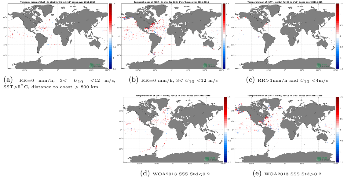
Figure 12: Temporal mean gridded over spatial boxes of size 1^\circ \times 1^\circ of \Delta SSS (Aquarius-L2-JPL-V5 - TSG-SAMOS) for 5 different subdatasets corresponding to:RR=0 mm/h, 3 < U_{10} < 12 m/s, SST >5^\circ C, distance to coast > 800 km (a), RR=0 mm/h, 3 < U_{10} < 12 m/s (b), RR >1 mm/h and U_{10} < 4 m/s (c), WOA2013 SSS Std <0.2 (d), WOA2013 SSS Std >0.2 (e).
