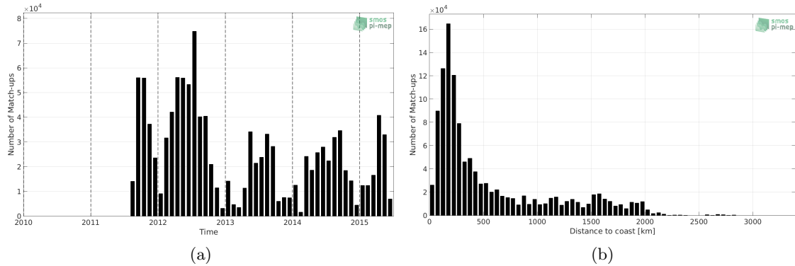
Figure 1: Number of match-ups between TSG-SAMOS and Aquarius-L2-JPL-V5 SSS as a function of time (a) and as function of the distance to coast (b) over the Global Ocean Pi-MEP region and for the full satellite product period.
