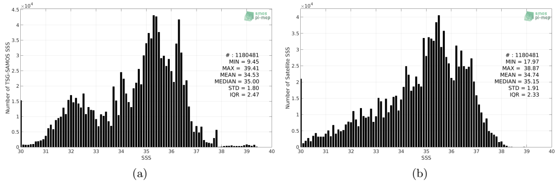
Figure 2: Histograms of SSS from TSG-SAMOS (a) and Aquarius-L2-JPL-V5 (b) considering all match-up pairs per bins of 0.1 over the Global Ocean Pi-MEP region and for the full satellite product period.
