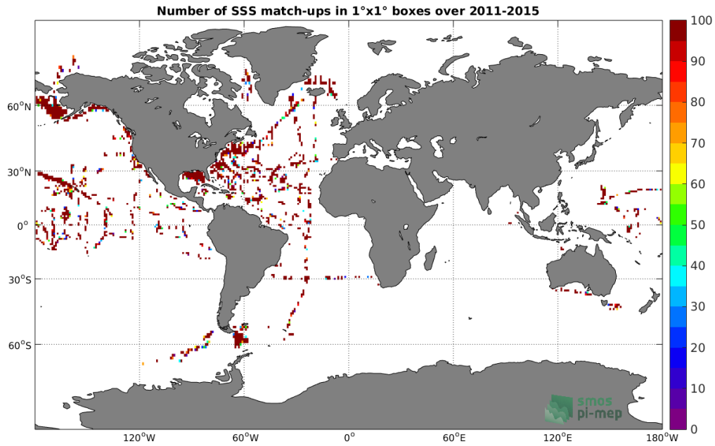
Figure 4: Number of SSS match-ups between TSG-SAMOS SSS and the Aquarius-L2-JPL-V5 SSS product for the Global Ocean Pi-MEP region over 1^\circ \times 1^\circ boxes and for the full satellite product period.
