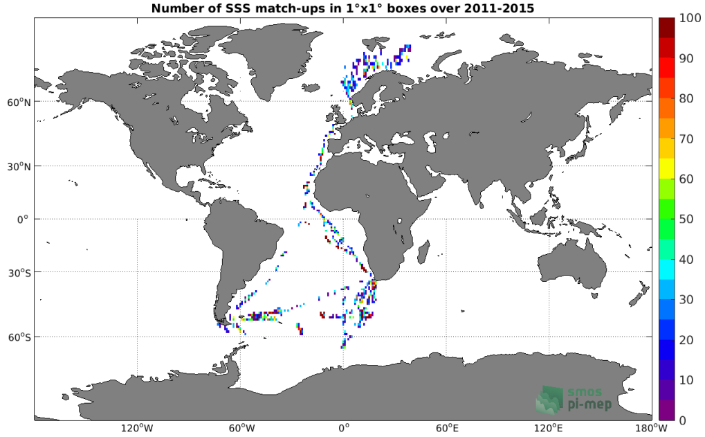
Figure 4: Number of SSS match-ups between TSG (Polarstern) SSS and the Aquarius SSS L2 CAP v5 (JPL) SSS product for the Global Ocean Pi-MEP region over 1^\circ \times 1^\circ boxes and for the full satellite product period.
