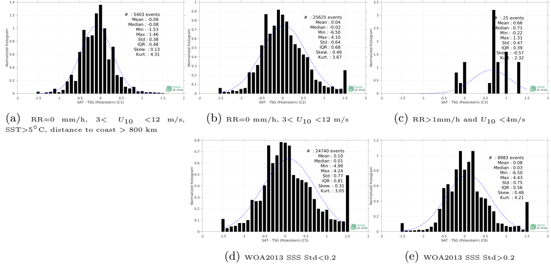
Figure 13: Normalized histogram of \Delta\text{SSS} (Aquarius SSS L2 CAP v5 (JPL) - TSG (Polarstern)) for 5 different subdatasets corresponding to: RR=0 mm/h, 3 < U_{10} < 12 m/s, SST>5°C, distance to coast > 800 km (a), RR=0 mm/h, 3 < U_{10} < 12 m/s (b), RR>1mm/h and U_{10} < 4 m/s (c), WOA2013 SSS Std<0.2 (d), WOA2013 SSS Std>0.2 (e).
