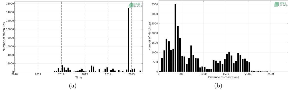
Figure 1: Number of match-ups between TSG (Polarstern) and Aquarius SSS L2 CAP v5 (JPL) SSS as a function of time (a) and as function of the distance to coast (b) over the Global Ocean Pi-MEP region and for the full satellite product period.
