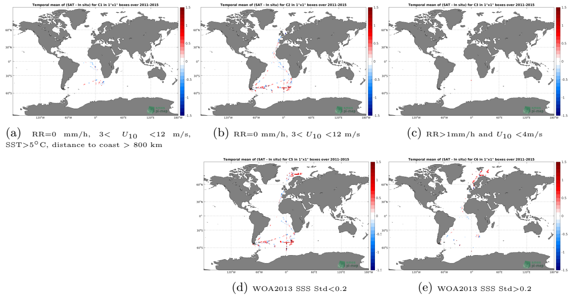
Figure 12: Temporal mean gridded over spatial boxes of size 1^\circ \times 1^\circ of \Delta SSS (Aquarius SSS L2 CAP v5 (JPL) - TSG (Polarstern)) for 5 different subdatasets corresponding to: RR=0 mm/h, 3 < U_{10} < 12 m/s, SST > 5^\circ\text{C} , distance to coast > 800 km (a), RR=0 mm/h, 3 < U_{10} < 12 m/s (b), RR > 1 mm/h and U_{10} < 4 m/s (c), WOA2013 SSS Std < 0.2 (d), WOA2013 SSS Std > 0.2 (e).
