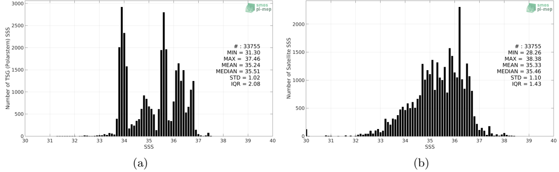
Figure 2: Histograms of SSS from TSG (Polarstern) (a) and Aquarius SSS L2 CAP v5 (JPL) (b) considering all match-up pairs per bins of 0.1 over the Global Ocean Pi-MEP region and for the full satellite product period.
