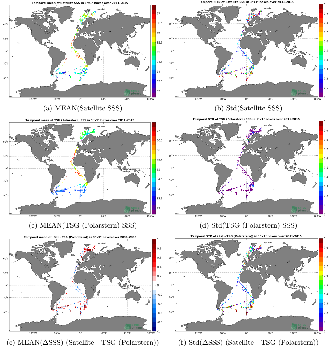
Figure 6: Temporal mean (left) and Std (right) of SSS from Aquarius SSS L2 CAP v5 (JPL) (top), TSG (Polarstern) (middle), and of \Delta SSS (Satellite - TSG (Polarstern)). Only match-up pairs are used to generate these maps.
