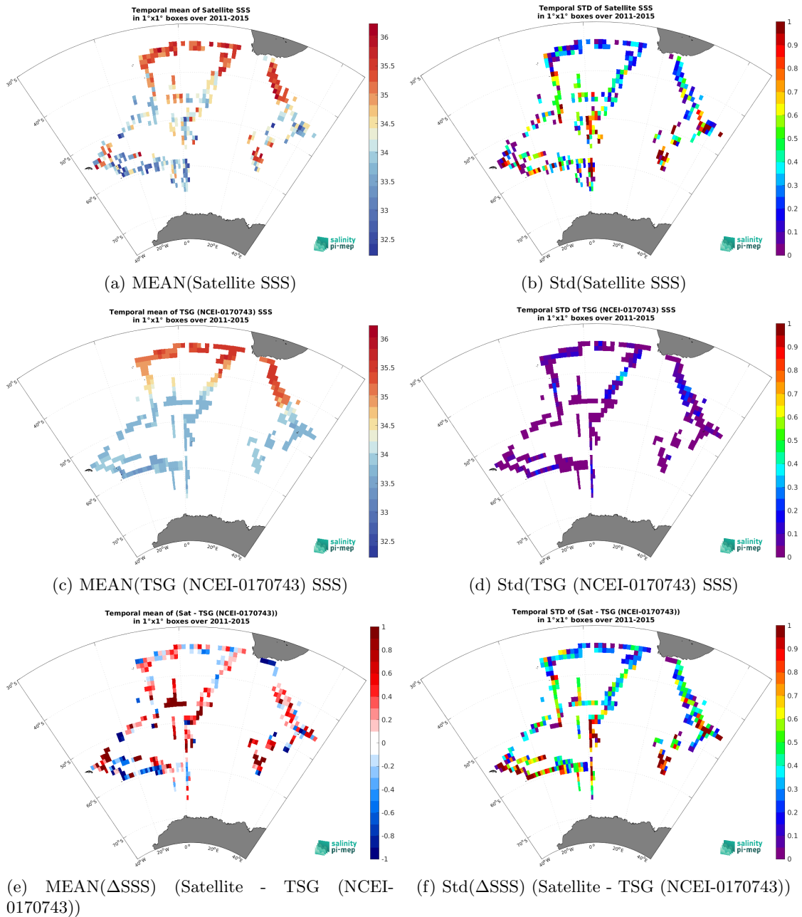
Figure 6: Temporal mean (left) and Std (right) of SSS from Aquarius SSS L2 CAP v5 (JPL) (top), TSG (NCEI-0170743) (middle), and of \Delta SSS (Satellite - TSG (NCEI-0170743)). Only match-up pairs are used to generate these maps.
