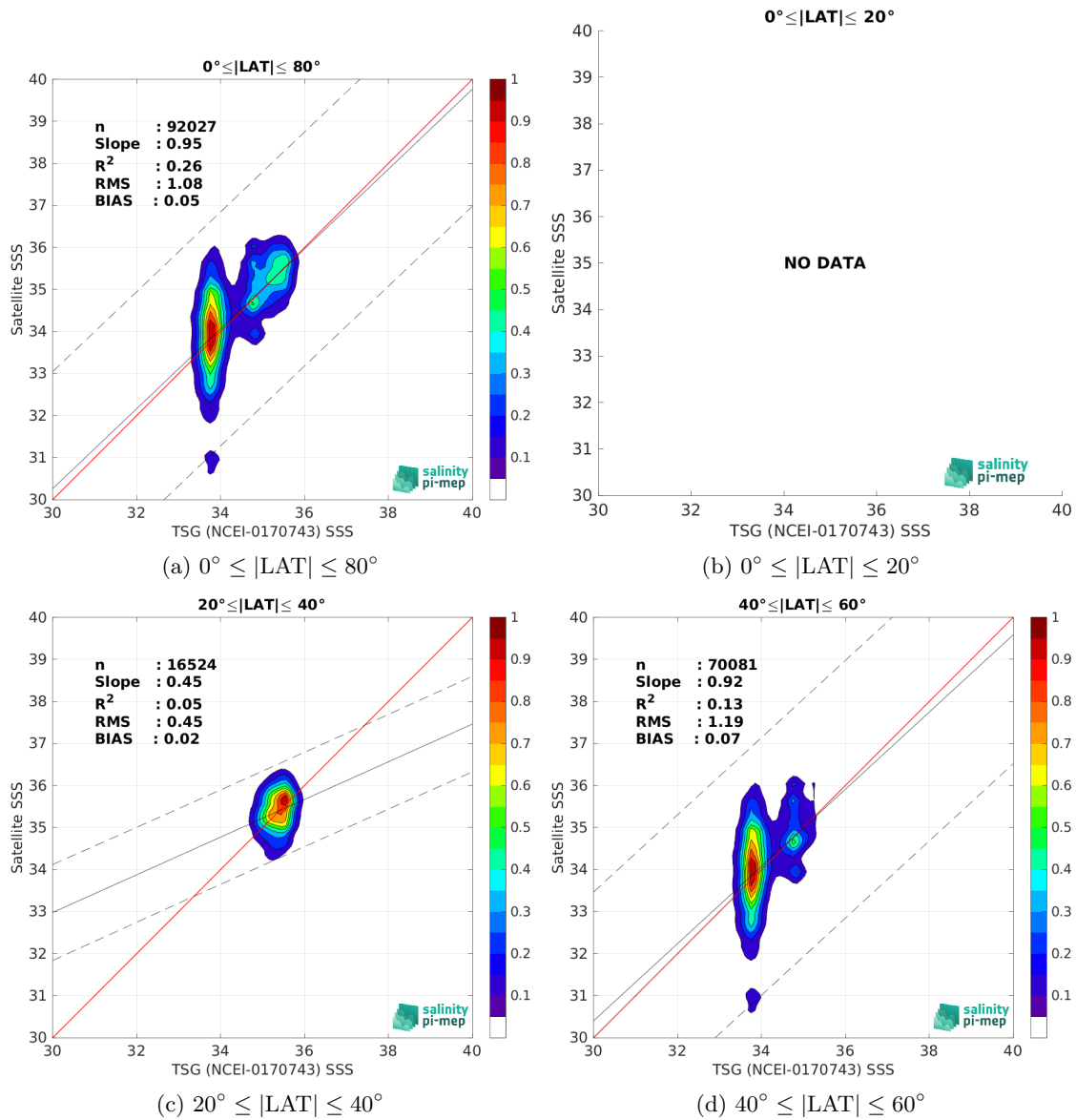
Figure 9: Contour maps of the concentration of Aquarius SSS L2 CAP v5 (JPL) SSS (y-axis) versus TSG (NCEI-0170743) SSS (x-axis) at match-up pairs for different latitude bands. For each plot, the red line shows x=y . The black thin and dashed lines indicate a linear fit through the data cloud and the \pm 95\% confidence levels, respectively. The number match-up pairs n , the slope and R^2 coefficient of the linear fit, the root mean square (RMS) and the mean bias between satellite and in situ data are indicated for each latitude band in each plots.
