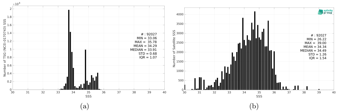
Figure 2: Histograms of SSS from TSG (NCEI-0170743) (a) and Aquarius SSS L2 CAP v5 (JPL) (b) considering all match-up pairs per bins of 0.1 over the Global Ocean Pi-MEP region and for the full satellite product period.
