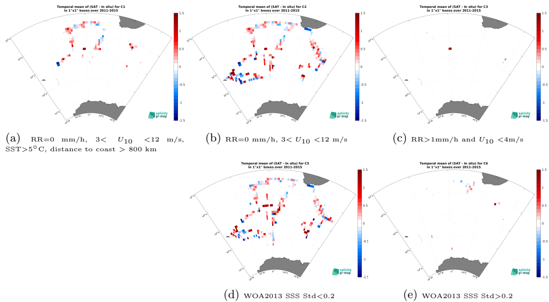
Figure 12: Temporal mean gridded over spatial boxes of size 1^\circ \times 1^\circ of \Delta SSS (Aquarius SSS L2 CAP v5 (JPL) - TSG (NCEI-0170743)) for 5 different subdatasets corresponding to:RR=0 mm/h, 3 < U_{10} < 12 m/s, SST >5^\circ C, distance to coast > 800 km (a), RR=0 mm/h, 3 < U_{10} < 12 m/s (b), RR >1 mm/h and U_{10} < 4 m/s (c), WOA2013 SSS Std <0.2 (d), WOA2013 SSS Std >0.2 (e).
