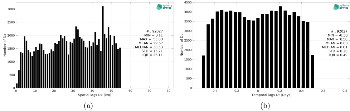
Figure 5: Histograms of the spatial (a) and temporal (b) lags between the location/time of the TSG (NCEI-0170743) measurement and the date of the corresponding Aquarius SSS L2 CAP v5 (JPL) SSS pixel.
