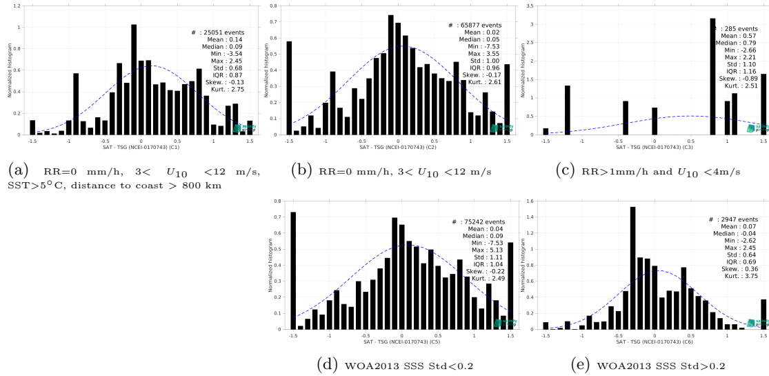
Figure 13: Normalized histogram of \Delta SSS (Aquarius SSS L2 CAP v5 (JPL) - TSG (NCEI-0170743)) for 5 different subdatasets corresponding to: RR=0 mm/h, 3 < U_{10} < 12 m/s, SST > 5°C, distance to coast > 800 km (a), RR=0 mm/h, 3 < U_{10} < 12 m/s (b), RR > 1mm/h and U_{10} < 4 m/s (c), WOA2013 SSS Std < 0.2 (d), WOA2013 SSS Std > 0.2 (e).
