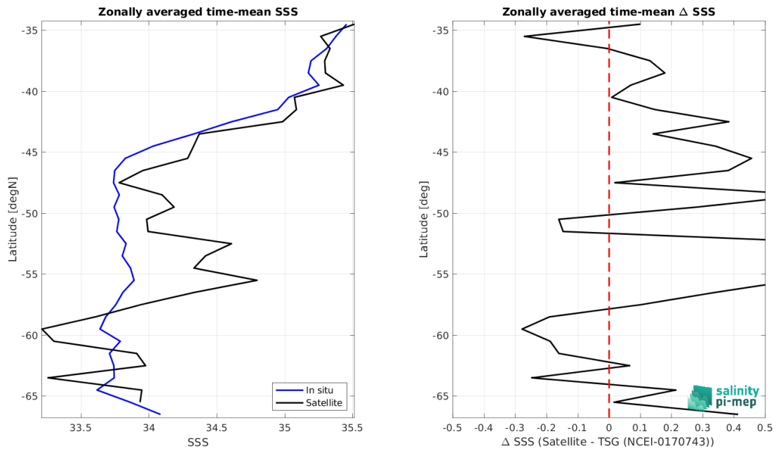
Figure 8: Left panel: Zonal mean SSS from Aquarius SSS L2 CAP v5 (JPL) satellite product (black) and from TSG (NCEI-0170743) (blue). Right panel: Zonal mean of \Delta SSS (Satellite - TSG (NCEI-0170743)) for all the collected Pi-MEP match-up pairs estimated over the full satellite product period.
