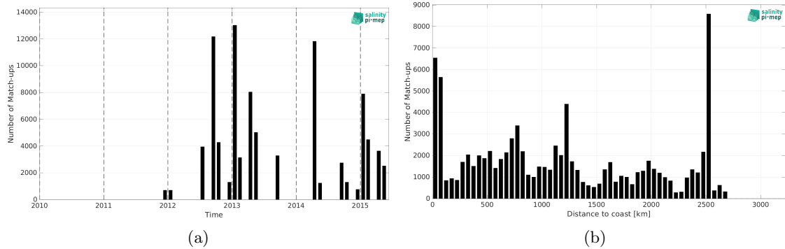
Figure 1: Number of match-ups between TSG (NCEI-0170743) and Aquarius SSS L2 CAP v5 (JPL) SSS as a function of time (a) and as function of the distance to coast (b) over the Global Ocean Pi-MEP region and for the full satellite product period.
