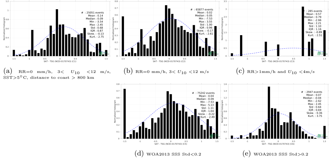
Figure 13: Normalized histogram of \Delta SSS (Aquarius SSS L2 CAP v5 (JPL) - TSG (NCEI-0170743)) for 5 different subdatasets corresponding to: RR=0 mm/h, 3 < U_{10} < 12 m/s, SST > 5°C, distance to coast > 800 km (a), RR=0 mm/h, 3 < U_{10} < 12 m/s (b), RR > 1mm/h and U_{10} < 4 m/s (c), WOA2013 SSS Std < 0.2 (d), WOA2013 SSS Std > 0.2 (e).
