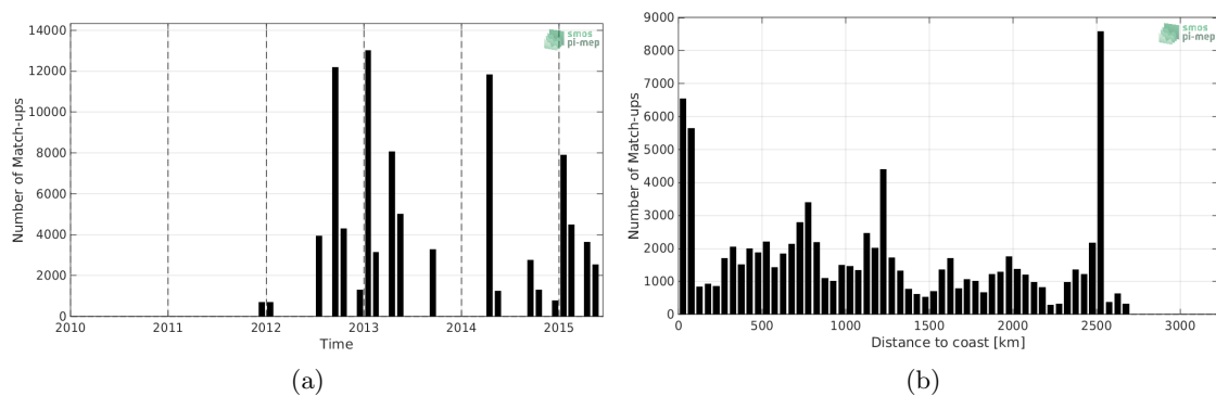
Figure 1: Number of match-ups between TSG-NCEI-0170743 and Aquarius-L2-JPL-V5 SSS as a function of time (a) and as function of the distance to coast (b) over the Global Ocean Pi-MEP region and for the full satellite product period.
