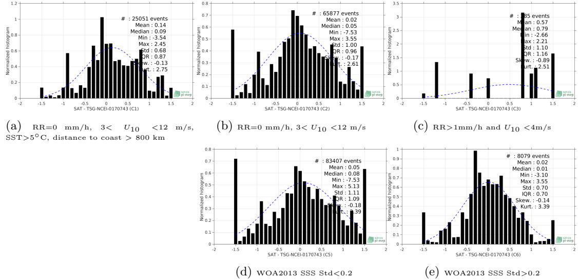
Figure 13: Normalized histogram of \Delta SSS (Aquarius-L2-JPL-V5 - TSG-NCEI-0170743) for 5 different subdatasets corresponding to: RR=0 mm/h, 3 < U_{10} < 12 m/s, SST>5°C, distance to coast > 800 km (a), RR=0 mm/h, 3 < U_{10} < 12 m/s (b), RR>1mm/h and U_{10} < 4 m/s (c), WOA2013 SSS Std<0.2 (d), WOA2013 SSS Std>0.2 (e).
