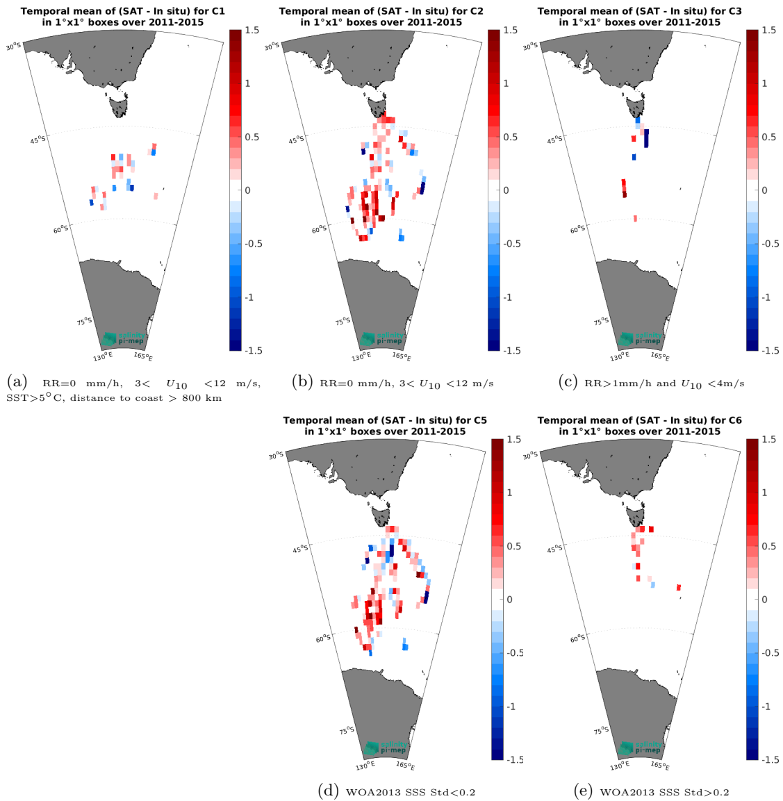
Figure 14: Temporal mean gridded over spatial boxes of size 1^\circ \times 1^\circ of \Delta SSS (Aquarius SSS L2 CAP v5 (JPL) - TSG (LEGOS-Survostral)) for 5 different subdatasets corresponding to: RR=0 mm/h, 3 < U_{10} < 12 m/s, SST > 5°C, distance to coast > 800 km (a), RR=0 mm/h, 3 < U_{10} < 12 m/s (b), RR > 1mm/h and U_{10} < 4 m/s (c), WOA2013 SSS Std < 0.2 (d), WOA2013 SSS Std > 0.2 (e).
