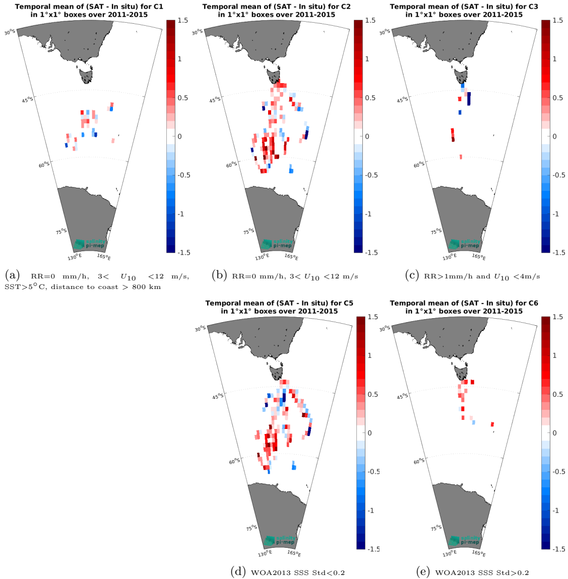
Figure 14: Temporal mean gridded over spatial boxes of size 1^\circ \times 1^\circ of \Delta SSS (Aquarius SSS L2 CAP v5 (JPL) - TSG (LEGOS-Survostral)) for 5 different subdatasets corresponding to:RR=0 mm/h, 3 < U_{10} < 12 m/s, SST>5°C, distance to coast > 800 km (a), RR=0 mm/h, 3 < U_{10} < 12 m/s (b), RR>1mm/h and U_{10} < 4 m/s (c), WOA2013 SSS Std<0.2 (d), WOA2013 SSS Std>0.2 (e).
