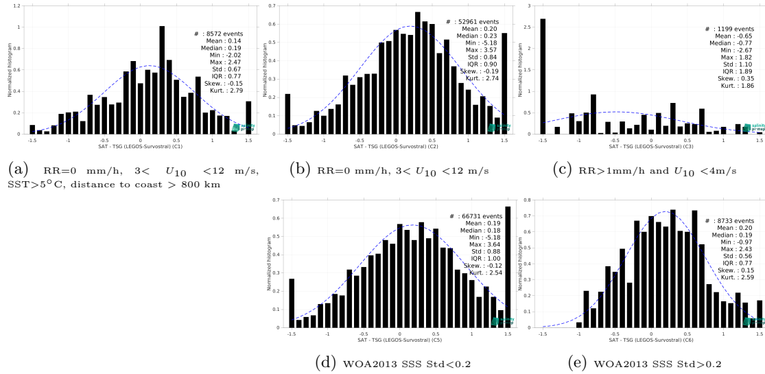
Figure 15: Normalized histogram of \Delta SSS (Aquarius SSS L2 CAP v5 (JPL) - TSG (LEGOS-Survostral)) for 5 different subdatasets corresponding to: RR=0 mm/h, 3 < U_{10} < 12 m/s, SST>5°C, distance to coast > 800 km (a), RR=0 mm/h, 3 < U_{10} < 12 m/s (b), RR>1mm/h and U_{10} < 4 m/s (c), WOA2013 SSS Std<0.2 (d), WOA2013 SSS Std>0.2 (e).
