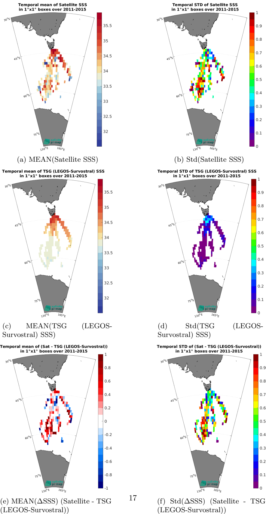
Figure 7: Temporal mean (left) and Std (right) of SSS from Aquarius SSS L2 CAP v5 (JPL) (top), TSG (LEGOS-Survostral) (middle), and of \Delta SSS (Satellite - TSG (LEGOS-Survostral)). Only match-up pairs are used to generate these maps.
