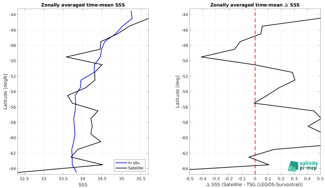
Figure 9: Left panel: Zonal mean SSS from Aquarius SSS L2 CAP v5 (JPL) satellite product (black) and from TSG (LEGOS-Survostral) (blue). Right panel: Zonal mean of \Delta SSS (Satellite - TSG (LEGOS-Survostral)) for all the collected Pi-MEP match-up pairs estimated over the full satellite product period.
