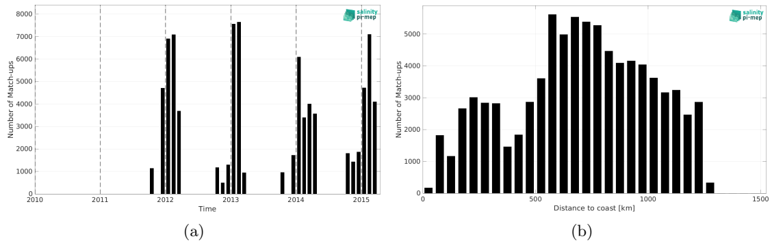
Figure 2: Number of match-ups between TSG (LEGOS-Survostral) and Aquarius SSS L2 CAP v5 (JPL) SSS as a function of time (a) and as function of the distance to coast (b) over the Global Ocean Pi-MEP region and for the full satellite product period.
