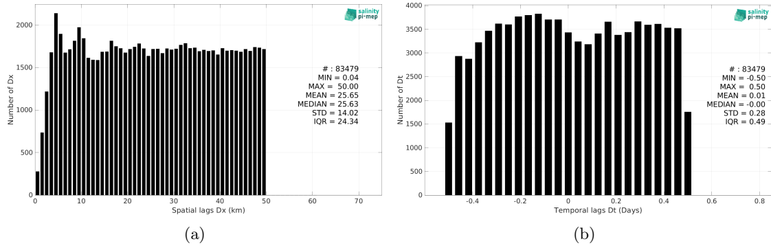
Figure 6: Histograms of the spatial (a) and temporal (b) lags between the location/time of the TSG (LEGOS-Survostral) measurement and the date of the corresponding Aquarius SSS L2 CAP v5 (JPL) SSS pixel.
