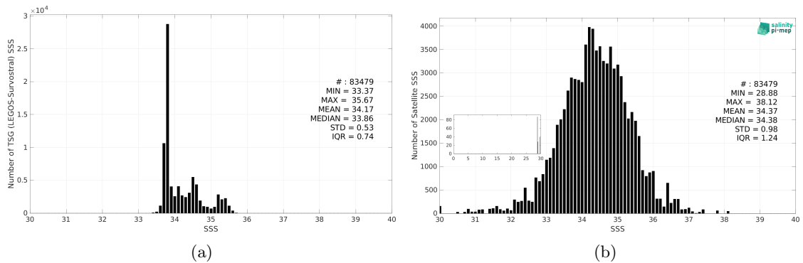
Figure 3: Histograms of SSS from TSG (LEGOS-Survostral) (a) and Aquarius SSS L2 CAP v5 (JPL) (b) considering all match-up pairs per bins of 0.1 over the Global Ocean Pi-MEP region and for the full satellite product period.
