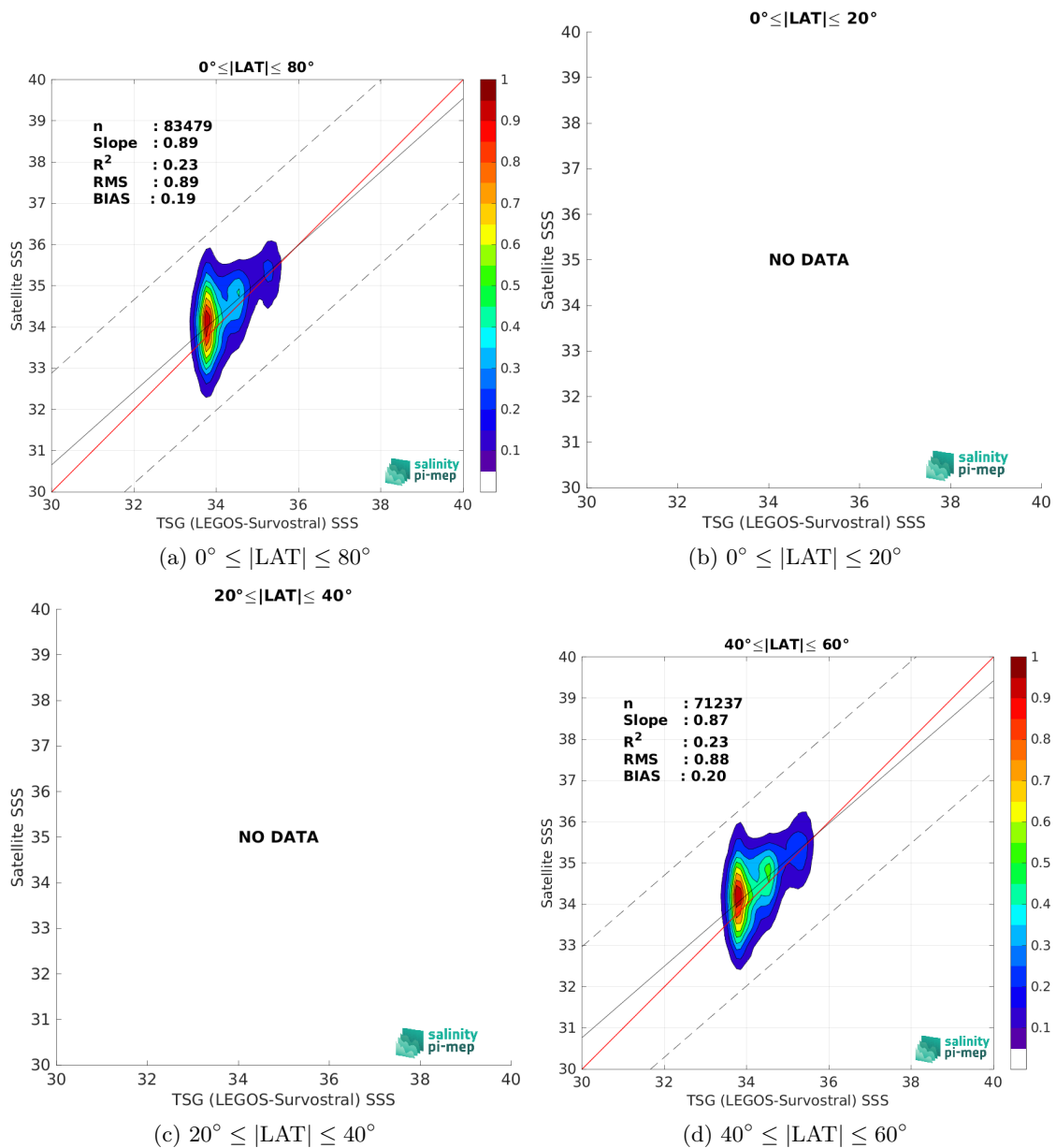
Figure 10: Contour maps of the concentration of Aquarius SSS L2 CAP v5 (JPL) SSS (y-axis) versus TSG (LEGOS-Survostral) SSS (x-axis) at match-up pairs for different latitude bands. For each plot, the red line shows x=y . The black thin and dashed lines indicate a linear fit through the data cloud and the \pm 95\% confidence levels, respectively. The number match-up pairs n , the slope and R^2 coefficient of the linear fit, the root mean square (RMS) and the mean bias between satellite and in situ data are indicated for each latitude band in each plot.
