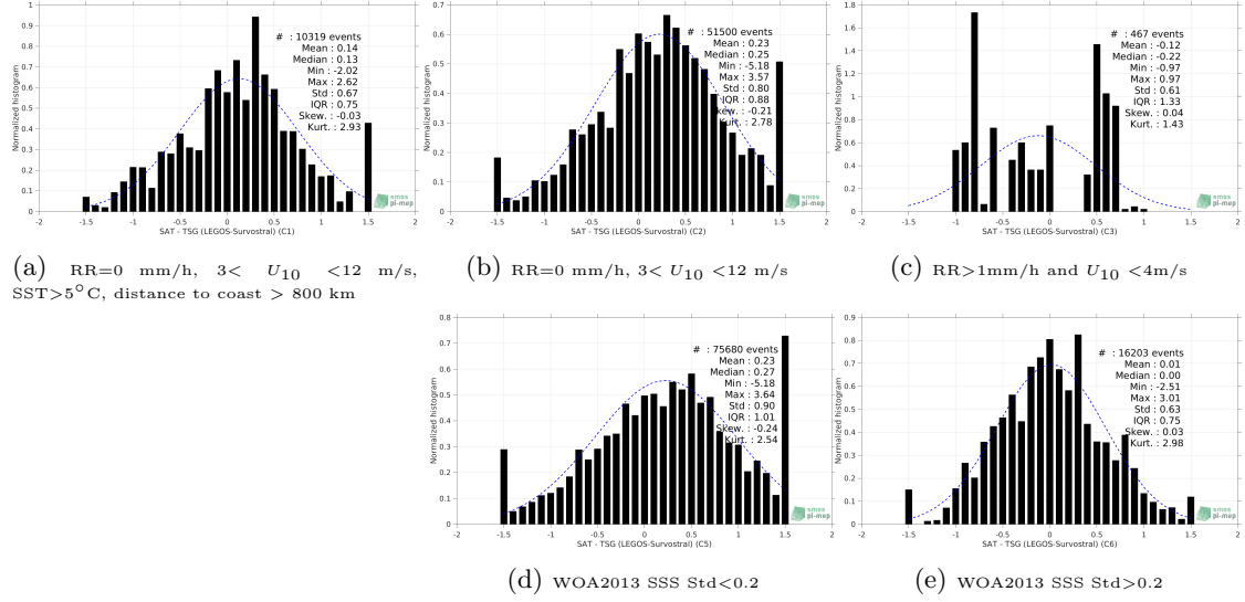
Figure 13: Normalized histogram of \Delta SSS (Aquarius SSS L2 CAP v5 (JPL) - TSG (LEGOS-Survostral)) for 5 different subdatasets corresponding to: RR=0 mm/h, 3 < U_{10} < 12 m/s, SST>5°C, distance to coast > 800 km (a), RR=0 mm/h, 3 < U_{10} < 12 m/s (b), RR>1mm/h and U_{10} < 4 m/s (c), WOA2013 SSS Std<0.2 (d), WOA2013 SSS Std>0.2 (e).
