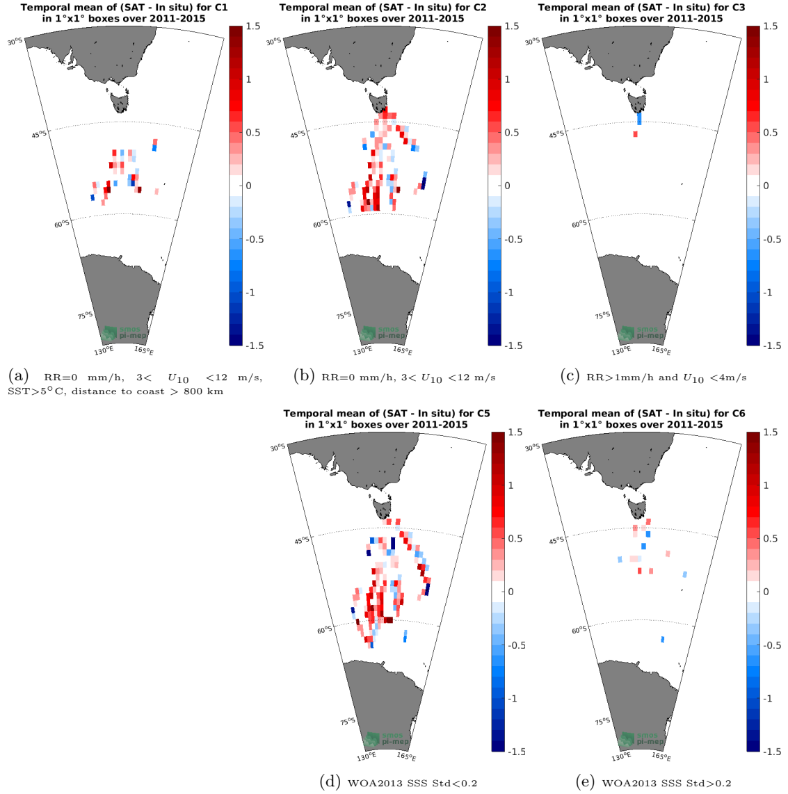
Figure 12: Temporal mean gridded over spatial boxes of size 1^{\circ} \times 1^{\circ} of \Delta\text{SSS} (Aquarius SSS L2 CAP v5 (JPL) - TSG (LEGOS-Survostral)) for 5 different subdatasets corresponding to: RR=0 mm/h, 3 < U_{10} < 12 m/s, SST > 5^{\circ}\text{C} , distance to coast > 800 km (a), RR=0 mm/h, 3 < U_{10} < 12 m/s (b), RR > 1 mm/h and U_{10} < 4 m/s (c), WOA2013 SSS Std < 0.2 (d), WOA2013 SSS Std > 0.2 (e).
