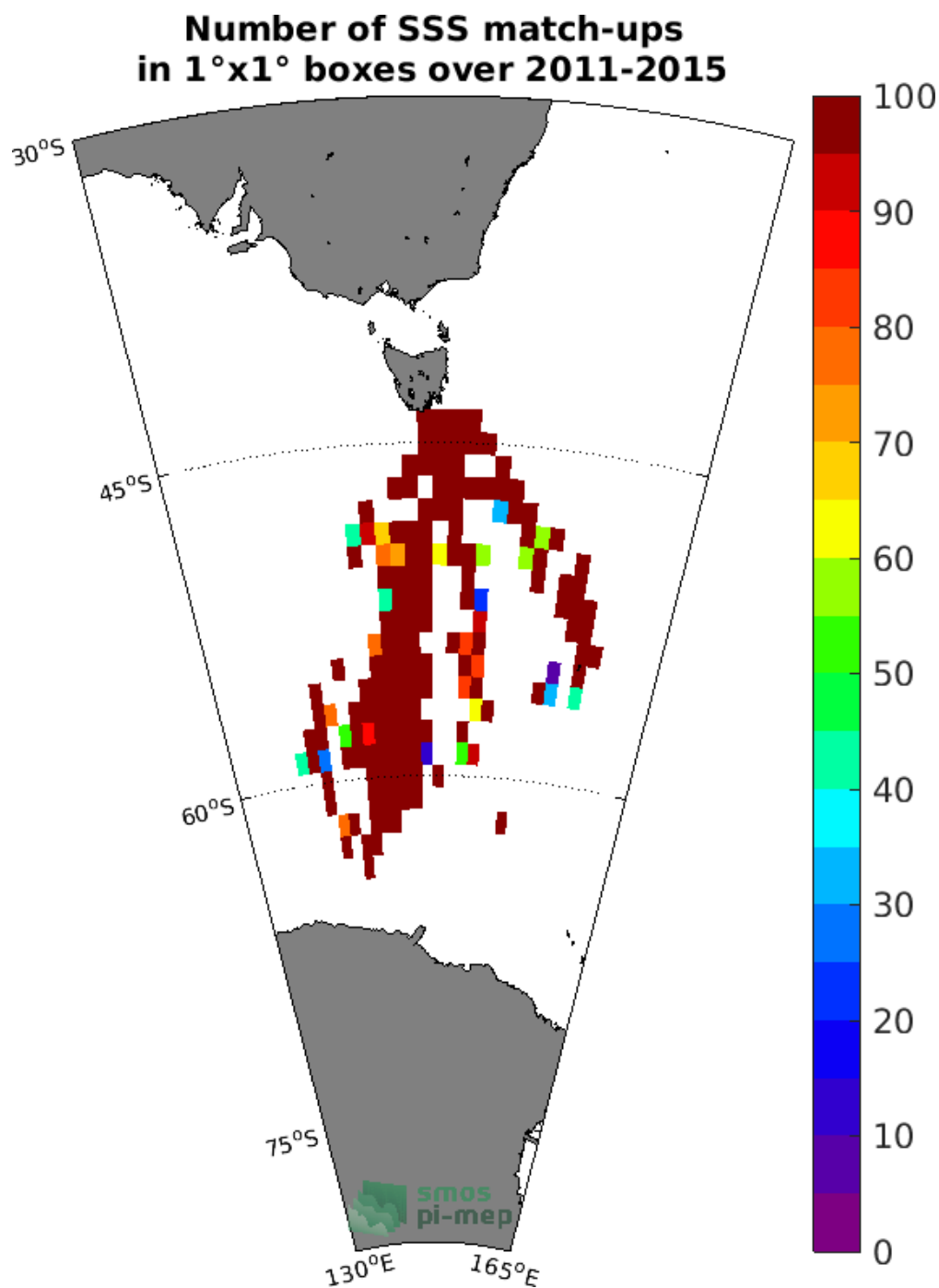
Figure 4: Number of SSS match-ups between TSG (LEGOS-Survostral) SSS and the Aquarius SSS L2 CAP v5 (JPL) SSS product for the Global Ocean Pi-MEP region over 1°x1° boxes and for the full satellite product period.
