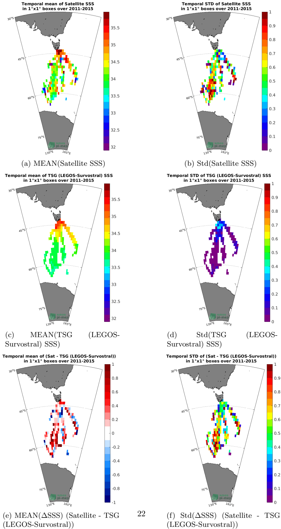
Figure 6: Temporal mean (left) and Std (right) of SSS from Aquarius SSS L2 CAP v5 (JPL) (top), TSG (LEGOS-Survostral) (middle), and of \Delta SSS (Satellite - TSG (LEGOS-Survostral)). Only match-up pairs are used to generate these maps.
