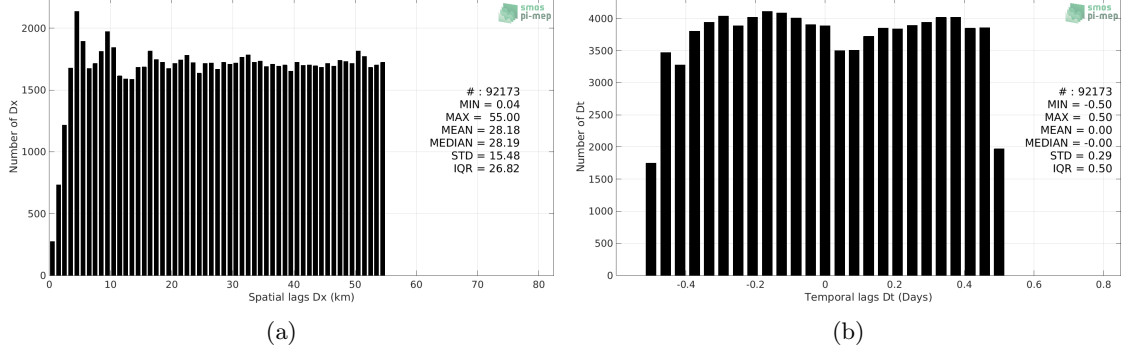
Figure 5: Histograms of the spatial (a) and temporal (b) lags between the time of the TSG (LEGOS-Survostral) measurements and the date of the corresponding Aquarius SSS L2 CAP v5 (JPL) SSS product.
