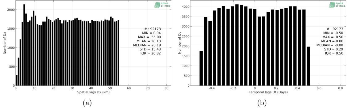
Figure 5: Histograms of the spatial (a) and temporal (b) lags between the time of the TSG-LEGOS-Survostral measurements and the date of the corresponding Aquarius-L2-JPL-V5 SSS product.
