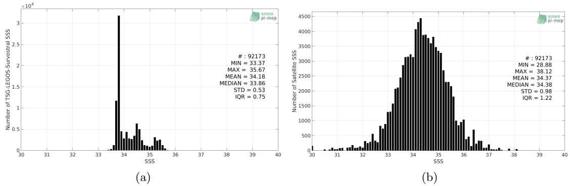
Figure 2: Histograms of SSS from TSG-LEGOS-Survostral (a) and Aquarius-L2-JPL-V5 (b) considering all match-up pairs per bins of 0.1 over the Global Ocean Pi-MEP region and for the full satellite product period.
