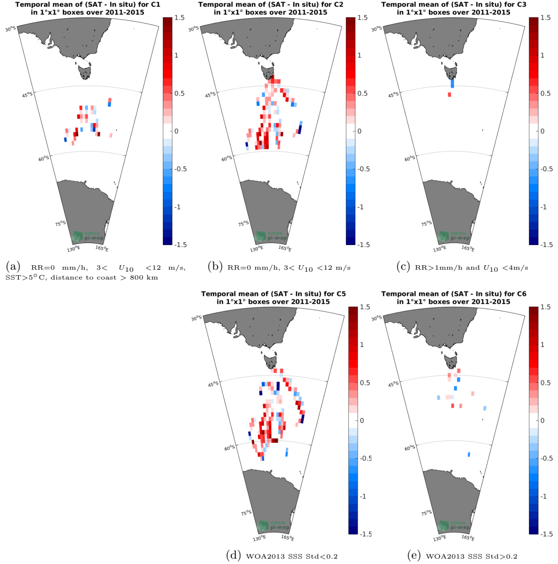
Figure 12: Temporal mean gridded over spatial boxes of size 1^\circ \times 1^\circ of \Delta\text{SSS} (Aquarius-L2-JPL-V5 - TSG-LEGOS-Survostral) for 5 different subdatasets corresponding to: RR=0 mm/h, 3 < U_{10} < 12 m/s, SST > 5^\circ\text{C} , distance to coast > 800 km (a), RR=0 mm/h, 3 < U_{10} < 12 m/s (b), RR > 1 mm/h and U_{10} < 4 m/s (c), WOA2013 SSS Std < 0.2 (d), WOA2013 SSS Std > 0.2 (e).
