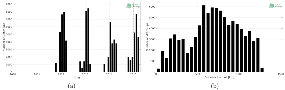
Figure 1: Number of match-ups between TSG-LEGOS-Survostral and Aquarius-L2-JPL-V5 SSS as a function of time (a) and as function of the distance to coast (b) over the Global Ocean Pi-MEP region and for the full satellite product period.
