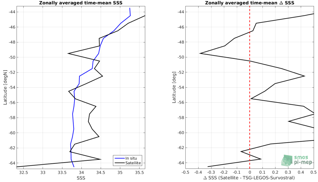
Figure 8: Left panel: Zonal mean SSS from Aquarius-L2-JPL-V5 satellite product (black) and from TSG-LEGOS-Survostral (blue). Right panel: Zonal mean of \Delta SSS (Satellite - TSG-LEGOS-Survostral) for all the collected Pi-MEP match-up pairs estimated over the full satellite product period.
