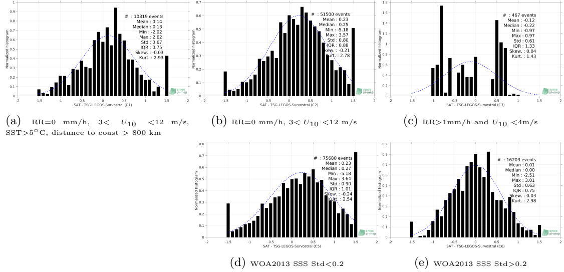
Figure 13: Normalized histogram of \Delta SSS (Aquarius-L2-JPL-V5 - TSG-LEGOS-Survostral) for 5 different subdatasets corresponding to: RR=0 mm/h, 3 < U_{10} < 12 m/s, SST > 5°C, distance to coast > 800 km (a), RR=0 mm/h, 3 < U_{10} < 12 m/s (b), RR > 1mm/h and U_{10} < 4 m/s (c), WOA2013 SSS Std < 0.2 (d), WOA2013 SSS Std > 0.2 (e).
