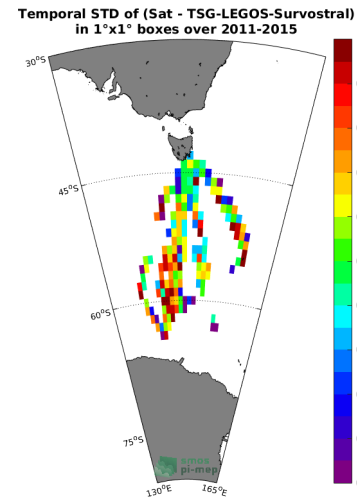
(f) Std( \Delta SSS) (Satellite - TSG-LEGOS-Survostral)
