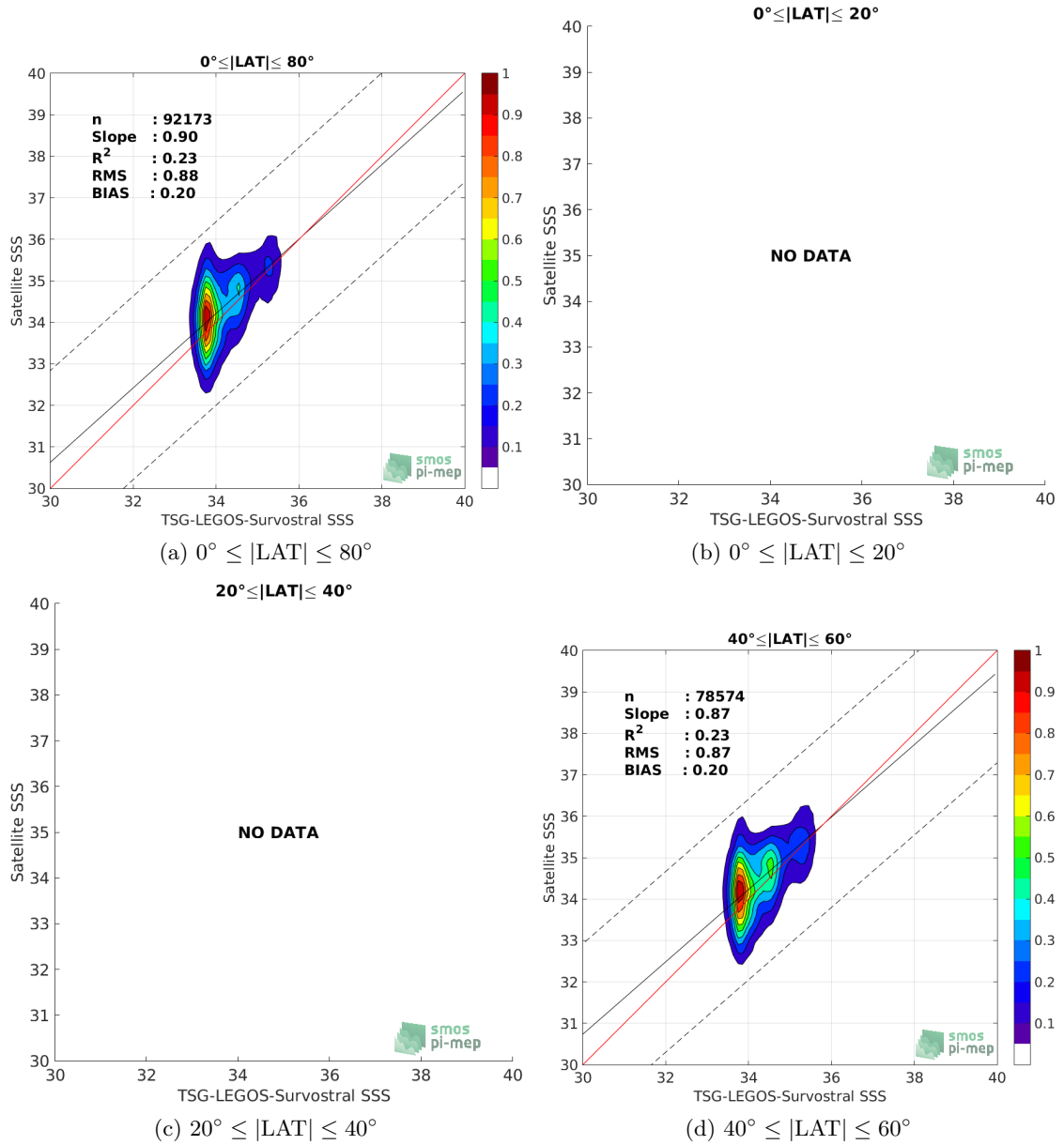
Figure 9: Contour maps of the concentration of Aquarius-L2-JPL-V5 SSS (y-axis) versus TSG-LEGOS-Survostral SSS (x-axis) at match-up pairs for different latitude bands. For each plot, the red line shows x=y . The black thin and dashed lines indicate a linear fit through the data cloud and the \pm 95\% confidence levels, respectively. The number match-up pairs n , the slope and R^2 coefficient of the linear fit, the root mean square (RMS) and the mean bias between satellite and in situ data are indicated for each latitude band in each plots.
