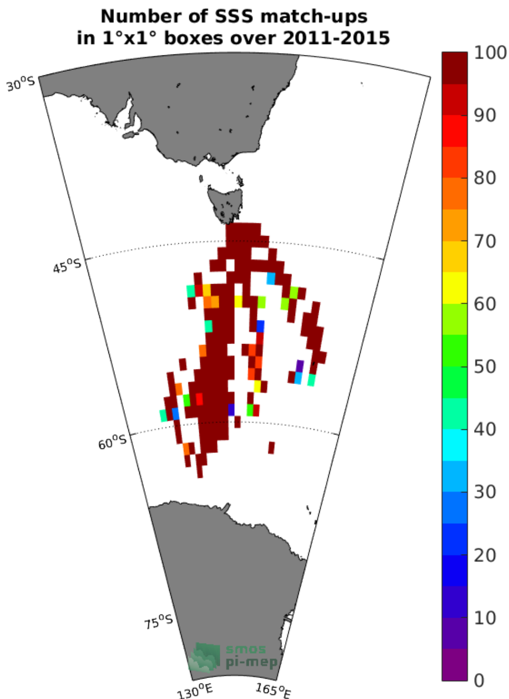
Figure 4: Number of SSS match-ups between TSG-LEGOS-Survostral SSS and the Aquarius-L2-JPL-V5 SSS product for the Global Ocean Pi-MEP region over 1°x1° boxes and for the full satellite product period.
