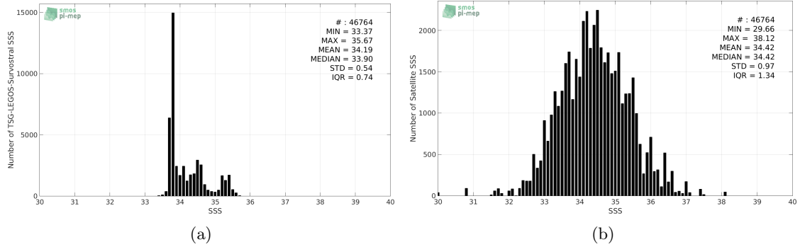
Figure 2: Histograms of SSS from TSG-LEGOS-Survostral (a) and Aquarius-L2-JPL-V5 (b) considering all match-up pairs per bins of 0.1 over the Global Ocean Pi-MEP region and for the full satellite product period.
