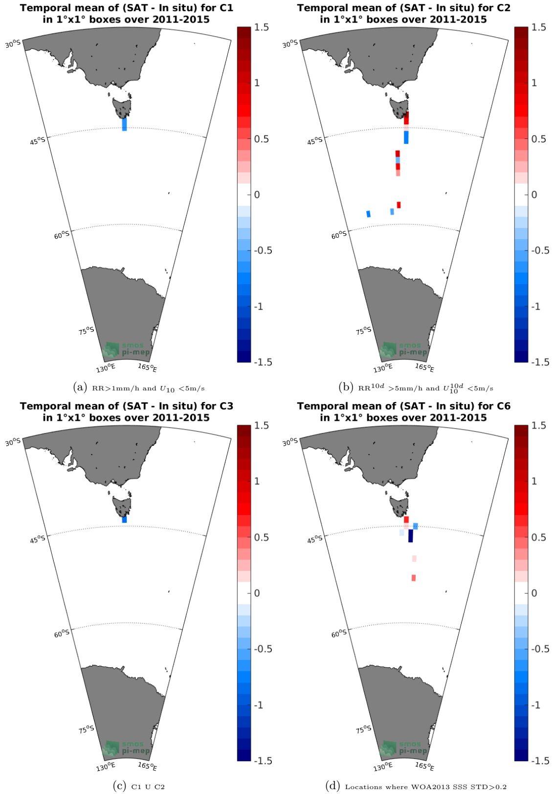
Figure 12: Temporal mean gridded over spatial boxes of size 1°x1° of \Delta\text{SSS} (Aquarius-L2-JPL-V5 - TSG-LEGOS-Survostral) for 4 different subdatasets corresponding to: RR > 1\text{mm/h} and U_{10} < 5\text{m/s} (a), RR^{10d} > 5\text{mm/h} and U_{10}^{10d} < 5\text{m/s} (b), C1 U C2 (c), Locations where WOA2013 SSS STD > 0.2 (d).
