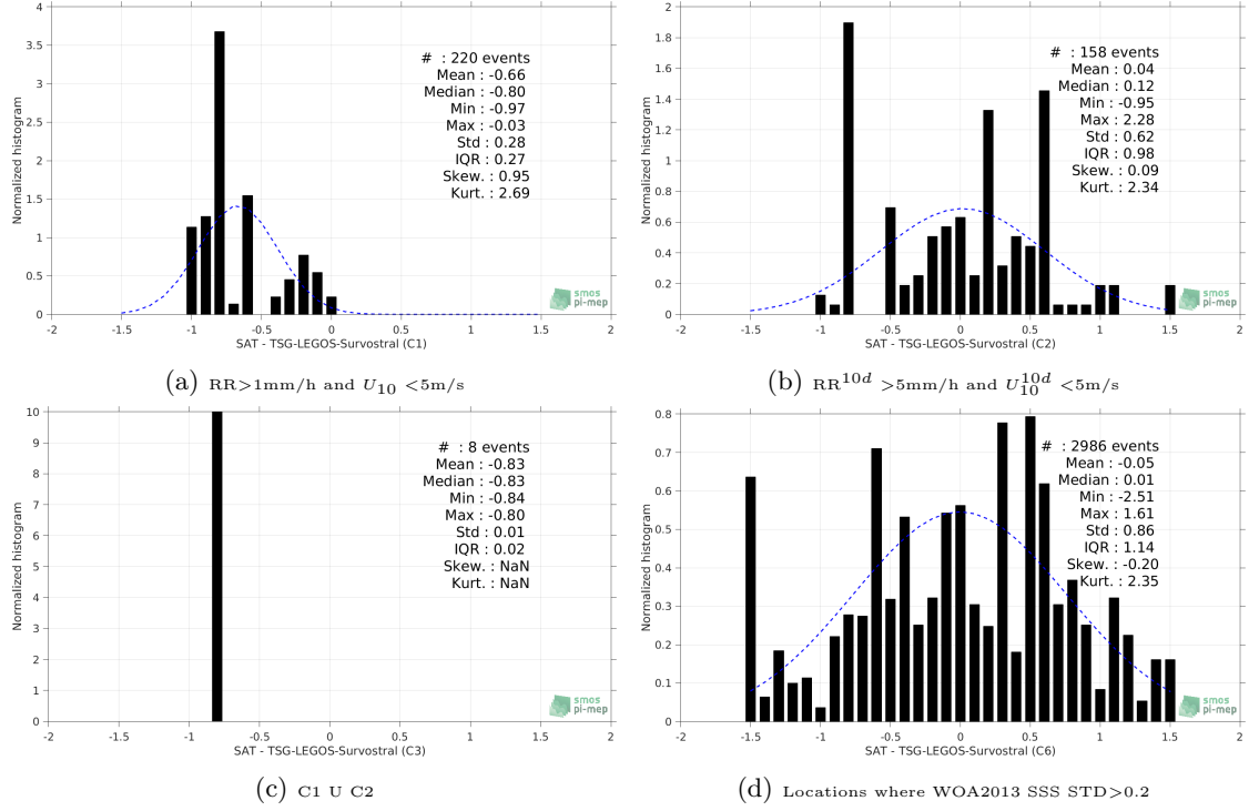
Figure 13: Normalized histogram of \Delta SSS (Aquarius-L2-JPL-V5 - TSG-LEGOS-Survostral) for 6 different subdatasets corresponding to: RR > 1\text{mm/h} and U_{10} < 5\text{m/s} (a), RR^{10d} > 5\text{mm/h} and U_{10}^{10d} < 5\text{m/s} (b), C1 U C2 (c), Locations where WOA2013 SSS STD > 0.2 (d).
