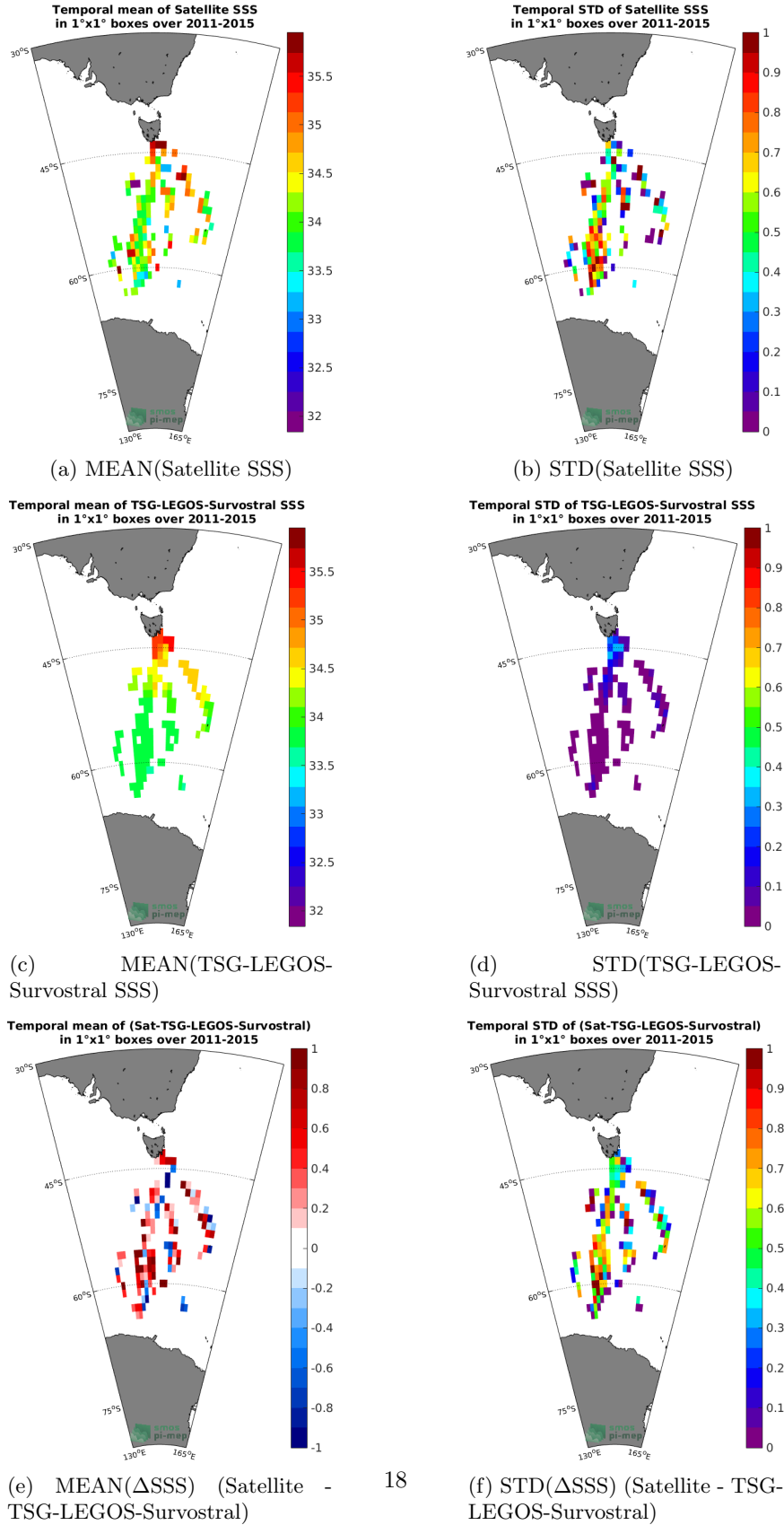
Figure 6: Temporal mean (left) and STD (right) of SSS from Aquarius-L2-JPL-V5 (top), TSG-LEGOS-Survostral (middle), and of \Delta SSS (Satellite - TSG-LEGOS-Survostral). Only match-up pairs are used to generate these maps.
