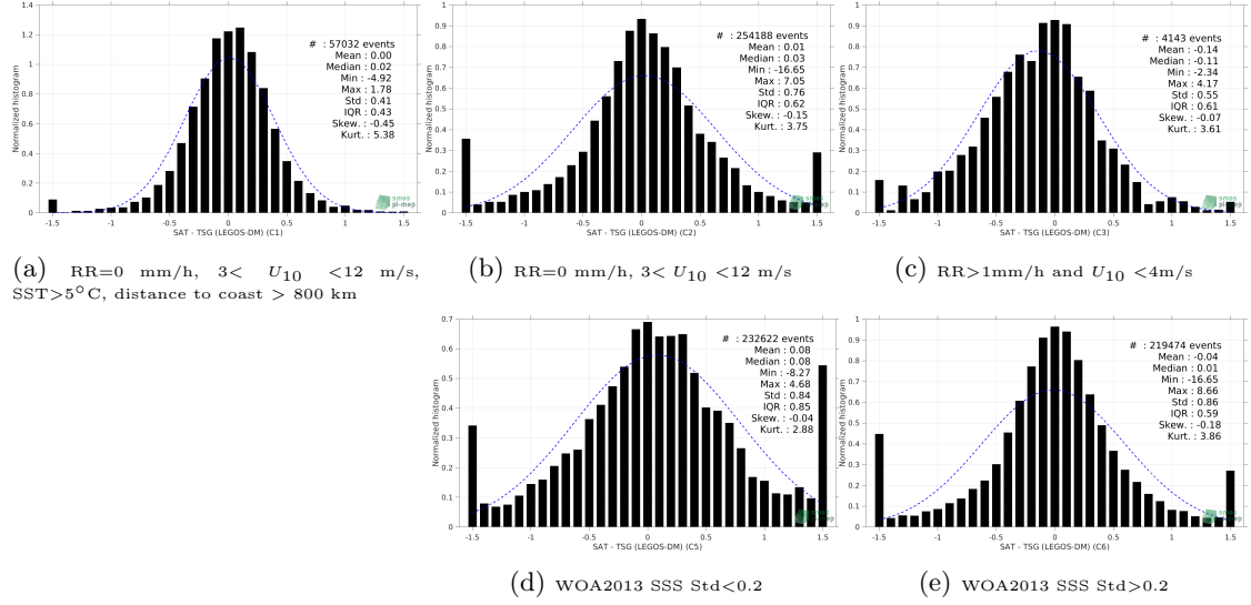
Figure 13: Normalized histogram of \Delta\text{SSS} (Aquarius SSS L2 CAP v5 (JPL) - TSG (LEGOS-DM)) for 5 different subdatasets corresponding to: RR=0 mm/h, 3 < U_{10} < 12 m/s, SST>5°C, distance to coast > 800 km (a), RR=0 mm/h, 3 < U_{10} < 12 m/s (b), RR>1mm/h and U_{10} < 4 m/s (c), WOA2013 SSS Std<0.2 (d), WOA2013 SSS Std>0.2 (e).
