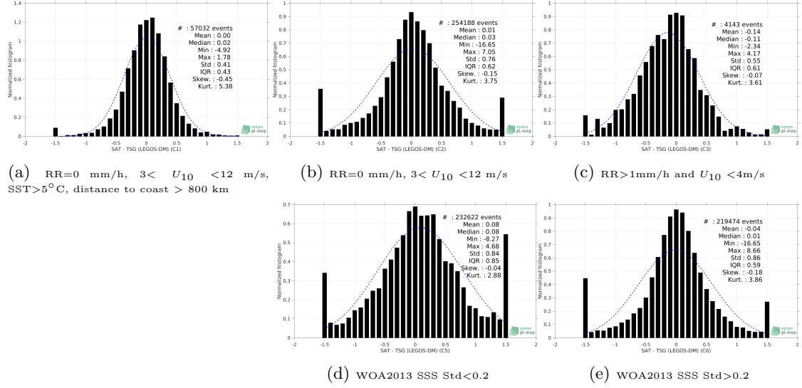
Figure 13: Normalized histogram of \Delta SSS (Aquarius SSS L2 CAP v5 (JPL) - TSG (LEGOS-DM)) for 5 different subdatasets corresponding to: RR=0 mm/h, 3 < U_{10} < 12 m/s, SST > 5^\circ\text{C} , distance to coast > 800 km (a), RR=0 mm/h, 3 < U_{10} < 12 m/s (b), RR > 1 mm/h and U_{10} < 4 m/s (c), WOA2013 SSS Std < 0.2 (d), WOA2013 SSS Std > 0.2 (e).
