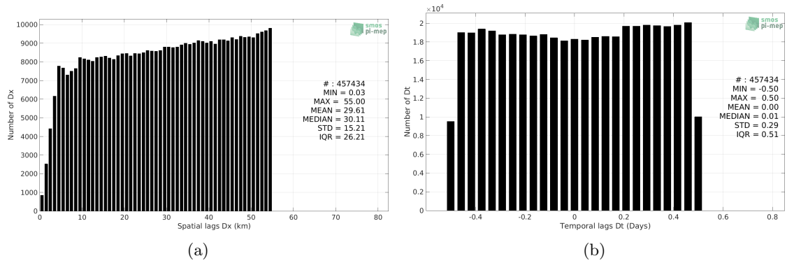
Figure 5: Histograms of the spatial (a) and temporal (b) lags between the time of the TSG (LEGOS-DM) measurements and the date of the corresponding Aquarius SSS L2 CAP v5 (JPL) SSS product.
