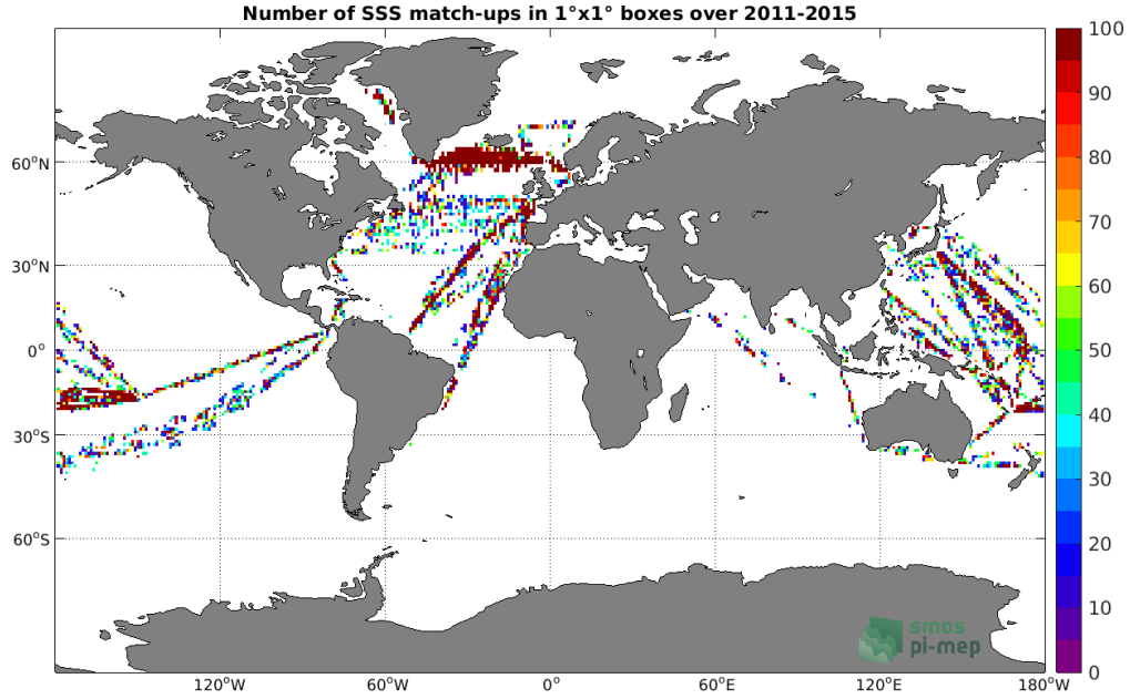
Figure 4: Number of SSS match-ups between TSG (LEGOS-DM) SSS and the Aquarius SSS L2 CAP v5 (JPL) SSS product for the Global Ocean Pi-MEP region over 1^\circ \times 1^\circ boxes and for the full satellite product period.
