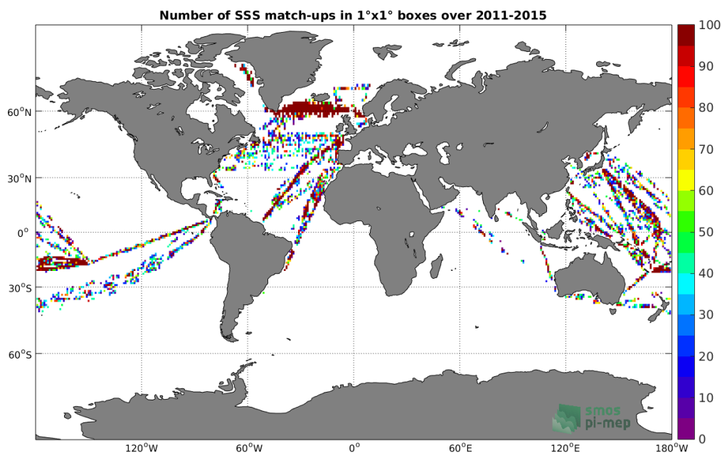
Figure 4: Number of SSS match-ups between TSG-LEGOS-DM SSS and the Aquarius-L2-JPL-V5 SSS product for the Global Ocean Pi-MEP region over 1^\circ \times 1^\circ boxes and for the full satellite product period.
