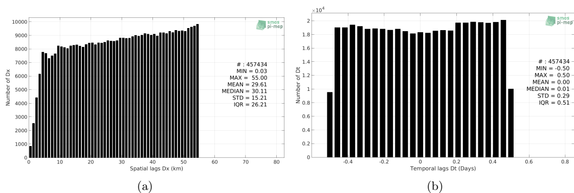
Figure 5: Histograms of the spatial (a) and temporal (b) lags between the time of the TSG-LEGOS-DM measurements and the date of the corresponding Aquarius-L2-JPL-V5 SSS product.
