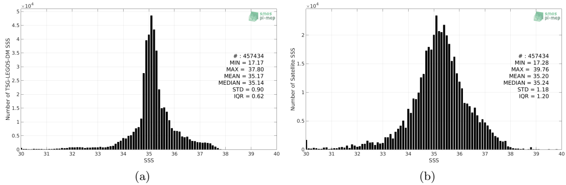
Figure 2: Histograms of SSS from TSG-LEGOS-DM (a) and Aquarius-L2-JPL-V5 (b) considering all match-up pairs per bins of 0.1 over the Global Ocean Pi-MEP region and for the full satellite product period.
