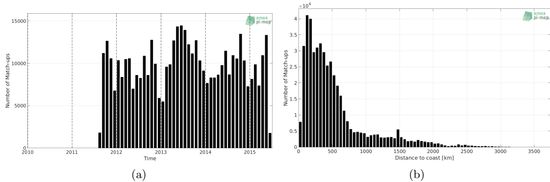
Figure 1: Number of match-ups between TSG-LEGOS-DM and Aquarius-L2-JPL-V5 SSS as a function of time (a) and as function of the distance to coast (b) over the Global Ocean Pi-MEP region and for the full satellite product period.
