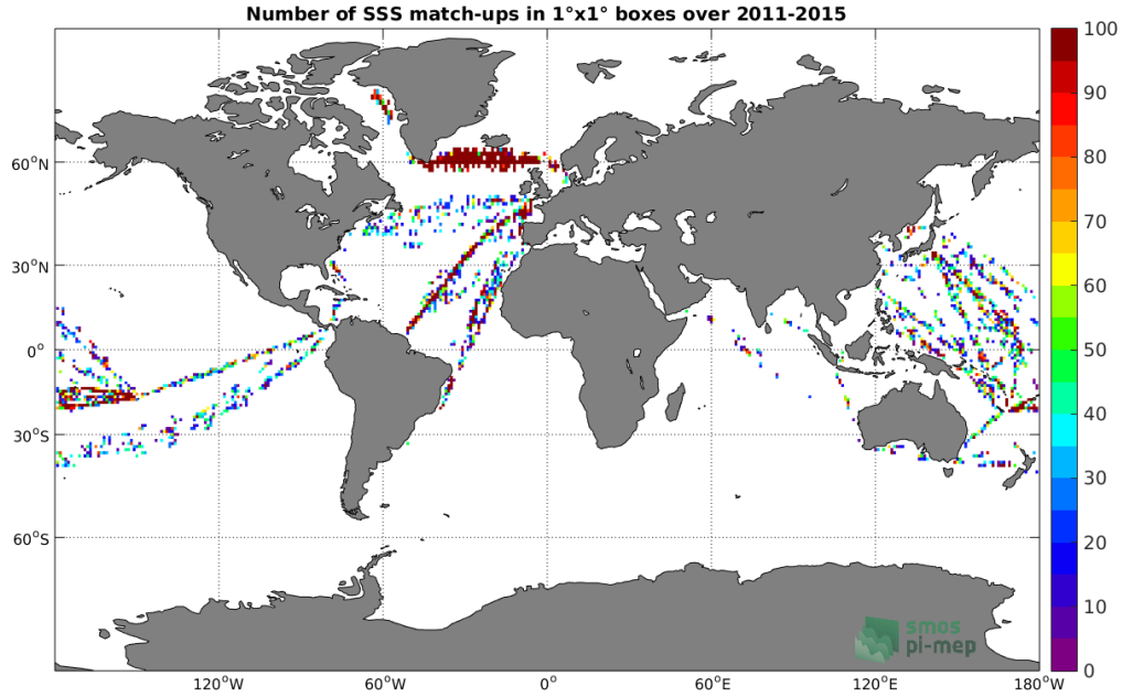
Figure 4: Number of SSS match-ups between TSG-LEGOS-DM SSS and the Aquarius-L2-JPL-V5 SSS product for the Global Ocean Pi-MEP region over 1°x1° boxes and for the full satellite product period.
