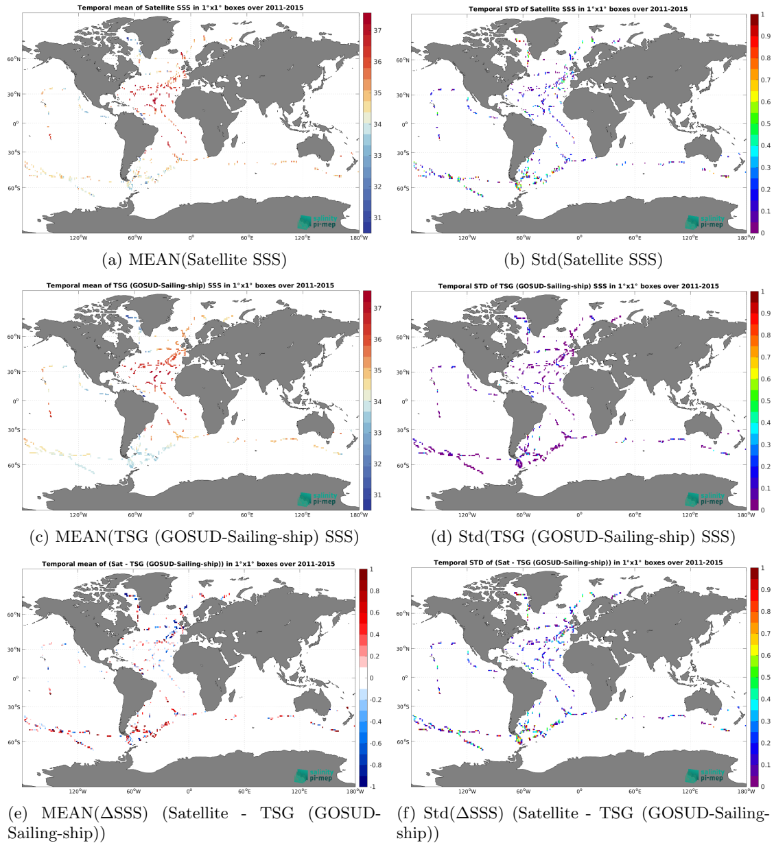
Figure 7: Temporal mean (left) and Std (right) of SSS from Aquarius SSS L2 CAP v5 (JPL) (top), TSG (GOSUD-Sailing-ship) (middle), and of \Delta SSS (Satellite - TSG (GOSUD-Sailing-ship)). Only match-up pairs are used to generate these maps.
