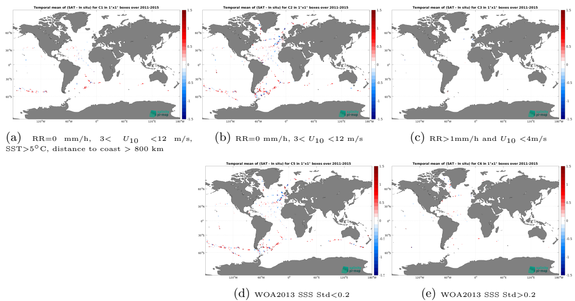
Figure 14: Temporal mean gridded over spatial boxes of size 1^\circ \times 1^\circ of \Delta SSS (Aquarius SSS L2 CAP v5 (JPL) - TSG (GOSUD-Sailing-ship)) for 5 different subdatasets corresponding to: RR=0 mm/h, 3 < U_{10} < 12 m/s, SST > 5°C, distance to coast > 800 km (a), RR=0 mm/h, 3 < U_{10} < 12 m/s (b), RR > 1mm/h and U_{10} < 4 m/s (c), WOA2013 SSS Std < 0.2 (d), WOA2013 SSS Std > 0.2 (e).
