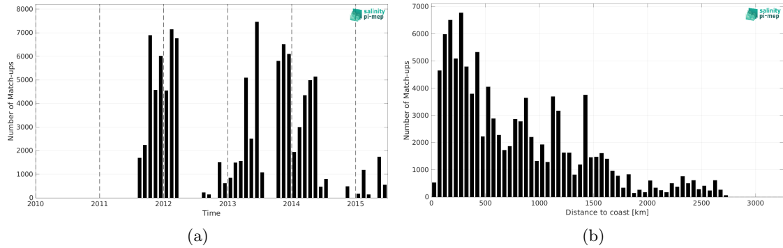
Figure 2: Number of match-ups between TSG (GOSUD-Sailing-ship) and Aquarius SSS L2 CAP v5 (JPL) SSS as a function of time (a) and as function of the distance to coast (b) over the Global Ocean Pi-MEP region and for the full satellite product period.
