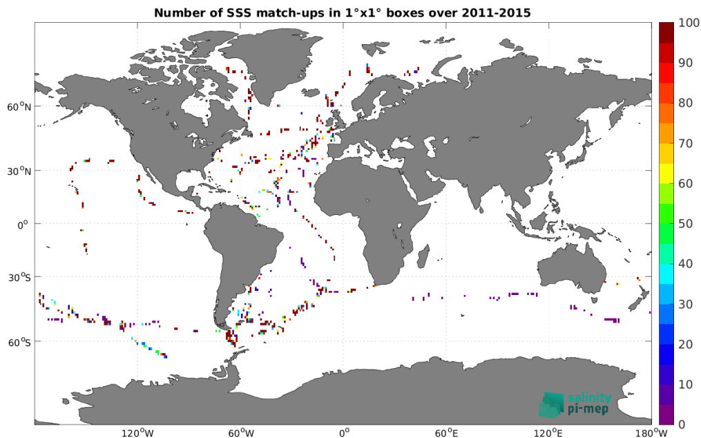
Figure 5: Number of SSS match-ups between TSG (GOSUD-Sailing-ship) SSS and the Aquarius SSS L2 CAP v5 (JPL) SSS product for the Global Ocean Pi-MEP region over 1^\circ \times 1^\circ boxes and for the full satellite product period.
