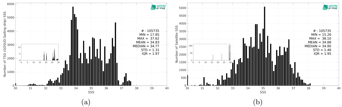
Figure 3: Histograms of SSS from TSG (GOSUD-Sailing-ship) (a) and Aquarius SSS L2 CAP v5 (JPL) (b) considering all match-up pairs per bins of 0.1 over the Global Ocean Pi-MEP region and for the full satellite product period.
