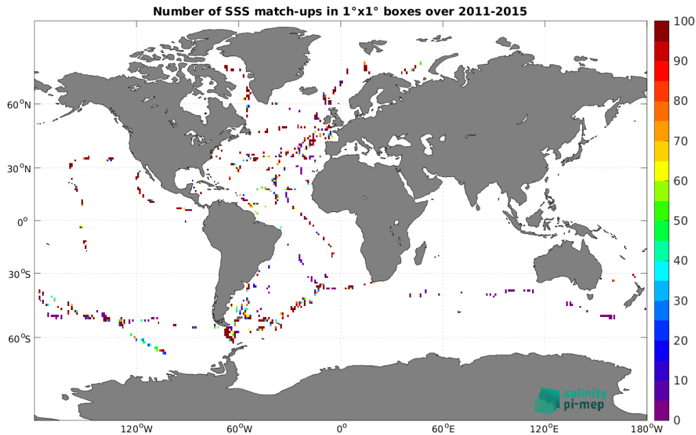
Figure 4: Number of SSS match-ups between TSG (GOSUD-Sailing-ship) SSS and the Aquarius SSS L2 CAP v5 (JPL) SSS product for the Global Ocean Pi-MEP region over 1^\circ \times 1^\circ boxes and for the full satellite product period.
