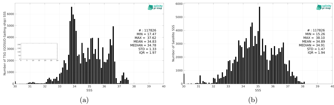
Figure 2: Histograms of SSS from TSG (GOSUD-Sailing-ship) (a) and Aquarius SSS L2 CAP v5 (JPL) (b) considering all match-up pairs per bins of 0.1 over the Global Ocean Pi-MEP region and for the full satellite product period.
