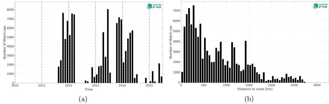
Figure 1: Number of match-ups between TSG (GOSUD-Sailing-ship) and Aquarius SSS L2 CAP v5 (JPL) SSS as a function of time (a) and as function of the distance to coast (b) over the Global Ocean Pi-MEP region and for the full satellite product period.
