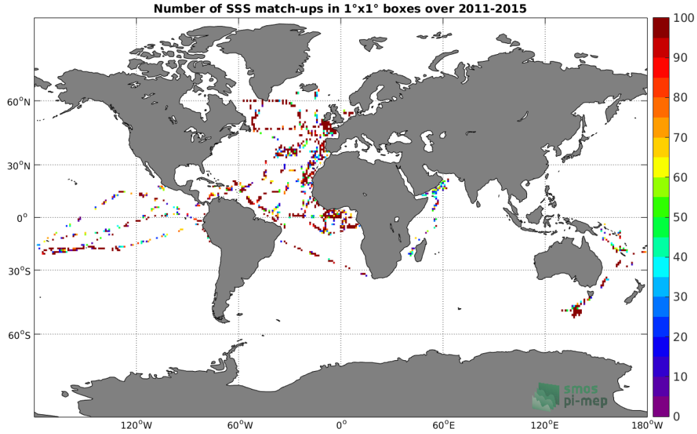
Figure 4: Number of SSS match-ups between TSG-GOSUD-Research-vessel SSS and the Aquarius-L2-JPL-V5 SSS product for the Global Ocean Pi-MEP region over 1^\circ \times 1^\circ boxes and for the full satellite product period.
