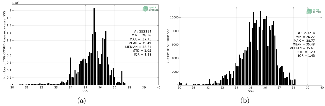
Figure 2: Histograms of SSS from TSG-GOSUD-Research-vessel (a) and Aquarius-L2-JPL-V5 (b) considering all match-up pairs per bins of 0.1 over the Global Ocean Pi-MEP region and for the full satellite product period.
