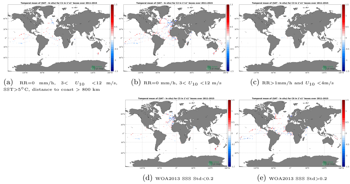
Figure 12: Temporal mean gridded over spatial boxes of size 1^\circ \times 1^\circ of \Delta SSS (Aquarius-L2-JPL-V5 - TSG-GOSUD-Research-vessel) for 5 different subdatasets corresponding to: RR=0 mm/h, 3 < U_{10} < 12 m/s, SST > 5^\circ\text{C} , distance to coast > 800 km (a), RR=0 mm/h, 3 < U_{10} < 12 m/s (b), RR > 1 mm/h and U_{10} < 4 m/s (c), WOA2013 SSS Std < 0.2 (d), WOA2013 SSS Std > 0.2 (e).
