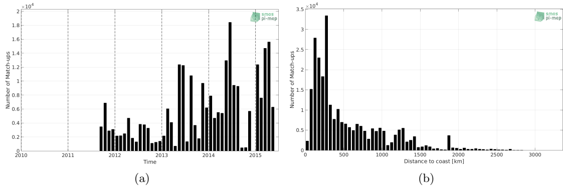
Figure 1: Number of match-ups between TSG-GOSUD-Research-vessel and Aquarius-L2-JPL-V5 SSS as a function of time (a) and as function of the distance to coast (b) over the Global Ocean Pi-MEP region and for the full satellite product period.
