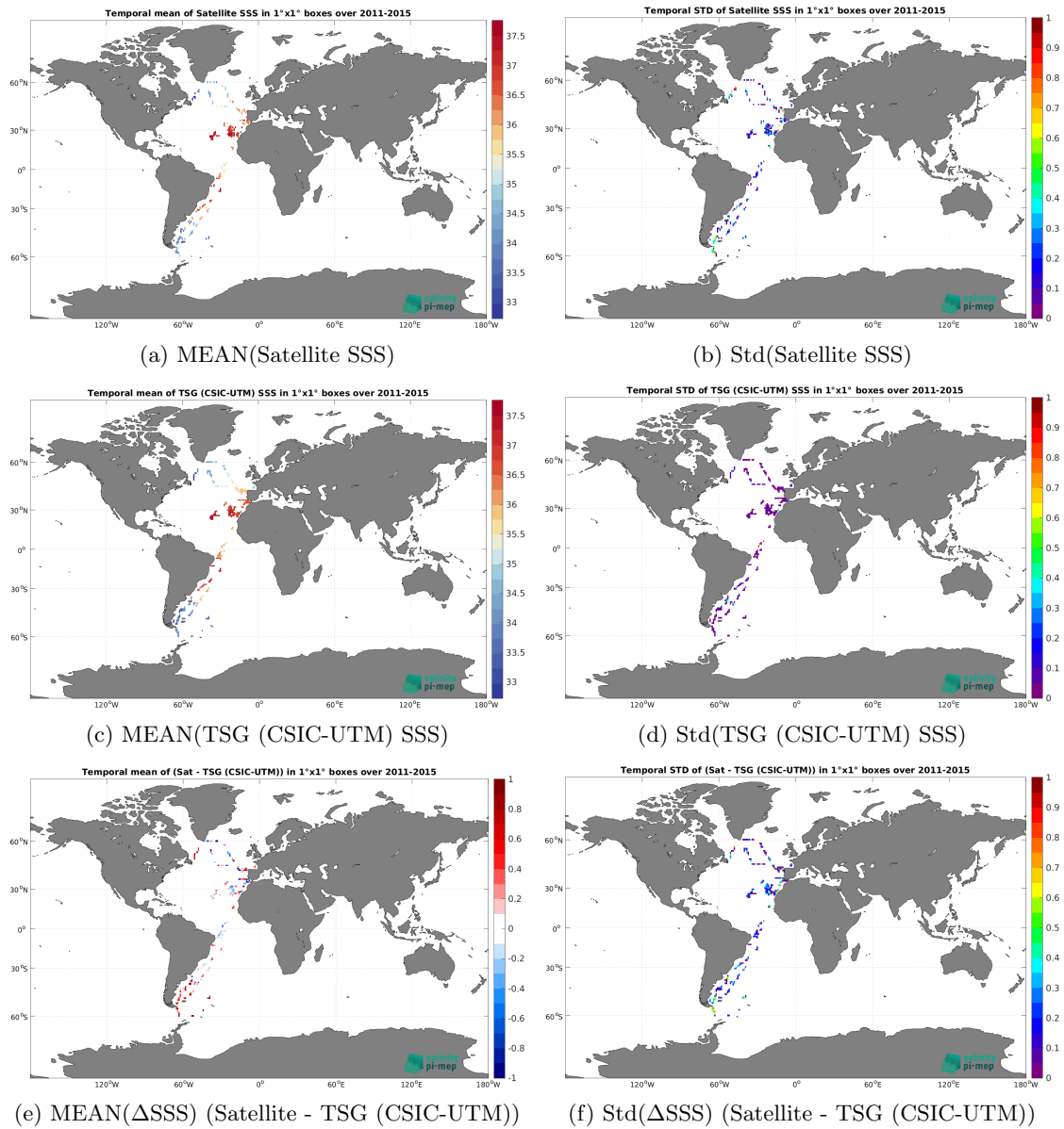
Figure 7: Temporal mean (left) and Std (right) of SSS from Aquarius SSS L2 CAP v5 (JPL) (top), TSG (CSIC-UTM) (middle), and of \Delta SSS (Satellite - TSG (CSIC-UTM)). Only match-up pairs are used to generate these maps.
