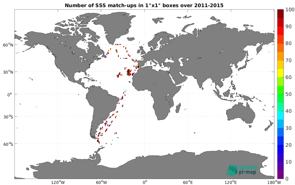
Figure 5: Number of SSS match-ups between TSG (CSIC-UTM) SSS and the Aquarius SSS L2 CAP v5 (JPL) SSS product for the Global Ocean Pi-MEP region over 1^\circ \times 1^\circ boxes and for the full satellite product period.
