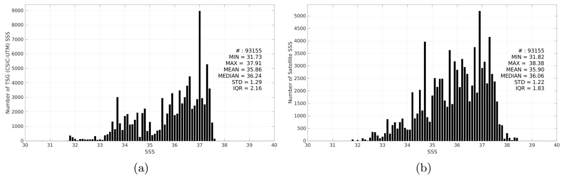
Figure 3: Histograms of SSS from TSG (CSIC-UTM) (a) and Aquarius SSS L2 CAP v5 (JPL) (b) considering all match-up pairs per bins of 0.1 over the Global Ocean Pi-MEP region and for the full satellite product period.
