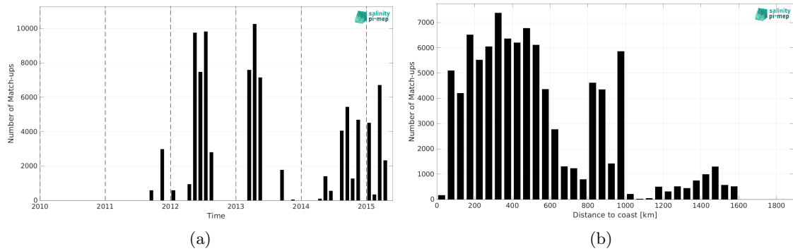
Figure 2: Number of match-ups between TSG (CSIC-UTM) and Aquarius SSS L2 CAP v5 (JPL) SSS as a function of time (a) and as function of the distance to coast (b) over the Global Ocean Pi-MEP region and for the full satellite product period.
