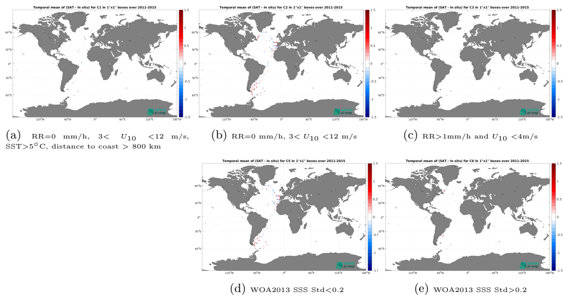
Figure 14: Temporal mean gridded over spatial boxes of size 1^\circ \times 1^\circ of \Delta SSS (Aquarius SSS L2 CAP v5 (JPL) - TSG (CSIC-UTM)) for 5 different subdatasets corresponding to:RR=0 mm/h, 3 < U_{10} < 12 m/s, SST > 5^\circ\text{C} , distance to coast > 800 km (a), RR=0 mm/h, 3 < U_{10} < 12 m/s (b), RR > 1 mm/h and U_{10} < 4 m/s (c), WOA2013 SSS Std < 0.2 (d), WOA2013 SSS Std > 0.2 (e).
