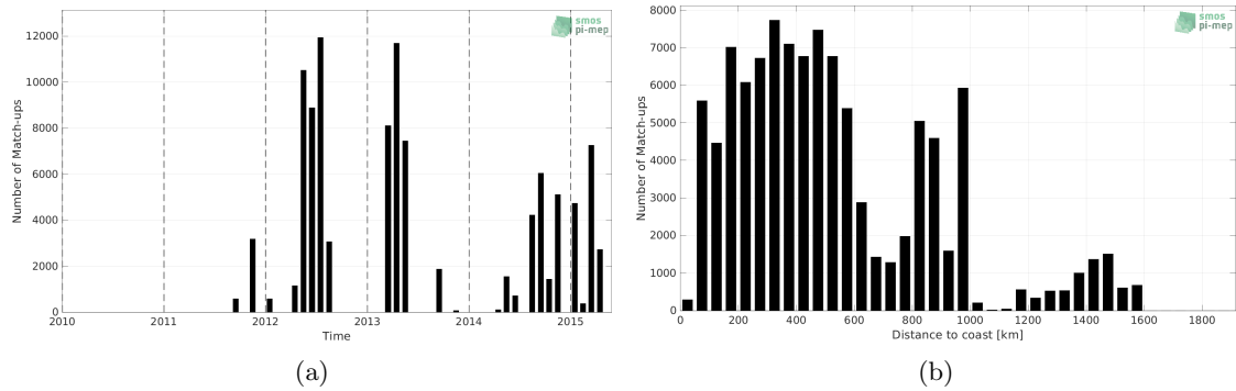
Figure 1: Number of match-ups between TSG (CSIC-UTM) and Aquarius SSS L2 CAP v5 (JPL) SSS as a function of time (a) and as function of the distance to coast (b) over the Global Ocean Pi-MEP region and for the full satellite product period.
