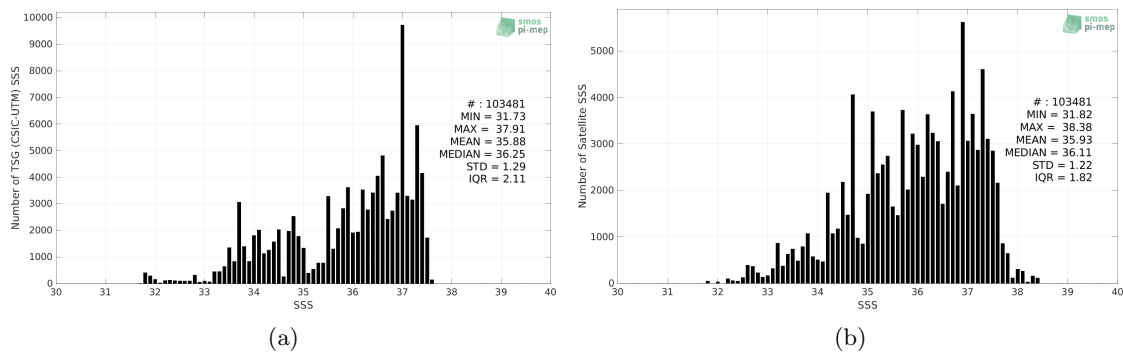
Figure 2: Histograms of SSS from TSG (CSIC-UTM) (a) and Aquarius SSS L2 CAP v5 (JPL) (b) considering all match-up pairs per bins of 0.1 over the Global Ocean Pi-MEP region and for the full satellite product period.
