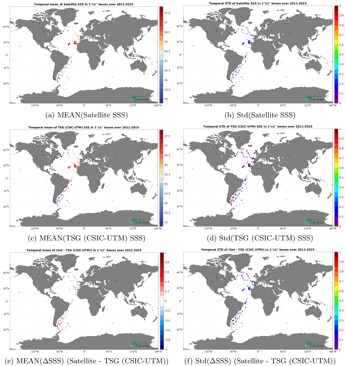
Figure 6: Temporal mean (left) and Std (right) of SSS from Aquarius SSS L2 CAP v5 (JPL) (top), TSG (CSIC-UTM) (middle), and of \Delta SSS (Satellite - TSG (CSIC-UTM)). Only match-up pairs are used to generate these maps.
