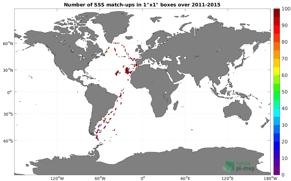
Figure 4: Number of SSS match-ups between TSG (CSIC-UTM) SSS and the Aquarius SSS L2 CAP v5 (JPL) SSS product for the Global Ocean Pi-MEP region over 1^\circ \times 1^\circ boxes and for the full satellite product period.
