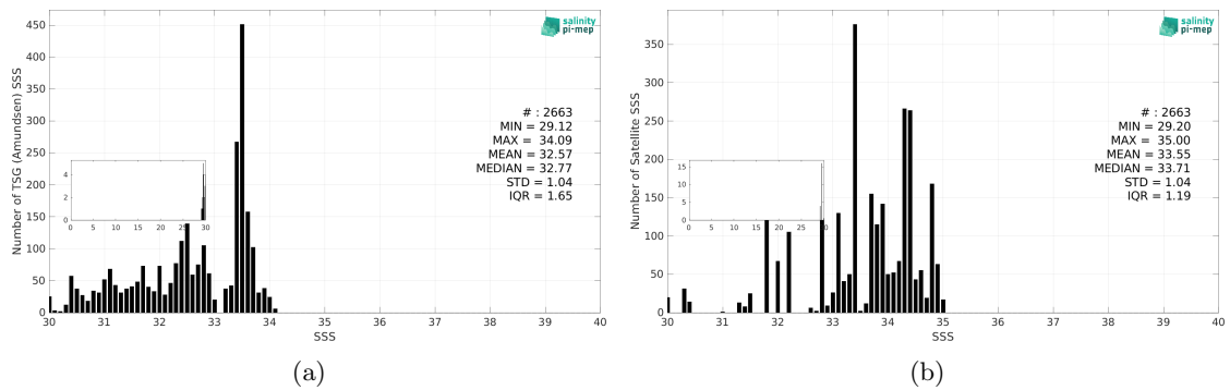
Figure 3: Histograms of SSS from TSG (Amundsen) (a) and Aquarius SSS L2 CAP v5 (JPL) (b) considering all match-up pairs per bins of 0.1 over the Global Ocean Pi-MEP region and for the full satellite product period.
