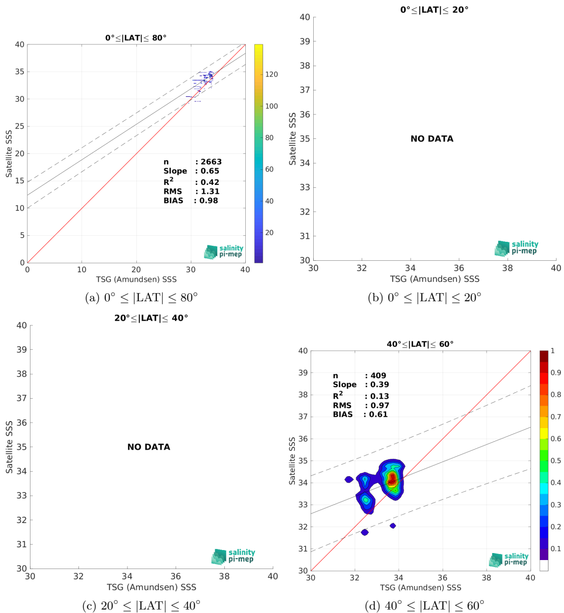
Figure 10: Contour maps of the concentration of Aquarius SSS L2 CAP v5 (JPL) SSS (y-axis) versus TSG (Amundsen) SSS (x-axis) at match-up pairs for different latitude bands. For each plot, the red line shows x=y . The black thin and dashed lines indicate a linear fit through the data cloud and the \pm 95\% confidence levels, respectively. The number match-up pairs n , the slope and R^2 coefficient of the linear fit, the root mean square (RMS) and the mean bias between satellite and in situ data are indicated for each latitude band in each plots.
