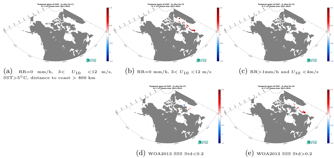
Figure 14: Temporal mean gridded over spatial boxes of size 1^\circ \times 1^\circ of \Delta SSS (Aquarius SSS L2 CAP v5 (JPL) - TSG (Amundsen)) for 5 different subdatasets corresponding to: RR=0 mm/h, 3 < U_{10} < 12 m/s, SST > 5°C, distance to coast > 800 km (a), RR=0 mm/h, 3 < U_{10} < 12 m/s (b), RR > 1mm/h and U_{10} < 4 m/s (c), WOA2013 SSS Std < 0.2 (d), WOA2013 SSS Std > 0.2 (e).
