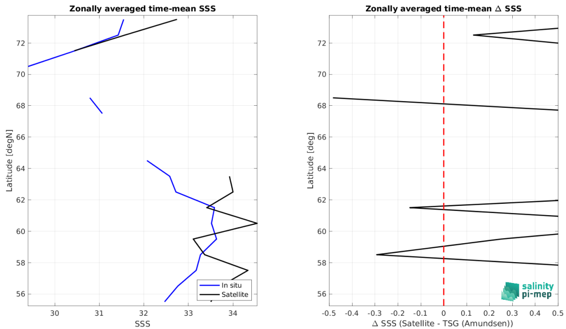
Figure 9: Left panel: Zonal mean SSS from Aquarius SSS L2 CAP v5 (JPL) satellite product (black) and from TSG (Amundsen) (blue). Right panel: Zonal mean of \Delta SSS (Satellite - TSG (Amundsen)) for all the collected Pi-MEP match-up pairs estimated over the full satellite product period.
