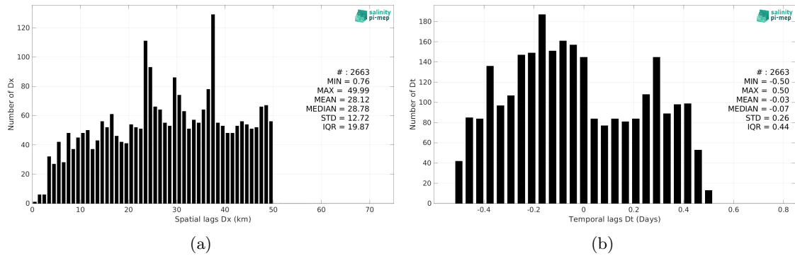
Figure 6: Histograms of the spatial (a) and temporal (b) lags between the location/time of the TSG (Amundsen) measurement and the date of the corresponding Aquarius SSS L2 CAP v5 (JPL) SSS pixel.
