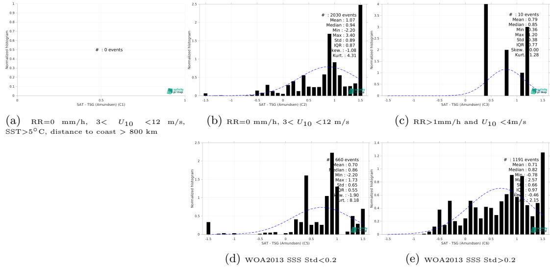
Figure 15: Normalized histogram of \Delta SSS (Aquarius SSS L2 CAP v5 (JPL) - TSG (Amundsen)) for 5 different subdatasets corresponding to: RR=0 mm/h, 3 < U_{10} < 12 m/s, SST > 5°C, distance to coast > 800 km (a), RR=0 mm/h, 3 < U_{10} < 12 m/s (b), RR > 1mm/h and U_{10} < 4 m/s (c), WOA2013 SSS Std < 0.2 (d), WOA2013 SSS Std > 0.2 (e).
