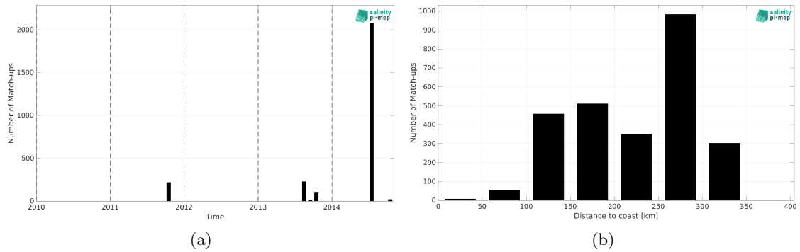
Figure 2: Number of match-ups between TSG (Amundsen) and Aquarius SSS L2 CAP v5 (JPL) SSS as a function of time (a) and as function of the distance to coast (b) over the Global Ocean Pi-MEP region and for the full satellite product period.
