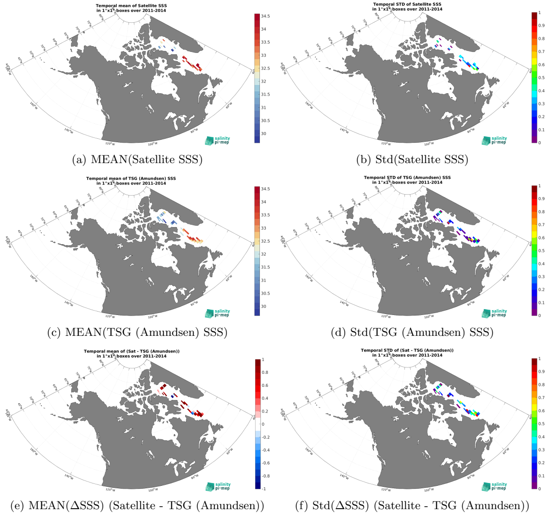
Figure 7: Temporal mean (left) and Std (right) of SSS from Aquarius SSS L2 CAP v5 (JPL) (top), TSG (Amundsen) (middle), and of \Delta SSS (Satellite - TSG (Amundsen)). Only match-up pairs are used to generate these maps.
