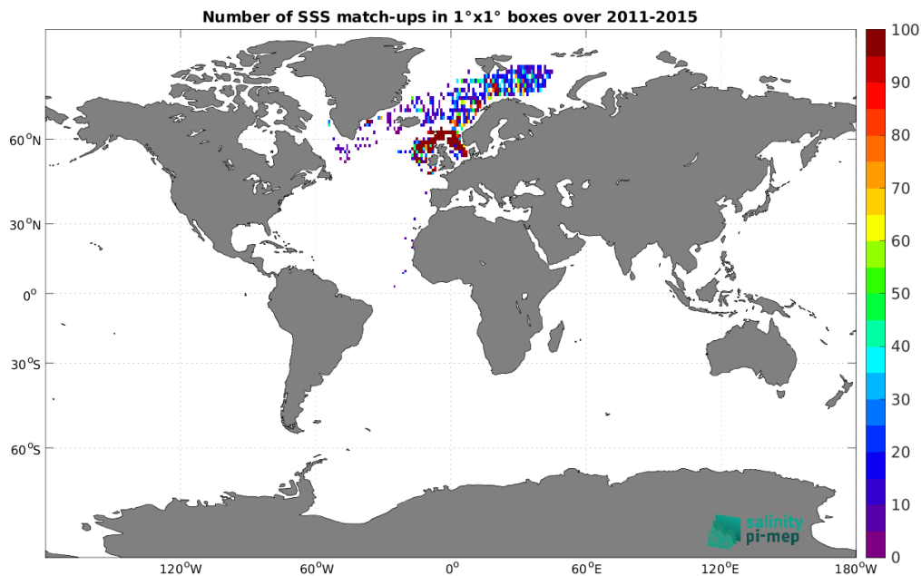
Figure 5: Number of SSS match-ups between ICES SSS and the Aquarius SSS L2 CAP v5 (JPL) SSS product for the Global Ocean Pi-MEP region over 1^\circ \times 1^\circ boxes and for the full satellite product period.
