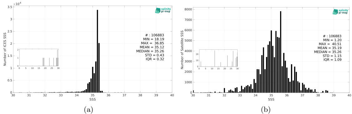
Figure 3: Histograms of SSS from ICES (a) and Aquarius SSS L2 CAP v5 (JPL) (b) considering all match-up pairs per bins of 0.1 over the Global Ocean Pi-MEP region and for the full satellite product period.
