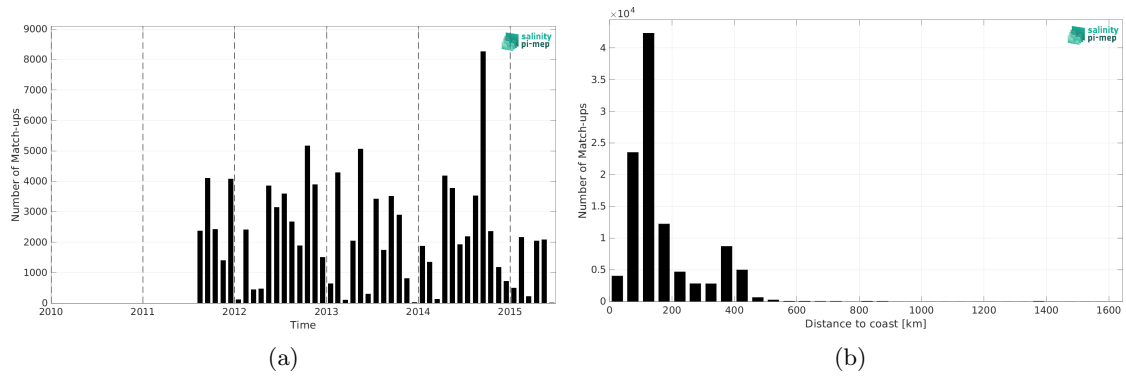
Figure 2: Number of match-ups between ICES and Aquarius SSS L2 CAP v5 (JPL) SSS as a function of time (a) and as function of the distance to coast (b) over the Global Ocean Pi-MEP region and for the full satellite product period.
