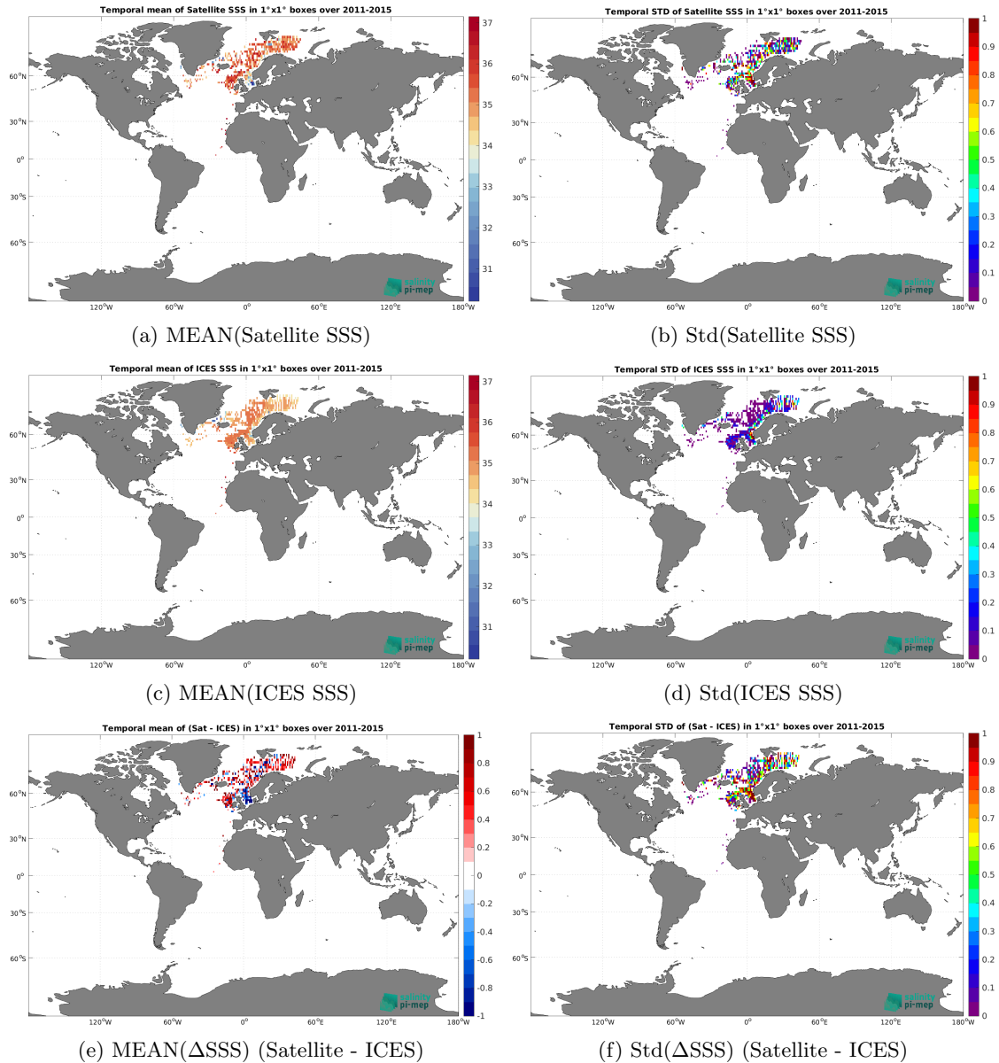
Figure 7: Temporal mean (left) and Std (right) of SSS from Aquarius SSS L2 CAP v5 (JPL) (top), ICES (middle), and of \Delta SSS (Satellite - ICES). Only match-up pairs are used to generate these maps.
