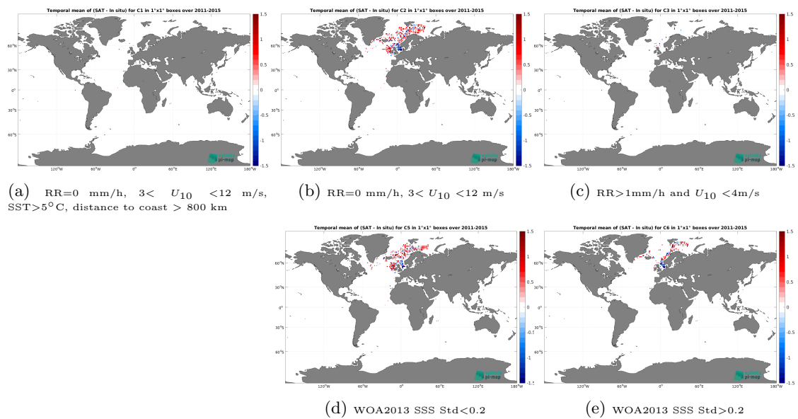
Figure 14: Temporal mean gridded over spatial boxes of size 1^\circ \times 1^\circ of \Delta SSS (Aquarius SSS L2 CAP v5 (JPL) - ICES) for 5 different subdatasets corresponding to:RR=0 mm/h, 3 < U_{10} < 12 m/s, SST > 5^\circ\text{C} , distance to coast > 800 km (a), RR=0 mm/h, 3 < U_{10} < 12 m/s (b), RR > 1 mm/h and U_{10} < 4 m/s (c), WOA2013 SSS Std < 0.2 (d), WOA2013 SSS Std > 0.2 (e).
