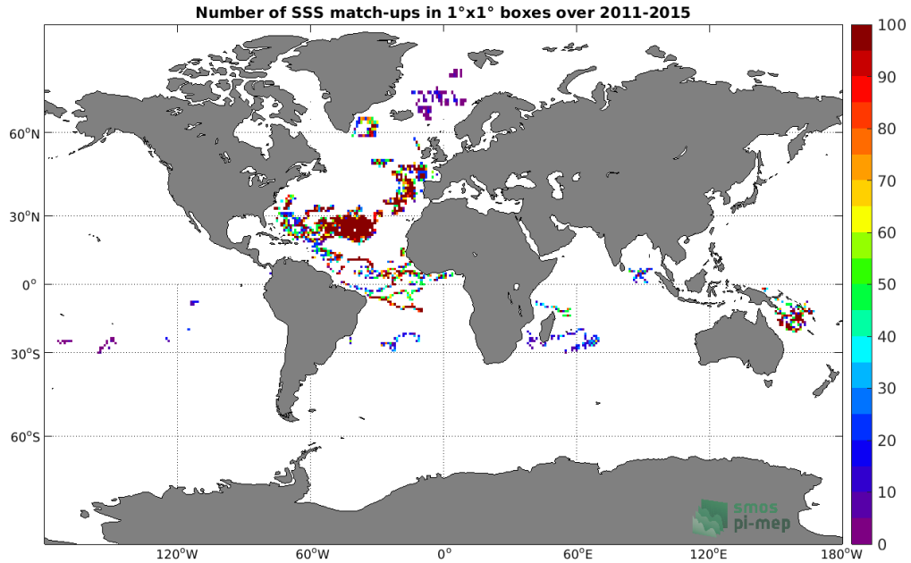
Figure 3: Number of SSS match-ups between Surface drifters SSS and the Aquarius SSS L2 CAP v5 (JPL) SSS product for the Global Ocean Pi-MEP region over 1°x1° boxes and for the full satellite product period.
