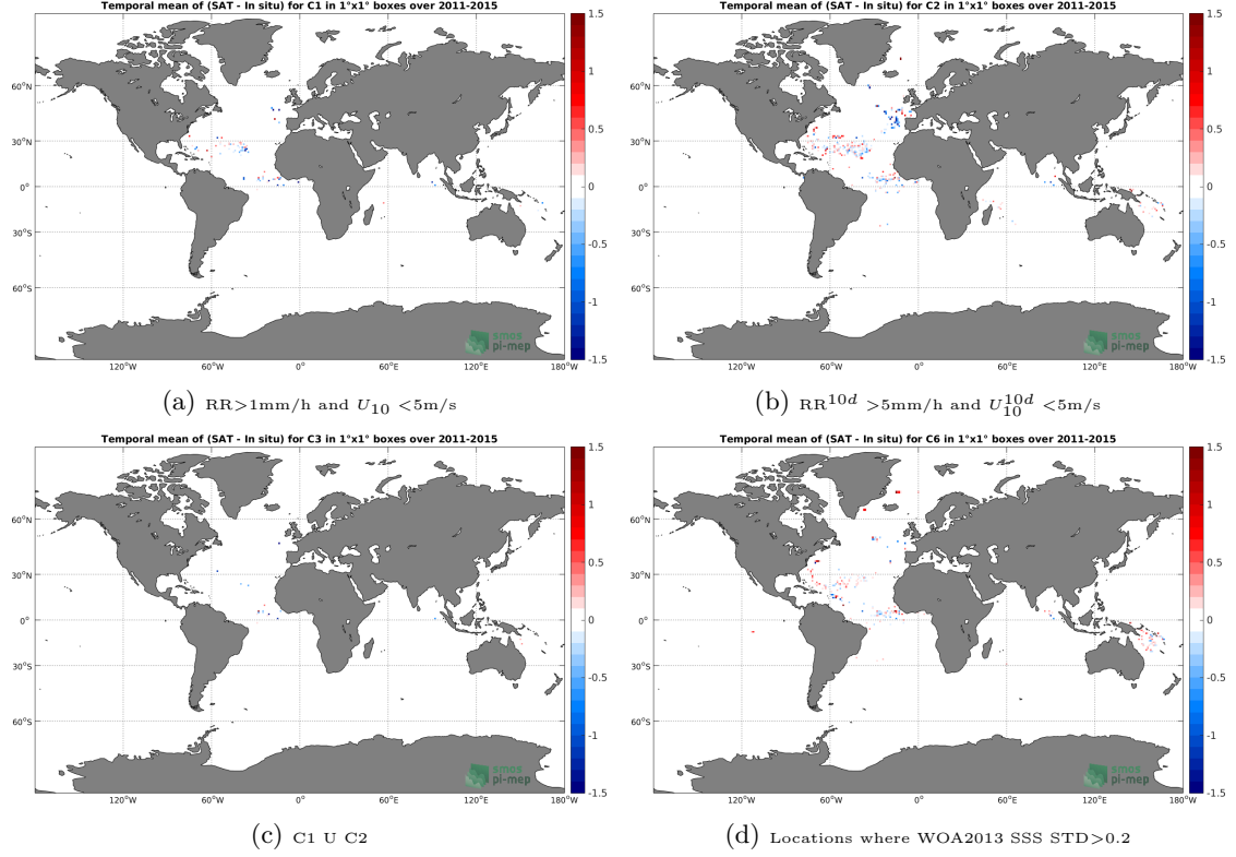
Figure 11: Temporal mean gridded over spatial boxes of size 1^\circ \times 1^\circ of \Delta SSS (Aquarius-L2-JPL-V5 - Surface drifters) for 4 different subdatasets corresponding to: RR > 1\text{mm/h} and U_{10} < 5\text{m/s} (a), RR^{10d} > 5\text{mm/h} and U_{10}^{10d} < 5\text{m/s} (b), C1 U C2 (c), Locations where WOA2013 SSS STD > 0.2 (d).
