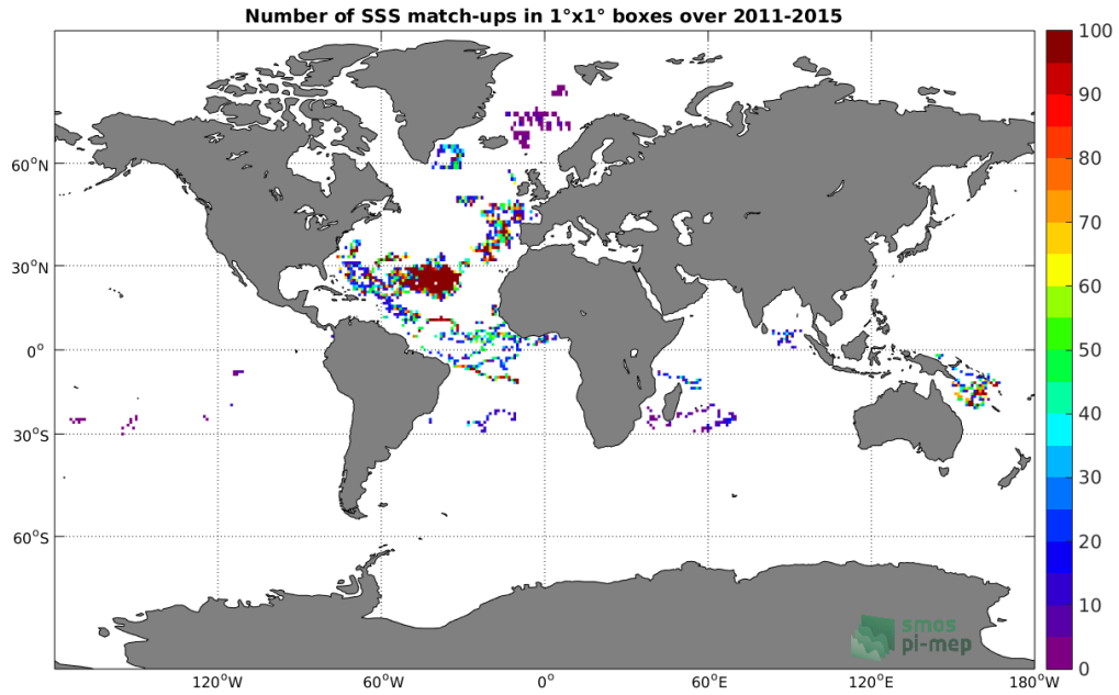
Figure 3: Number of SSS match-ups between Surface drifters SSS and the Aquarius-L2-JPL-V5 SSS product for the Global Ocean Pi-MEP region over 1°x1° boxes and for the full satellite product period.
