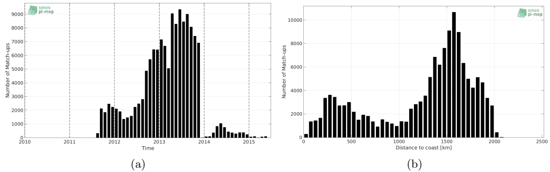
Figure 1: Number of match-ups between Surface drifters and Aquarius-L2-JPL-V5 SSS as a function of time (a) and as function of the distance to coast (b) over the Global Ocean Pi-MEP region and for the full satellite product period.
