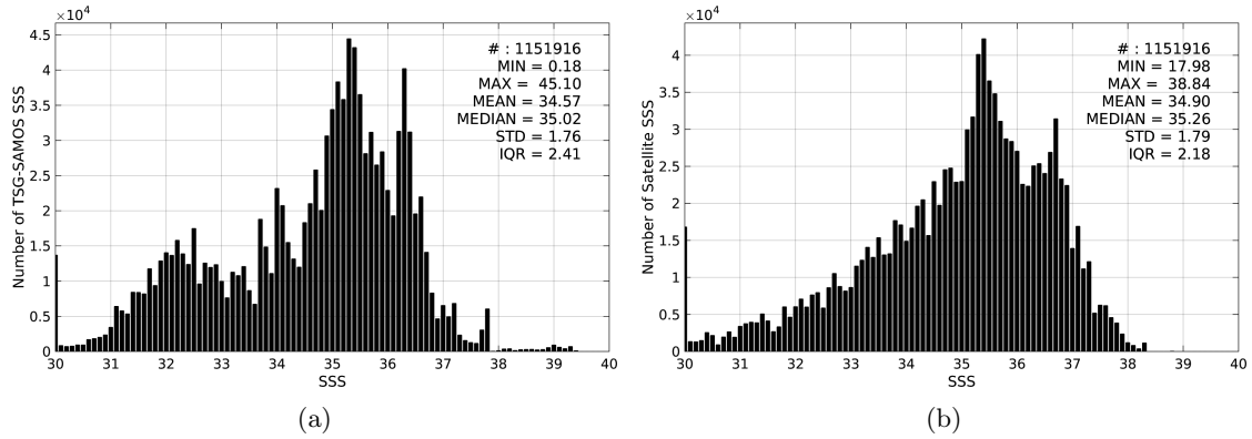
Figure 2: Histograms of SSS from TSG-SAMOS (a) and AQUARIUS-L2-JPL-V4 (b) considering all match-up pairs per bins of 0.1 over the Global Ocean Pi-MEP region and for the full satellite product period.
