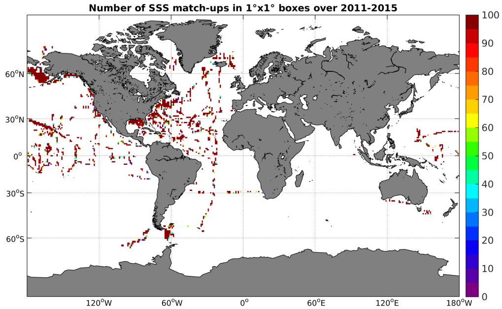
Figure 4: Number of SSS match-ups between TSG-SAMOS SSS and the AQUARIUS-L2-JPL-V4 SSS product for the Global Ocean Pi-MEP region over 1^\circ \times 1^\circ boxes and for the full satellite product period.
