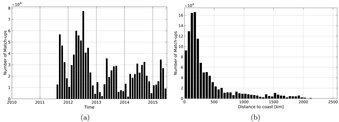
Figure 1: Number of match-ups between TSG-SAMOS and AQUARIUS-L2-JPL-V4 SSS as a function of time (a) and as function of the distance to coast (b) over the Global Ocean Pi-MEP region and for the full satellite product period.
