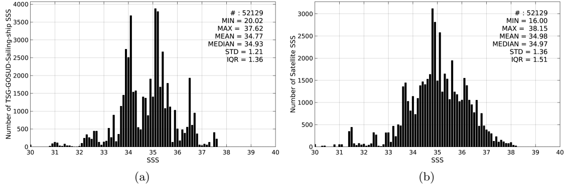
Figure 2: Histograms of SSS from TSG-GOSUD-Sailing-ship (a) and AQUARIUS-L2-JPL-V4 (b) considering all match-up pairs per bins of 0.1 over the Global Ocean Pi-MEP region and for the full satellite product period.
