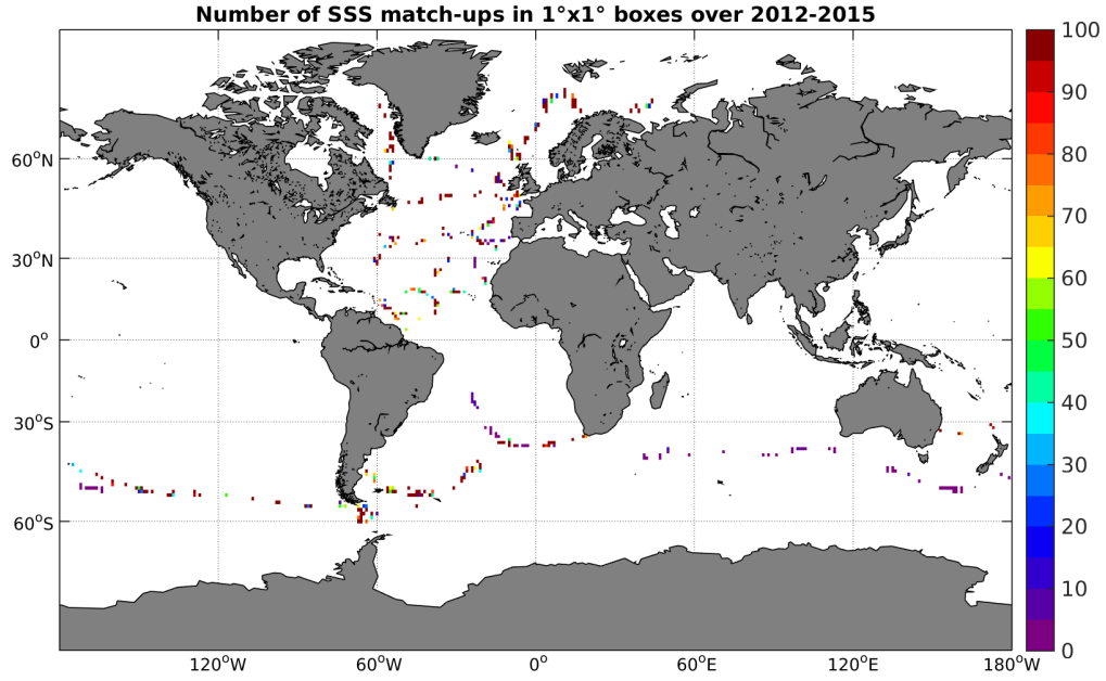
Figure 4: Number of SSS match-ups between TSG-GOSUD-Sailing-ship SSS and the AQUARIUS-L2-JPL-V4 SSS product for the Global Ocean Pi-MEP region over 1°x1° boxes and for the full satellite product period.
