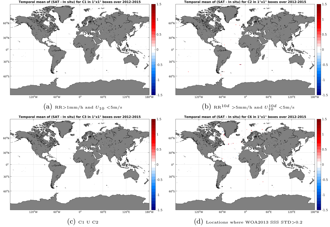
Figure 12: Temporal mean gridded over spatial boxes of size 1^\circ \times 1^\circ of \Delta SSS (AQUARIUS-L2-JPL-V4 - TSG-GOSUD-Sailing-ship) for 4 different subdatasets corresponding to: RR > 1\text{mm/h} and U_{10} < 5\text{m/s} (a), RR^{10d} > 5\text{mm/h} and U_{10}^{10d} < 5\text{m/s} (b), C1 U C2 (c), Locations where WOA2013 SSS STD > 0.2 (d).
