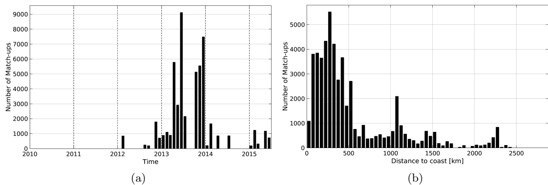
Figure 1: Number of match-ups between TSG-GOSUD-Sailing-ship and AQUARIUS-L2-JPL-V4 SSS as a function of time (a) and as function of the distance to coast (b) over the Global Ocean Pi-MEP region and for the full satellite product period.
