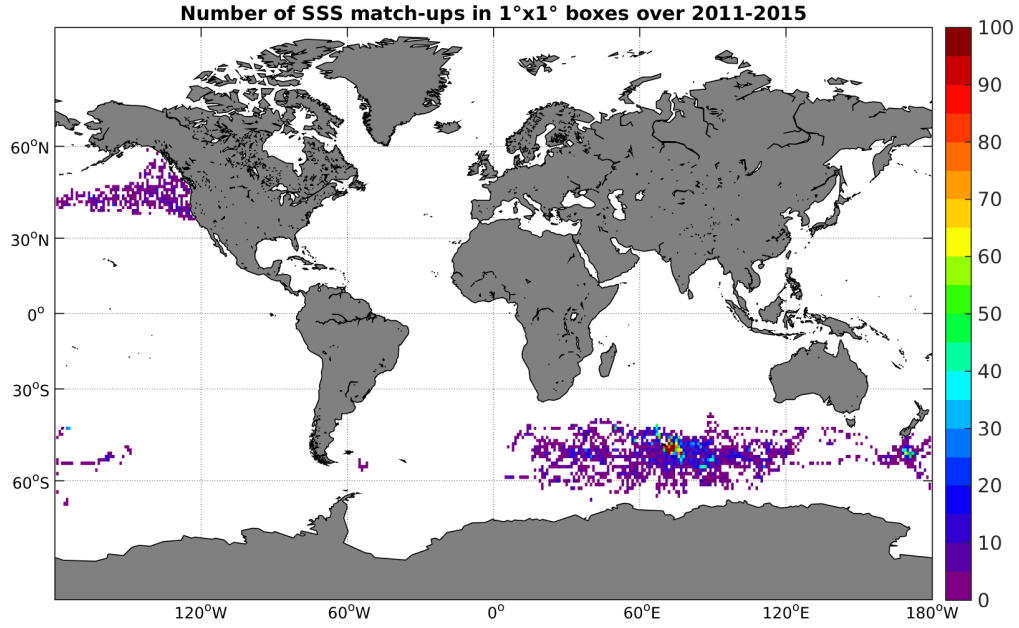
Figure 4: Number of SSS match-ups between Sea mammals SSS and the AQUARIUS-L2-JPL-V4 SSS product for the Global Ocean Pi-MEP region over 1°x1° boxes and for the full satellite product period.
