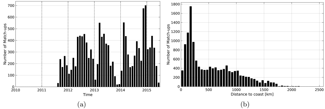
Figure 1: Number of match-ups between Sea mammals and AQUARIUS-L2-JPL-V4 SSS as a function of time (a) and as function of the distance to coast (b) over the Global Ocean Pi-MEP region and for the full satellite product period.
