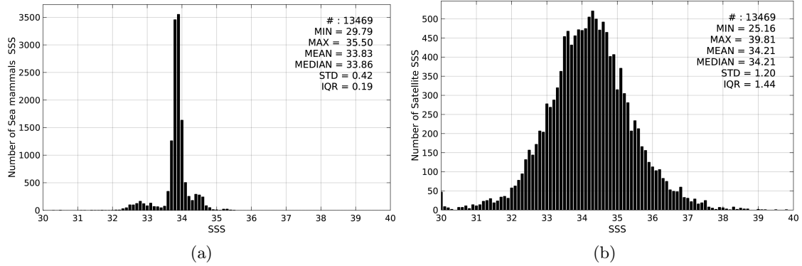
Figure 2: Histograms of SSS from Sea mammals (a) and AQUARIUS-L2-JPL-V4 (b) considering all match-up pairs per bins of 0.1 over the Global Ocean Pi-MEP region and for the full satellite product period.
