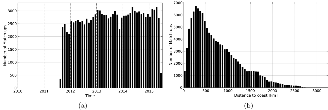
Figure 1: Number of match-ups between Argo and AQUARIUS-L2-JPL-V4 SSS as a function of time (a) and as function of the distance to coast (b) over the Global Ocean Pi-MEP region and for the full satellite product period.
