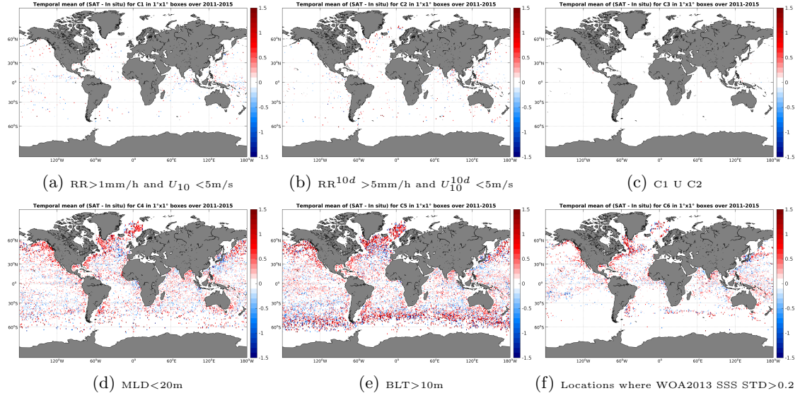
Figure 12: Temporal mean gridded over spatial boxes of size 1^\circ \times 1^\circ of \Delta\text{SSS} (AQUARIUS-L2-JPL-V4 - Argo) for 6 different subdatasets corresponding to: \text{RR} > 1\text{mm/h} and U_{10} < 5\text{m/s} (a), \text{RR}^{10d} > 5\text{mm/h} and U_{10}^{10d} < 5\text{m/s} (b), C1 U C2 (c), \text{MLD} < 20\text{m} (d), \text{BLT} > 10\text{m} (e), Locations where WOA2013 SSS STD > 0.2 (f).
