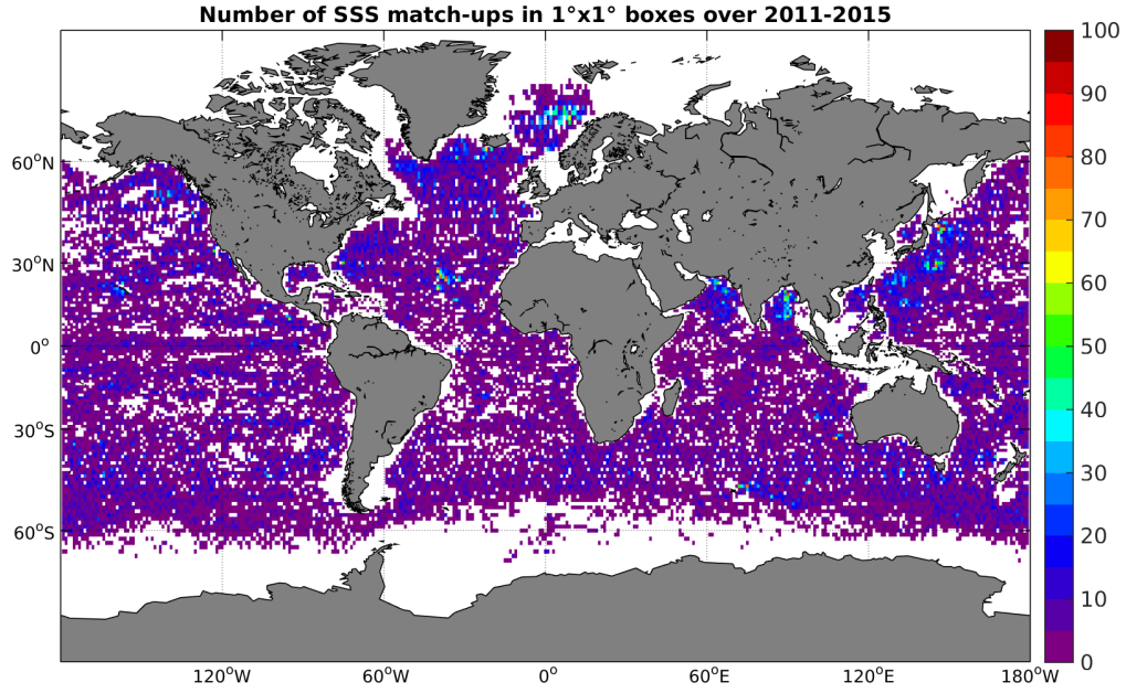
Figure 4: Number of SSS match-ups between Argo SSS and the AQUARIUS-L2-JPL-V4 SSS product for the Global Ocean Pi-MEP region over 1^\circ \times 1^\circ boxes and for the full satellite product period.
