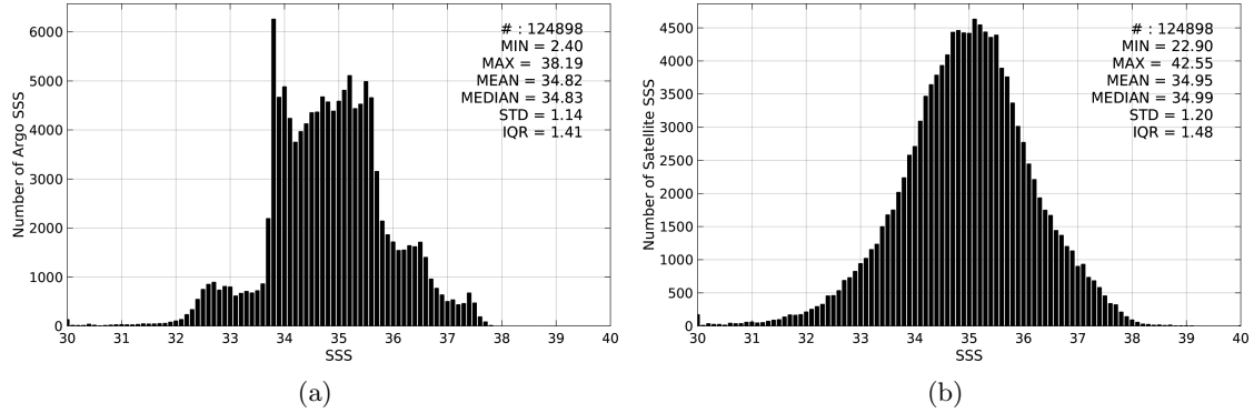
Figure 2: Histograms of SSS from Argo (a) and AQUARIUS-L2-JPL-V4 (b) considering all match-up pairs per bins of 0.1 over the Global Ocean Pi-MEP region and for the full satellite product period.
