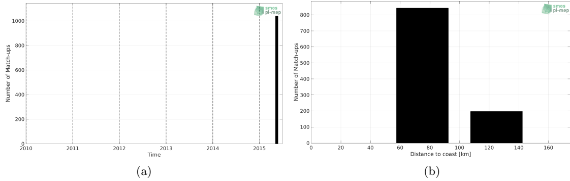
Figure 1: Number of match-ups between TSG (SAMOS) and SMOS and SMAP SSS L4 OI v1 - 7 Days (LOPS) SSS as a function of time (a) and as function of the distance to coast (b) over the Ganga and Brahmaputra river plumes Pi-MEP region and for the full satellite product period.
