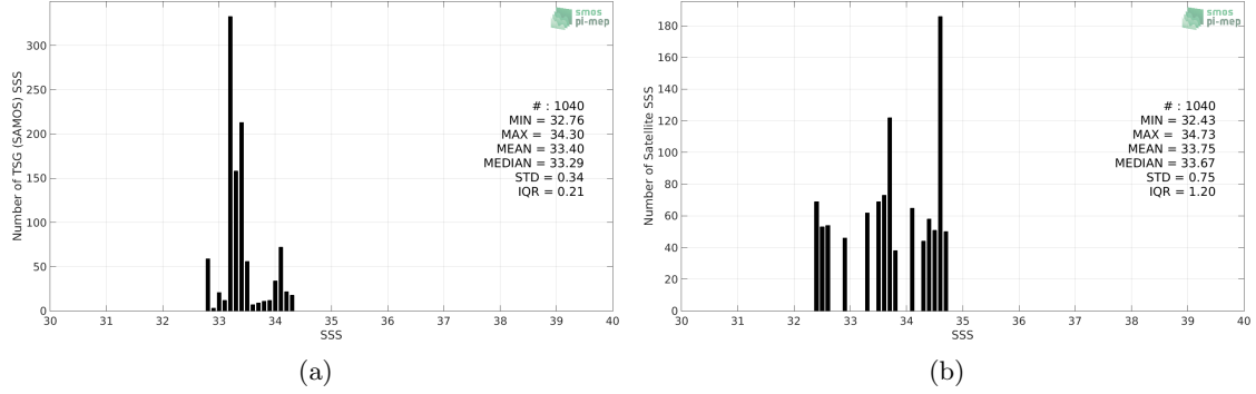
Figure 2: Histograms of SSS from TSG (SAMOS) (a) and SMOS and SMAP SSS L4 OI v1 - 7 Days (LOPS) (b) considering all match-up pairs per bins of 0.1 over the Ganga and Brahmaputra river plumes Pi-MEP region and for the full satellite product period.
