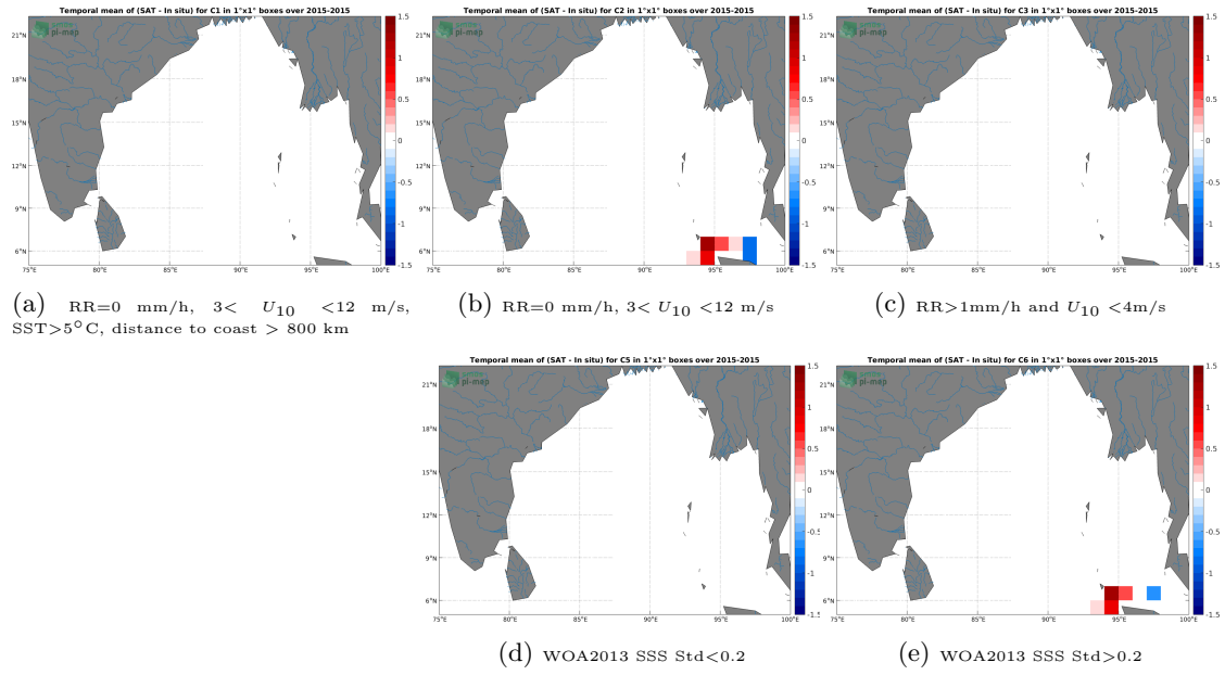
Figure 12: Temporal mean gridded over spatial boxes of size 1^\circ \times 1^\circ of \Delta SSS (SMOS and SMAP SSS L4 OI v1 - 7 Days (LOPS) - TSG (SAMOS)) for 5 different subdatasets corresponding to:RR=0 mm/h, 3 < U_{10} < 12 m/s, SST >5^\circ\text{C} , distance to coast > 800 km (a), RR=0 mm/h, 3 < U_{10} < 12 m/s (b), RR >1 mm/h and U_{10} < 4 m/s (c), WOA2013 SSS Std <0.2 (d), WOA2013 SSS Std >0.2 (e).
