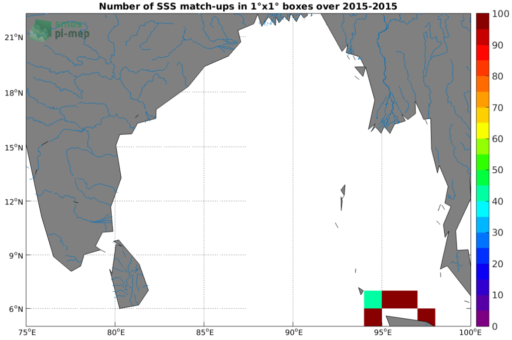
Figure 4: Number of SSS match-ups between TSG (SAMOS) SSS and the SMOS and SMAP SSS L4 OI v1 - 7 Days (LOPS) SSS product for the Ganga and Brahmaputra river plumes Pi-MEP region over 1^\circ \times 1^\circ boxes and for the full satellite product period.
