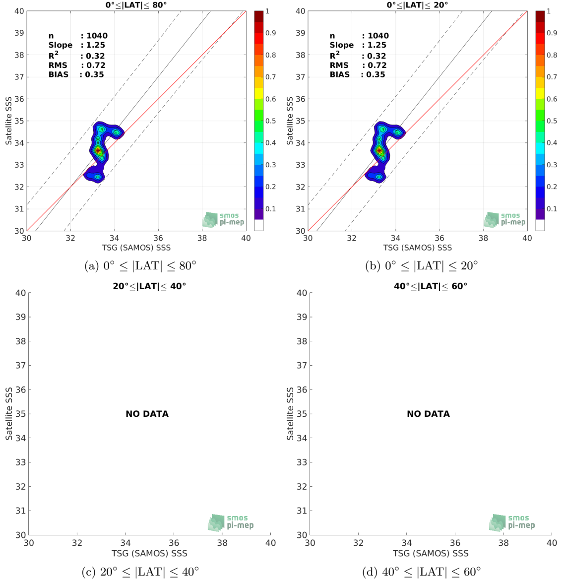
Figure 9: Contour maps of the concentration of SMOS and SMAP SSS L4 OI v1 - 7 Days (LOPS) SSS (y-axis) versus TSG (SAMOS) SSS (x-axis) at match-up pairs for different latitude bands. For each plot, the red line shows x=y . The black thin and dashed lines indicate a linear fit through the data cloud and the \pm 95\% confidence levels, respectively. The number match-up pairs n , the slope and R^2 coefficient of the linear fit, the root mean square (RMS) and the mean bias between satellite and in situ data are indicated for each latitude band in each plots.
