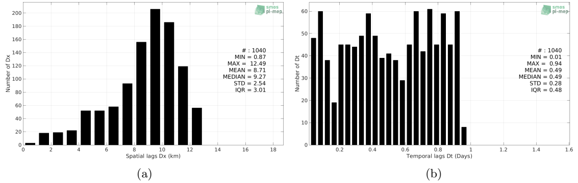
Figure 5: Histograms of the spatial (a) and temporal (b) lags between the location/time of the TSG (SAMOS) measurement and the date of the corresponding SMOS and SMAP SSS L4 OI v1 - 7 Days (LOPS) SSS pixel.
