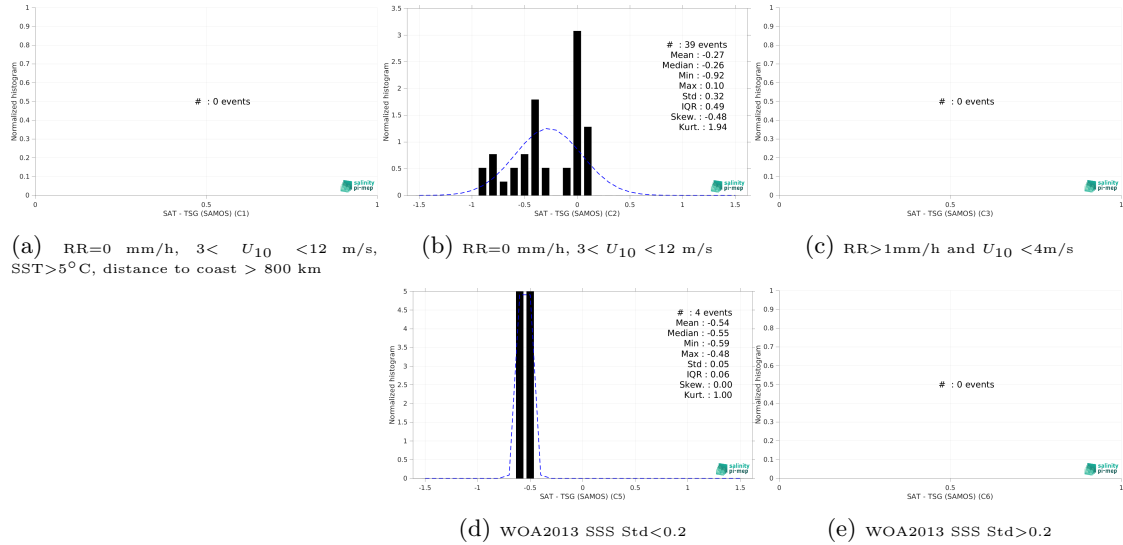
Figure 15: Normalized histogram of \Delta SSS (SMOS SSS L4 v1 - Monthly (CMEMS-CNR) - TSG (SAMOS)) for 5 different subdatasets corresponding to: RR=0 mm/h, 3 < U_{10} < 12 m/s, SST >5^{\circ} C, distance to coast > 800 km (a), RR=0 mm/h, 3 < U_{10} < 12 m/s (b), RR >1 mm/h and U_{10} < 4 m/s (c), WOA2013 SSS Std <0.2 (d), WOA2013 SSS Std >0.2 (e).
