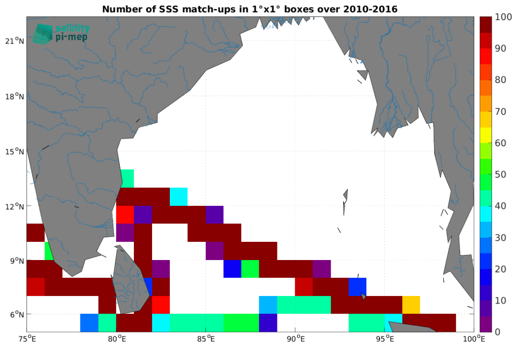
Figure 4: Number of SSS match-ups between TSG (LEGOS-DM) SSS and the SMOS SSS L4 v1 - Monthly (CMEMS-CNR) SSS product for the Ganga and Brahmaputra river plumes Pi-MEP region over 1^\circ \times 1^\circ boxes and for the full satellite product period.
