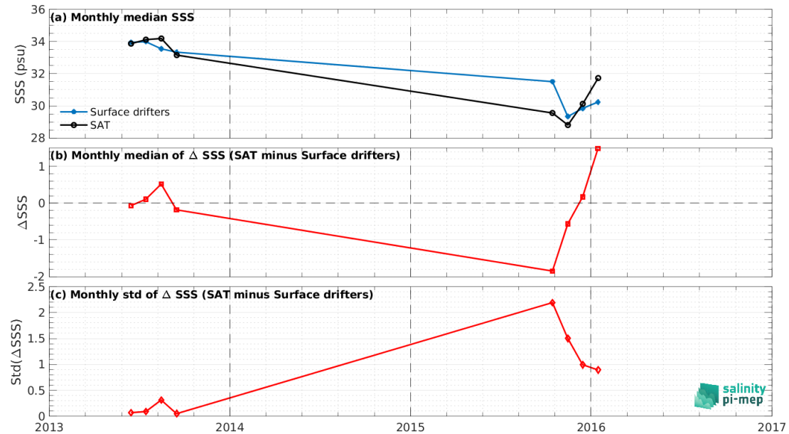
Figure 7: Time series of the monthly median SSS (top), median of \Delta\text{SSS} (Satellite - Surface drifters) and Std of \Delta\text{SSS} (Satellite - Surface drifters) over the Ganga and Brahmaputra river plumes Pi-MEP region considering all match-ups collected by the Pi-MEP.
