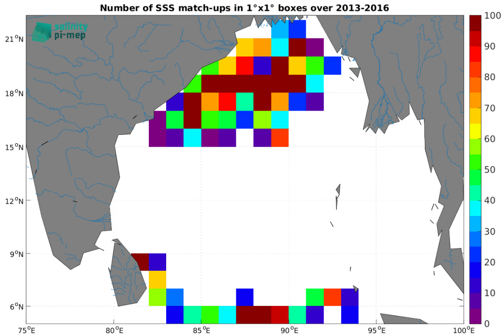
Figure 4: Number of SSS match-ups between Surface drifters SSS and the SMOS SSS L4 v1 - Monthly (CMEMS-CNR) SSS product for the Ganga and Brahmaputra river plumes Pi-MEP region over 1^\circ \times 1^\circ boxes and for the full satellite product period.
