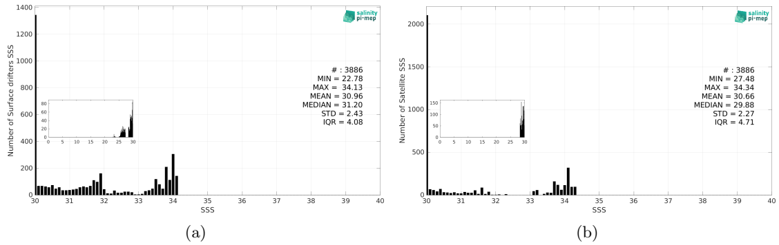
Figure 3: Histograms of SSS from Surface drifters (a) and SMOS SSS L4 v1 - Monthly (CMEMS-CNR) (b) considering all match-up pairs per bins of 0.1 over the Ganga and Brahmaputra river plumes Pi-MEP region and for the full satellite product period.
