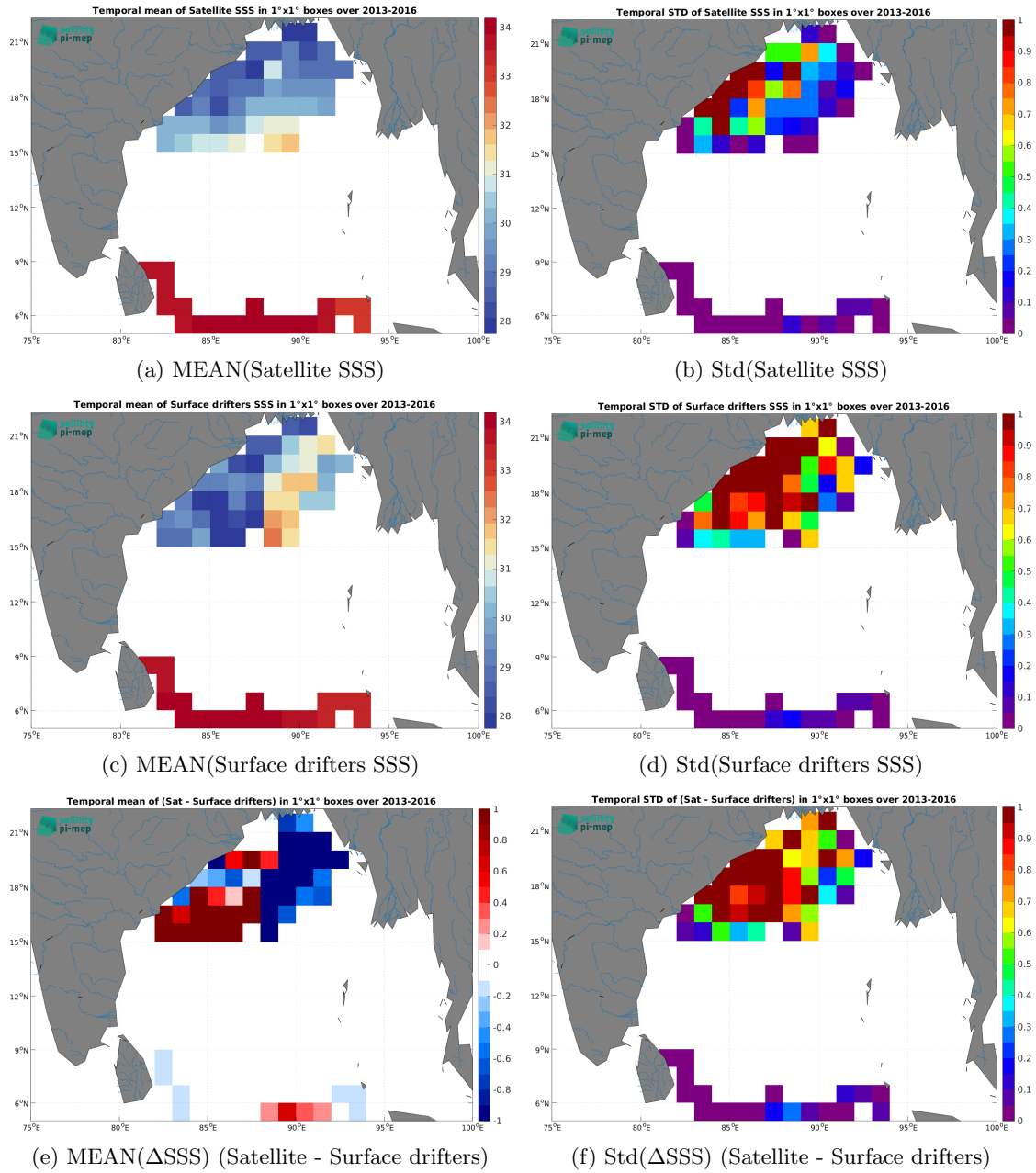
Figure 6: Temporal mean (left) and Std (right) of SSS from SMOS SSS L4 v1 - Monthly (CMEMS-CNR) (top), Surface drifters (middle), and of \Delta SSS (Satellite - Surface drifters). Only match-up pairs are used to generate these maps.
