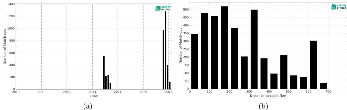
Figure 2: Number of match-ups between Surface drifters and SMOS SSS L4 v1 - Monthly (CMEMS-CNR) SSS as a function of time (a) and as function of the distance to coast (b) over the Ganga and Brahmaputra river plumes Pi-MEP region and for the full satellite product period.
