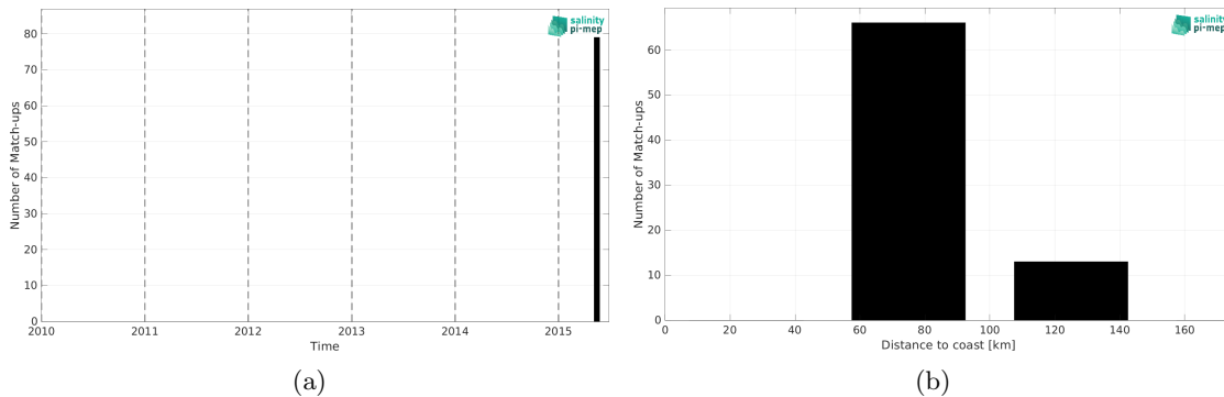
Figure 2: Number of match-ups between TSG (SAMOS) and SMOS SSS L4 v1 - Daily (CMEMS-CNR) SSS as a function of time (a) and as function of the distance to coast (b) over the Ganga and Brahmaputra river plumes Pi-MEP region and for the full satellite product period.
