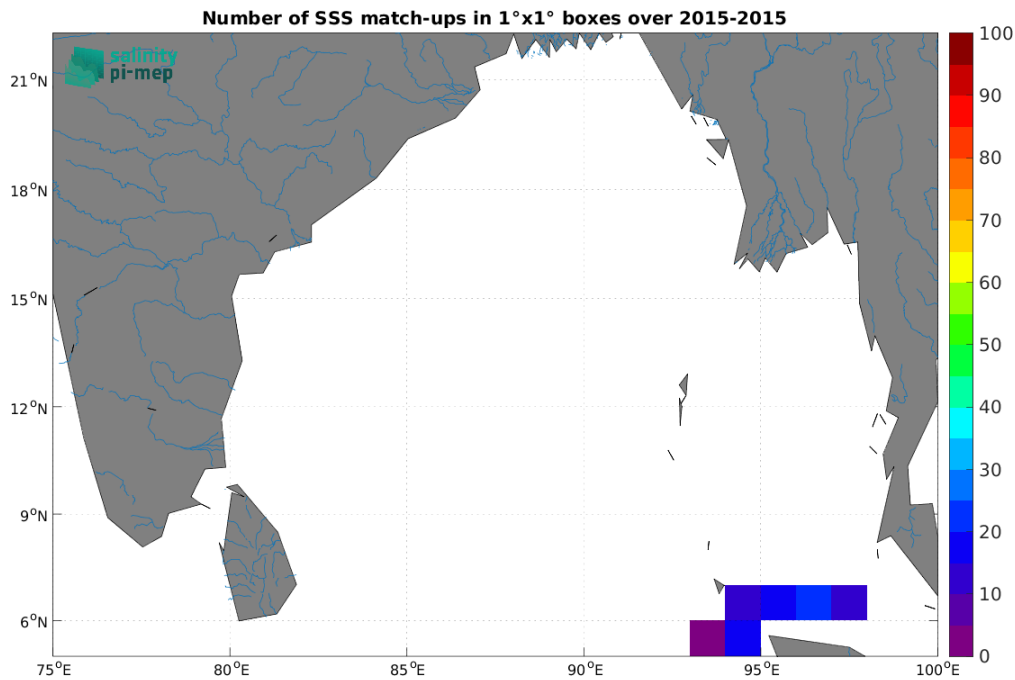
Figure 5: Number of SSS match-ups between TSG (SAMOS) SSS and the SMOS SSS L4 v1 - Daily (CMEMS-CNR) SSS product for the Ganga and Brahmaputra river plumes Pi-MEP region over 1^\circ \times 1^\circ boxes and for the full satellite product period.
