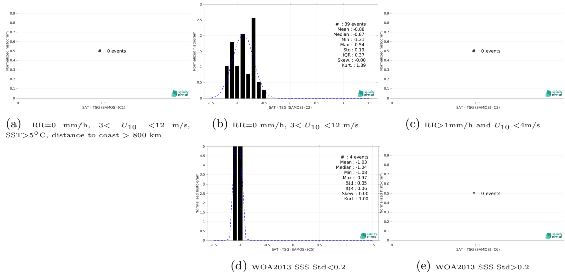
Figure 15: Normalized histogram of \Delta SSS (SMOS SSS L4 v1 - Daily (CMEMS-CNR) - TSG (SAMOS)) for 5 different subdatasets corresponding to: RR=0 mm/h, 3 < U_{10} < 12 m/s, SST >5^{\circ} C, distance to coast > 800 km (a), RR=0 mm/h, 3 < U_{10} < 12 m/s (b), RR >1 mm/h and U_{10} < 4 m/s (c), WOA2013 SSS Std <0.2 (d), WOA2013 SSS Std >0.2 (e).
