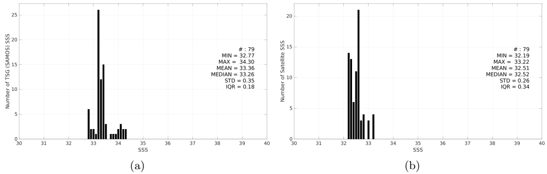
Figure 3: Histograms of SSS from TSG (SAMOS) (a) and SMOS SSS L4 v1 - Daily (CMEMS-CNR) (b) considering all match-up pairs per bins of 0.1 over the Ganga and Brahmaputra river plumes Pi-MEP region and for the full satellite product period.
