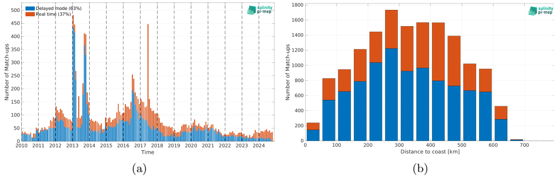
Figure 2: Number of match-ups between Argo and SMOS SSS L4 v1 - Daily (CMEMS-CNR) SSS as a function of time (a) and as function of the distance to coast (b) over the Ganga and Brahmaputra river plumes Pi-MEP region and for the full satellite product period.
