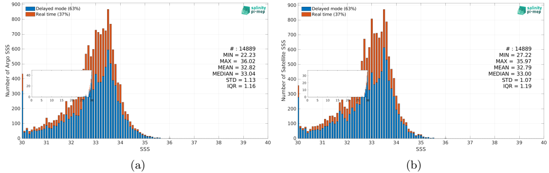
Figure 3: Histograms of SSS from Argo (a) and SMOS SSS L4 v1 - Daily (CMEMS-CNR) (b) considering all match-up pairs per bins of 0.1 over the Ganga and Brahmaputra river plumes Pi-MEP region and for the full satellite product period.
