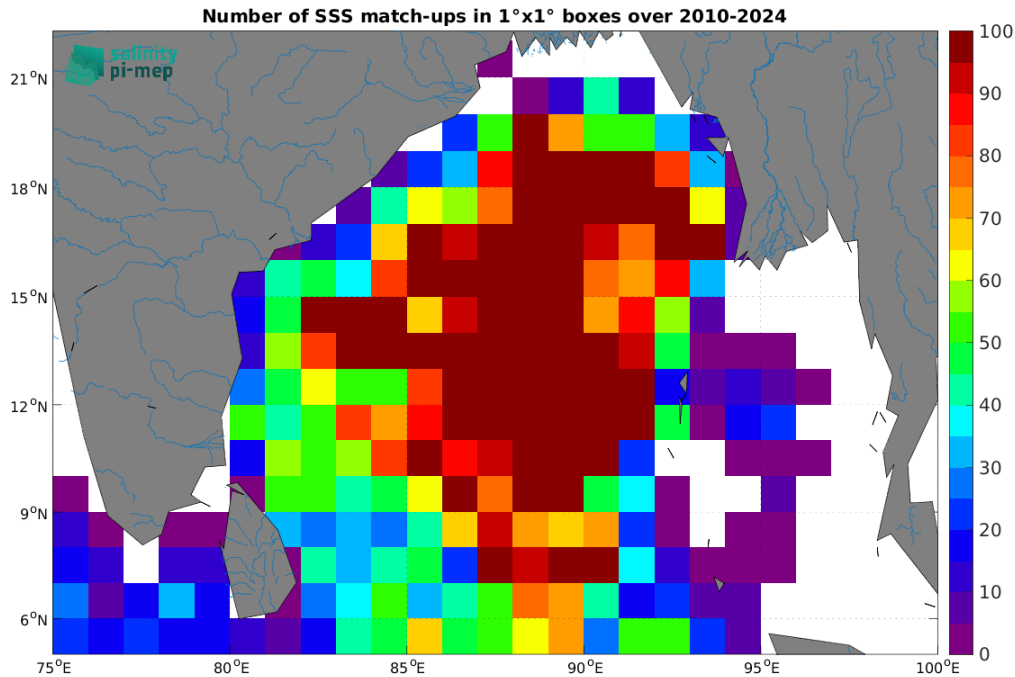
Figure 5: Number of SSS match-ups between Argo SSS and the SMOS SSS L4 v1 - Daily (CMEMS-CNR) SSS product for the Ganga and Brahmaputra river plumes Pi-MEP region over 1^\circ \times 1^\circ boxes and for the full satellite product period.
