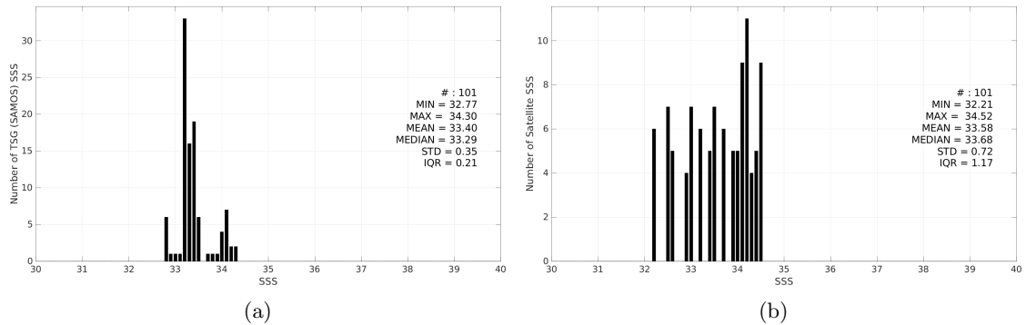
Figure 3: Histograms of SSS from TSG (SAMOS) (a) and SMOS SSS L4 OI v346 - Weekly (CMEMS-CATDS-LOPS) (b) considering all match-up pairs per bins of 0.1 over the Ganga and Brahmaputra river plumes Pi-MEP region and for the full satellite product period.
