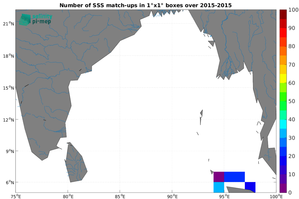
Figure 5: Number of SSS match-ups between TSG (SAMOS) SSS and the SMOS SSS L4 OI v346 - Weekly (CMEMS-CATDS-LOPS) SSS product for the Ganga and Brahmaputra river plumes Pi-MEP region over 1^\circ \times 1^\circ boxes and for the full satellite product period.
