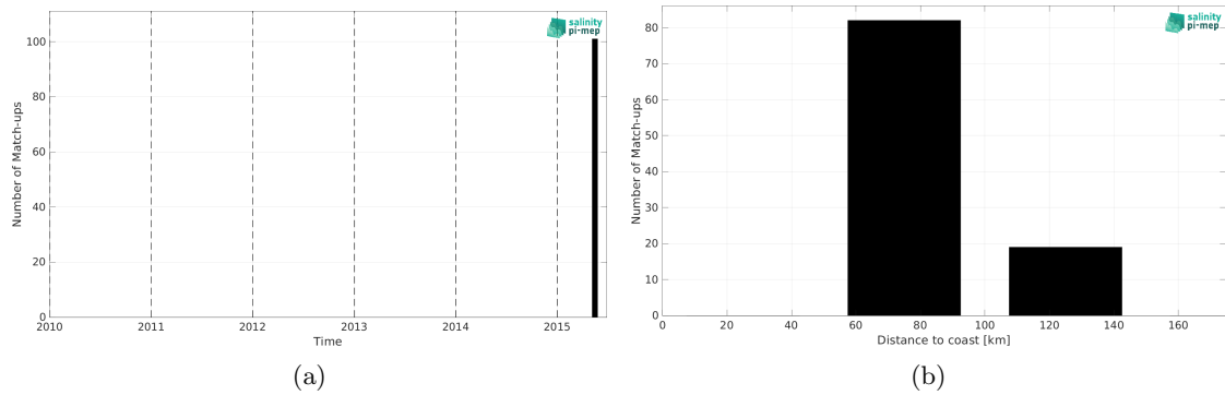
Figure 2: Number of match-ups between TSG (SAMOS) and SMOS SSS L4 OI v346 - Weekly (CMEMS-CATDS-LOPS) SSS as a function of time (a) and as function of the distance to coast (b) over the Ganga and Brahmaputra river plumes Pi-MEP region and for the full satellite product period.
