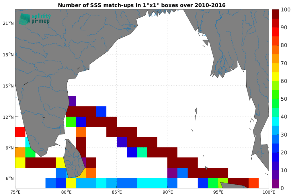
Figure 5: Number of SSS match-ups between TSG (LEGOS-DM) SSS and the SMOS SSS L4 OI v346 - Weekly (CMEMS-CATDS-LOPS) SSS product for the Ganga and Brahmaputra river plumes Pi-MEP region over 1^{\circ} \times 1^{\circ} boxes and for the full satellite product period.
