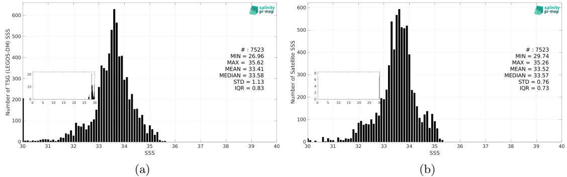
Figure 3: Histograms of SSS from TSG (LEGOS-DM) (a) and SMOS SSS L4 OI v346 - Weekly (CMEMS-CATDS-LOPS) (b) considering all match-up pairs per bins of 0.1 over the Ganga and Brahmaputra river plumes Pi-MEP region and for the full satellite product period.
