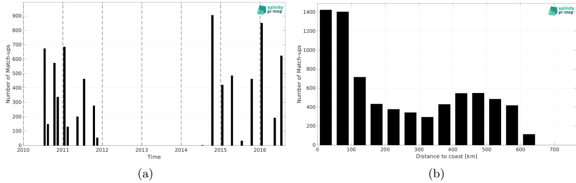
Figure 2: Number of match-ups between TSG (LEGOS-DM) and SMOS SSS L4 OI v346 - Weekly (CMEMS-CATDS-LOPS) SSS as a function of time (a) and as function of the distance to coast (b) over the Ganga and Brahmaputra river plumes Pi-MEP region and for the full satellite product period.
