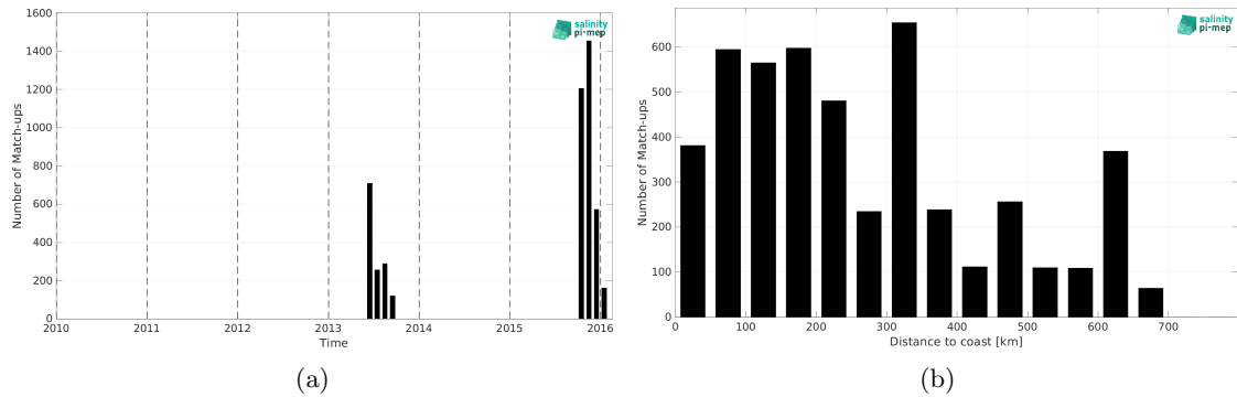
Figure 2: Number of match-ups between Surface drifters and SMOS SSS L4 OI v346 - Weekly (CMEMS-CATDS-LOPS) SSS as a function of time (a) and as function of the distance to coast (b) over the Ganga and Brahmaputra river plumes Pi-MEP region and for the full satellite product period.
