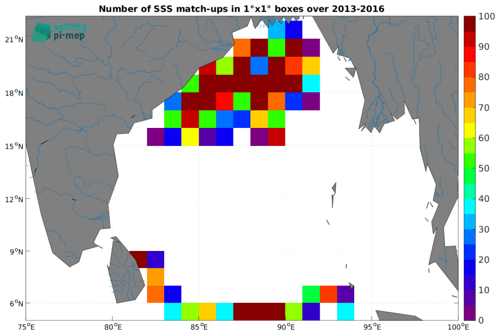
Figure 4: Number of SSS match-ups between Surface drifters SSS and the SMOS SSS L4 OI v346 - Weekly (CMEMS-CATDS-LOPS) SSS product for the Ganga and Brahmaputra river plumes Pi-MEP region over 1^{\circ} \times 1^{\circ} boxes and for the full satellite product period.
