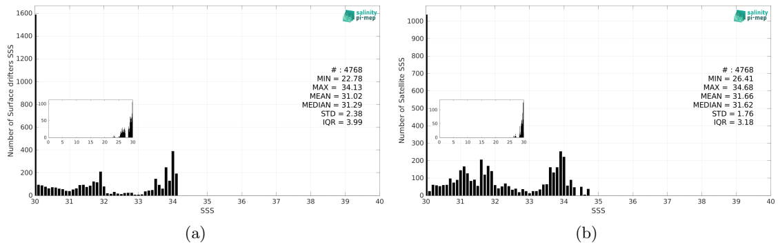
Figure 3: Histograms of SSS from Surface drifters (a) and SMOS SSS L4 OI v346 - Weekly (CMEMS-CATDS-LOPS) (b) considering all match-up pairs per bins of 0.1 over the Ganga and Brahmaputra river plumes Pi-MEP region and for the full satellite product period.
