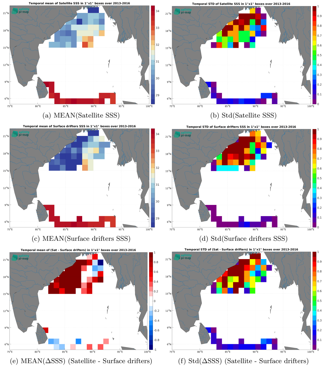
Figure 6: Temporal mean (left) and Std (right) of SSS from SMOS SSS L4 OI v346 - Weekly (CMEMS-CATDS-LOPS) (top), Surface drifters (middle), and of \Delta SSS (Satellite - Surface drifters). Only match-up pairs are used to generate these maps.
