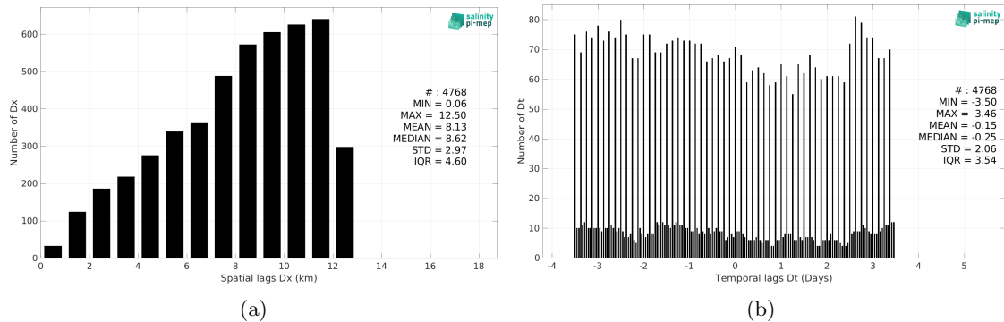
Figure 5: Histograms of the spatial (a) and temporal (b) lags between the location/time of the Surface drifters measurement and the date of the corresponding SMOS SSS L4 OI v346 - Weekly (CMEMS-CATDS-LOPS) SSS pixel.
