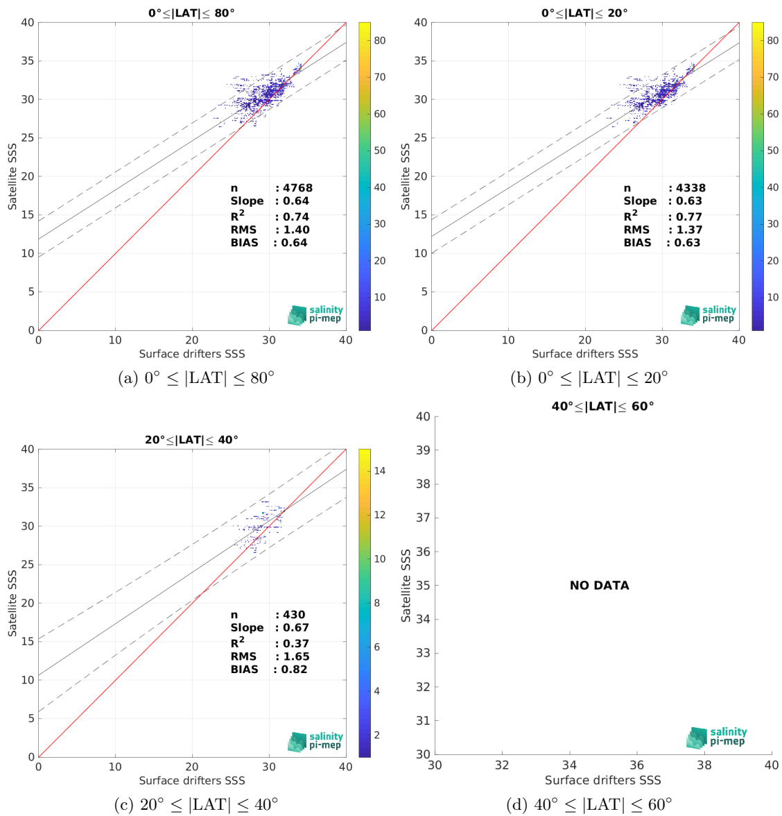
Figure 9: Contour maps of the concentration of SMOS SSS L4 OI v346 - Weekly (CMEMS-CATDS-LOPS) SSS (y-axis) versus Surface drifters SSS (x-axis) at match-up pairs for different latitude bands. For each plot, the red line shows x=y . The black thin and dashed lines indicate a linear fit through the data cloud and the \pm 95\% confidence levels, respectively. The number match-up pairs n , the slope and R^2 coefficient of the linear fit, the root mean square (RMS) and the mean bias between satellite and in situ data are indicated for each latitude band in each plots.
