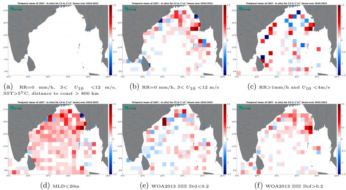
Figure 14: Temporal mean gridded over spatial boxes of size 1^\circ \times 1^\circ of \Delta SSS (SMOS SSS L4 OI v346 - Weekly (CMEMS-CATDS-LOPS) - Argo) for 6 different subdatasets corresponding to:RR=0 mm/h, 3 < U_{10} < 12 m/s, SST >5^\circ C, distance to coast > 800 km (a), RR=0 mm/h, 3 < U_{10} < 12 m/s (b), RR >1 mm/h and U_{10} < 4 m/s (c),MLD <20 m (d),WOA2013 SSS Std <0.2 (e),WOA2013 SSS Std >0.2 (f).
