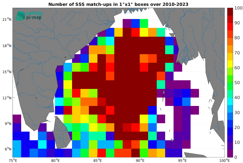
Figure 5: Number of SSS match-ups between Argo SSS and the SMOS SSS L4 OI v346 - Weekly (CMEMS-CATDS-LOPS) SSS product for the Ganga and Brahmaputra river plumes Pi-MEP region over 1^\circ \times 1^\circ boxes and for the full satellite product period.
