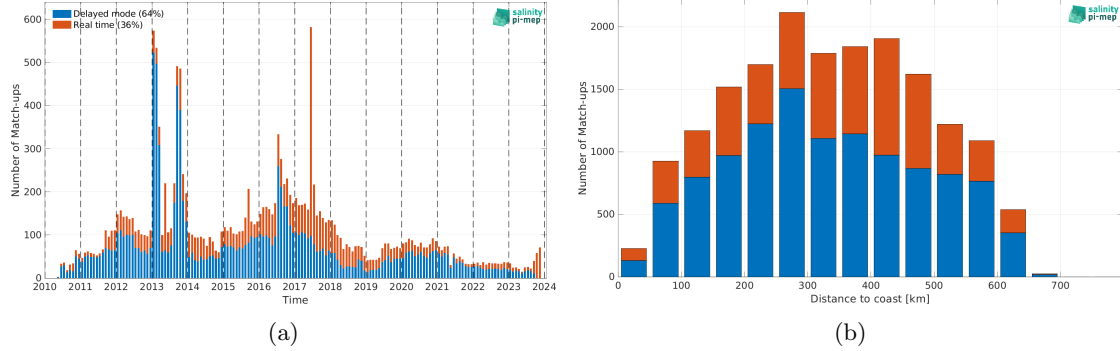
Figure 2: Number of match-ups between Argo and SMOS SSS L4 OI v346 - Weekly (CMEMS-CATDS-LOPS) SSS as a function of time (a) and as function of the distance to coast (b) over the Ganga and Brahmaputra river plumes Pi-MEP region and for the full satellite product period.
