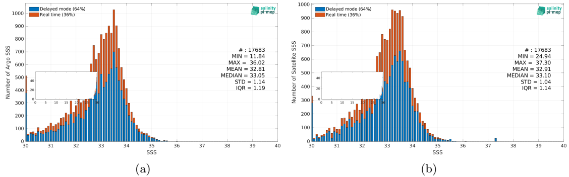
Figure 3: Histograms of SSS from Argo (a) and SMOS SSS L4 OI v346 - Weekly (CMEMS-CATDS-LOPS) (b) considering all match-up pairs per bins of 0.1 over the Ganga and Brahmaputra river plumes Pi-MEP region and for the full satellite product period.
