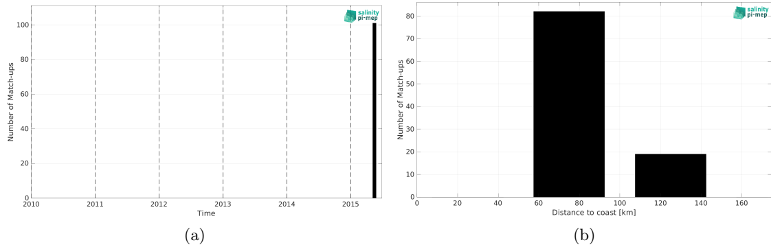
Figure 1: Number of match-ups between TSG (SAMOS) and SMOS SSS L4 OI v342 - Weekly (CMEMS-CATDS-LOPS) SSS as a function of time (a) and as function of the distance to coast (b) over the Ganga and Brahmaputra river plumes Pi-MEP region and for the full satellite product period.
