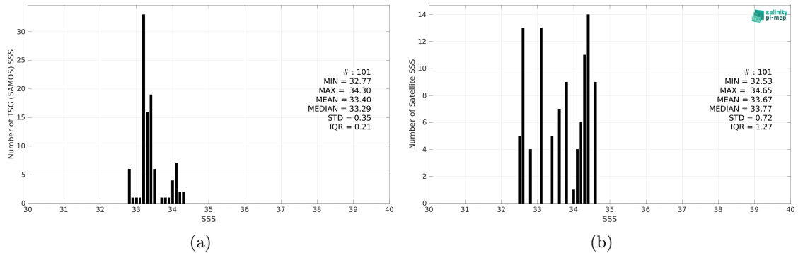
Figure 2: Histograms of SSS from TSG (SAMOS) (a) and SMOS SSS L4 OI v342 - Weekly (CMEMS-CATDS-LOPS) (b) considering all match-up pairs per bins of 0.1 over the Ganga and Brahmaputra river plumes Pi-MEP region and for the full satellite product period.
