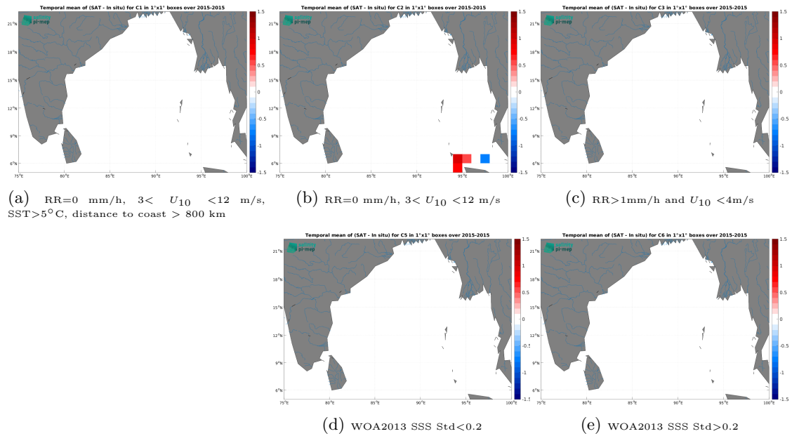
Figure 12: Temporal mean gridded over spatial boxes of size 1^{\circ}\times 1^{\circ} of \Delta\text{SSS} (SMOS SSS L4 OI v342 - Weekly (CMEMS-CATDS-LOPS) - TSG (SAMOS)) for 5 different subdatasets corresponding to:RR=0 mm/h, 3 < U_{10} < 12 m/s, SST > 5^{\circ}\text{C} , distance to coast > 800 km (a), RR=0 mm/h, 3 < U_{10} < 12 m/s (b), RR > 1 mm/h and U_{10} < 4 m/s (c), WOA2013 SSS Std < 0.2 (d), WOA2013 SSS Std > 0.2 (e).
