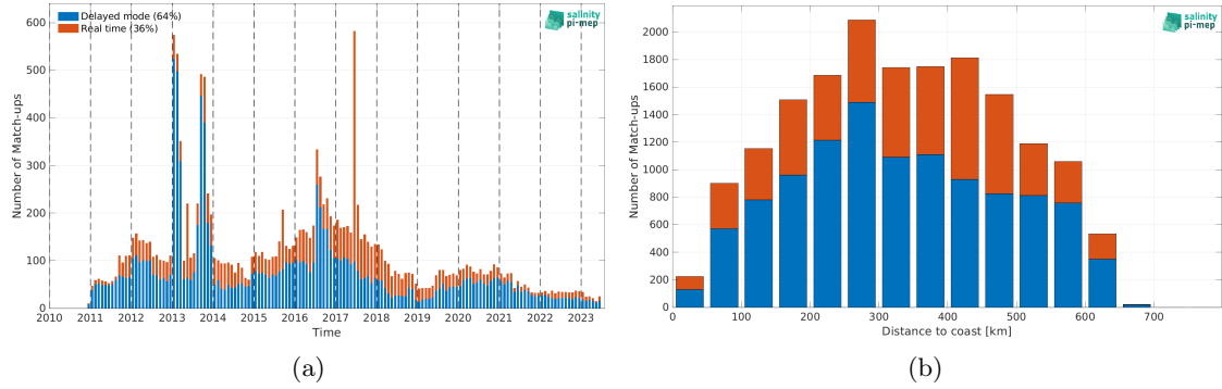
Figure 1: Number of match-ups between Argo and SMOS SSS L4 OI v342 - Weekly (CMEMS-CATDS-LOPS) SSS as a function of time (a) and as function of the distance to coast (b) over the Ganga and Brahmaputra river plumes Pi-MEP region and for the full satellite product period.
