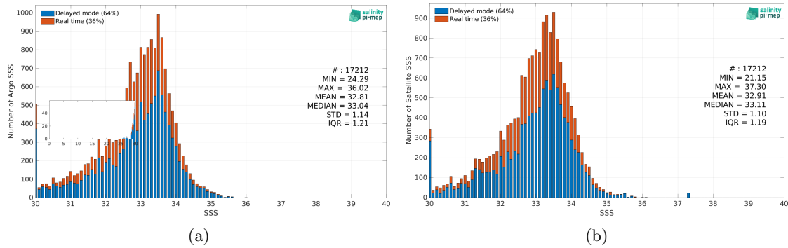
Figure 2: Histograms of SSS from Argo (a) and SMOS SSS L4 OI v342 - Weekly (CMEMS-CATDS-LOPS) (b) considering all match-up pairs per bins of 0.1 over the Ganga and Brahmaputra river plumes Pi-MEP region and for the full satellite product period.
