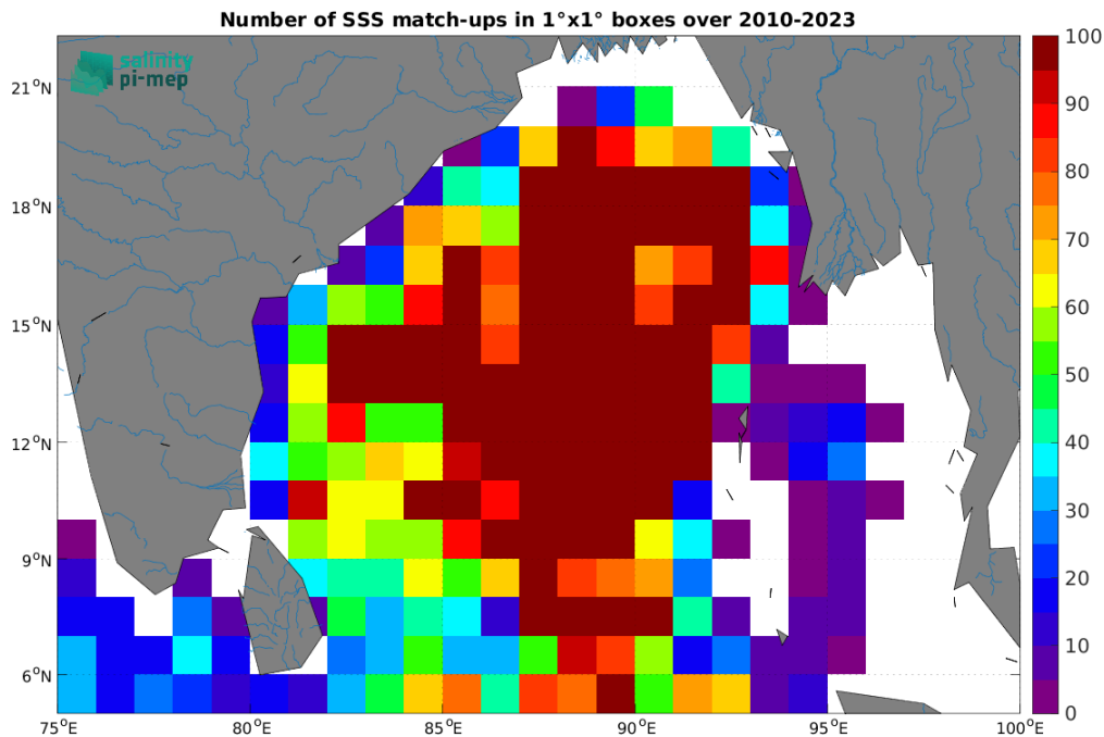
Figure 4: Number of SSS match-ups between Argo SSS and the SMOS SSS L4 OI v342 - Weekly (CMEMS-CATDS-LOPS) SSS product for the Ganga and Brahmaputra river plumes Pi-MEP region over 1^\circ \times 1^\circ boxes and for the full satellite product period.
